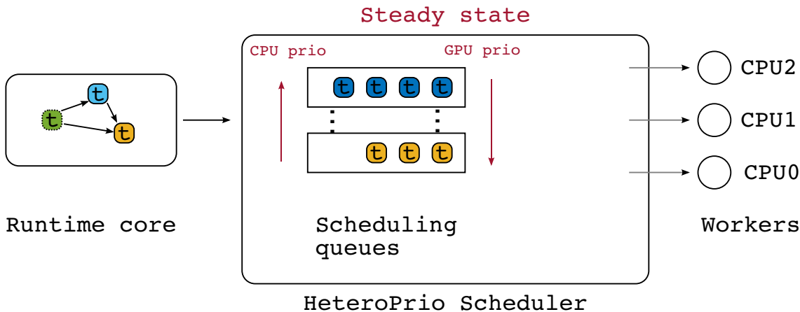
Figure 6.6: HeteroPrio steady-state policy.
