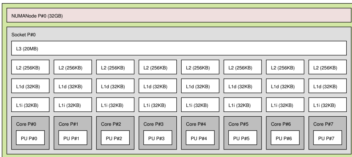
Figure 1.24: The architecture of one of the four sockets on the Ada computer.
