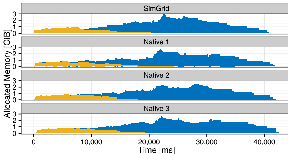
Figure 7.7: Native and simulated memory consumption for matrix #6 on the Fourmi system.
