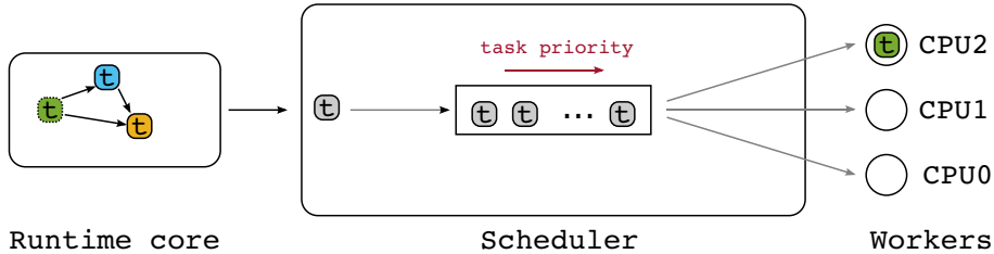
Figure 3.4: Sorted central queue scheduler in qrm_starpu .
