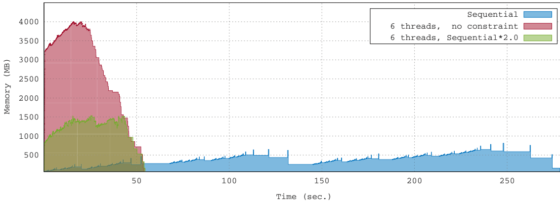
Figure 5.1: The memory profiles for matrix #12 for a sequential (in blue) and 6-threaded parallel factorization without memory constraint (in red) and with a constraint equal to 2.0 times the sequential peak (in green).
