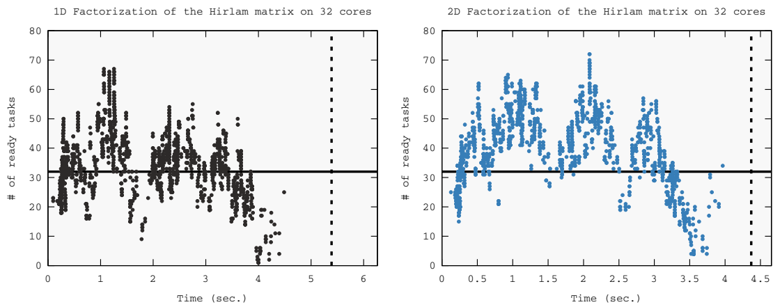
Figure 5.6: Concurrency under a memory constraint for the Hirlam matrix on Ada (32 cores).
