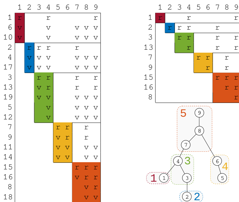
Figure 1.7: Example of multifrontal QR factorization. On the left side the factorized matrix (the same as in Figure 1.6 with a row permutation). On the upper-right part, the structure of the resulting R factor. On the right-bottom part the elimination tree; the dashed boxes show how the nodes are amalgamated into supernodes.
