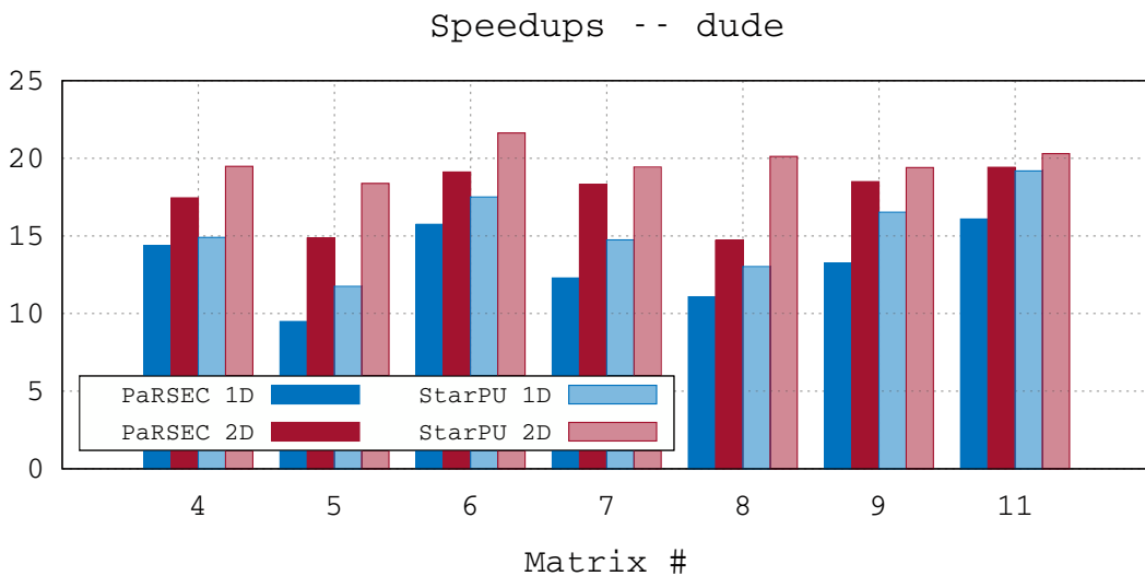
Figure 7.4: Speedup for the qr_starpus and qr_parsec on dude system (24 cores).
