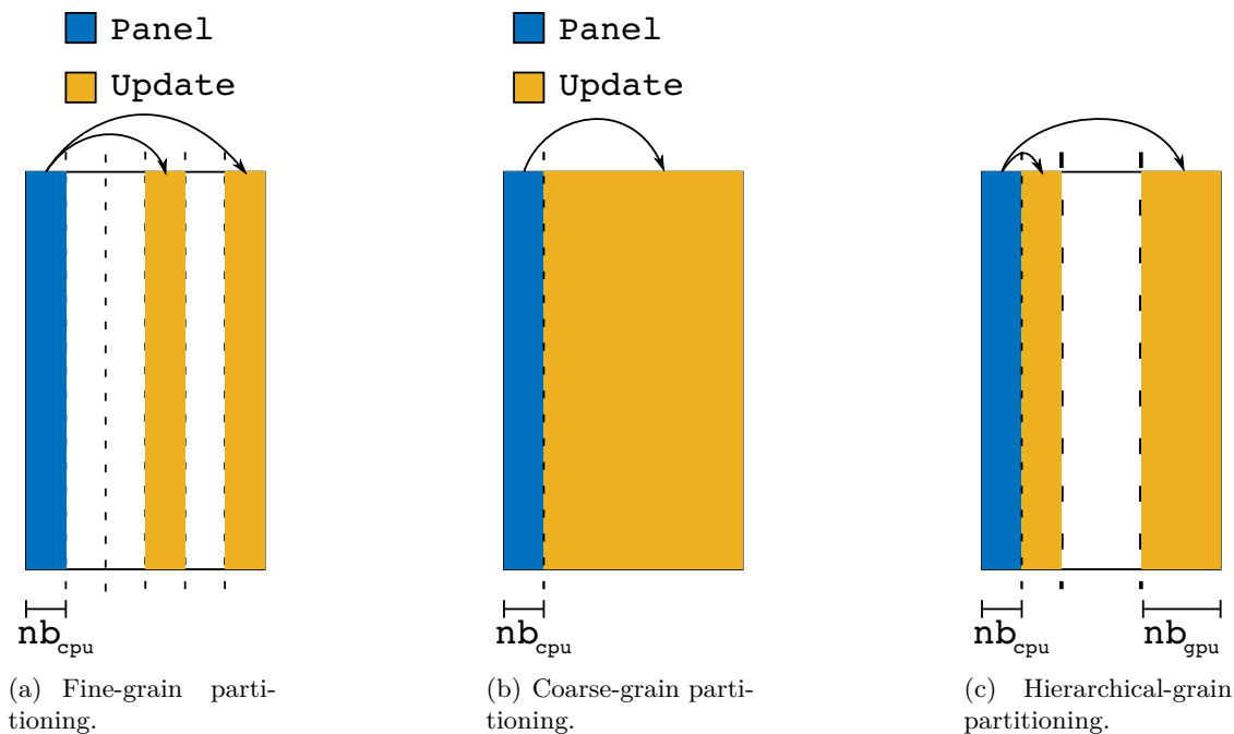
Figure 6.1: Partitioning schemes.
