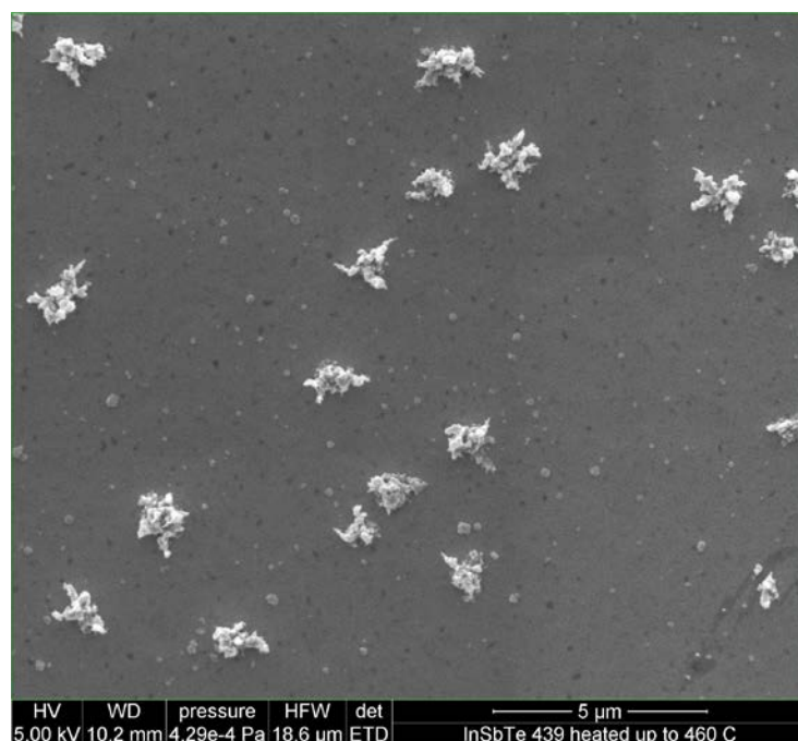
Figure 57: \text{In}_3\text{Sb}_{2.5}\text{Te}_{1.2} (sample 439) heated to 460^\circ\text{C} and return to the room temperature (RT) - Heterogeneous surface
