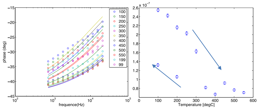
Figure 63: sample MOIST434 (90nm) left: phase calculated (line) with optimal value of R_t and measured (hollow disk); right: identified R_T' in K.m^2/W .
