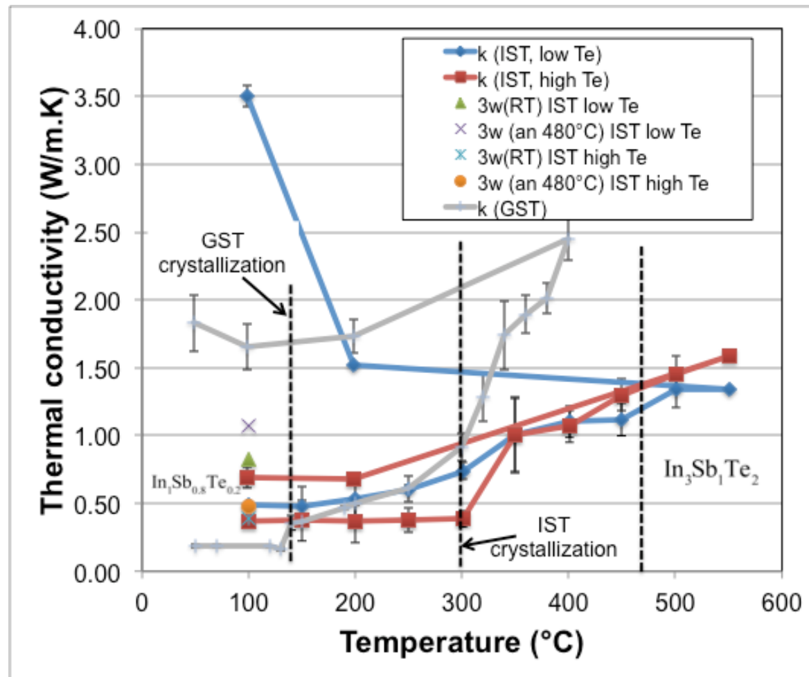
Figure 72: In-Sb-Te thermal conductivity k_{IST} for the two Te contents, comparison with GST(225). The data obtained on as-deposited IST using the 3 \omega method for both compositions are also reported.
