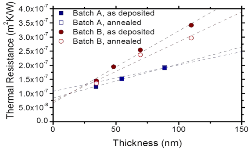
Figure 39: Thermal resistance (R_T - 2e_{\text{dielect}}/k_{\text{dielect}}) versus IST thickness. SiO 2 -capped composition A (squares) and B (circles) both before (full symbol) and after (hollow symbol) thermal annealing. [Symbols are consistent with those defined in Table 3]
