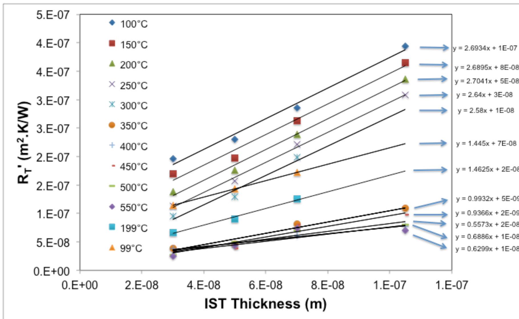
Figure 69 : Thermal resistance of high-Tc sample.
