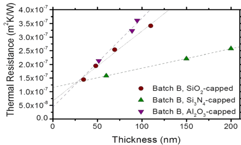
Figure 40: thermal resistance (R_T - 2e_{\text{dielect}}/k_{\text{dielect}}) versus IST thickness. Composition B, as deposited, capped between: SiO 2 (circles), Si 3 N 4 (upward triangles) and Al 2 O 3 (downward triangles). [Symbols are consistent with those defined in Table 3]
