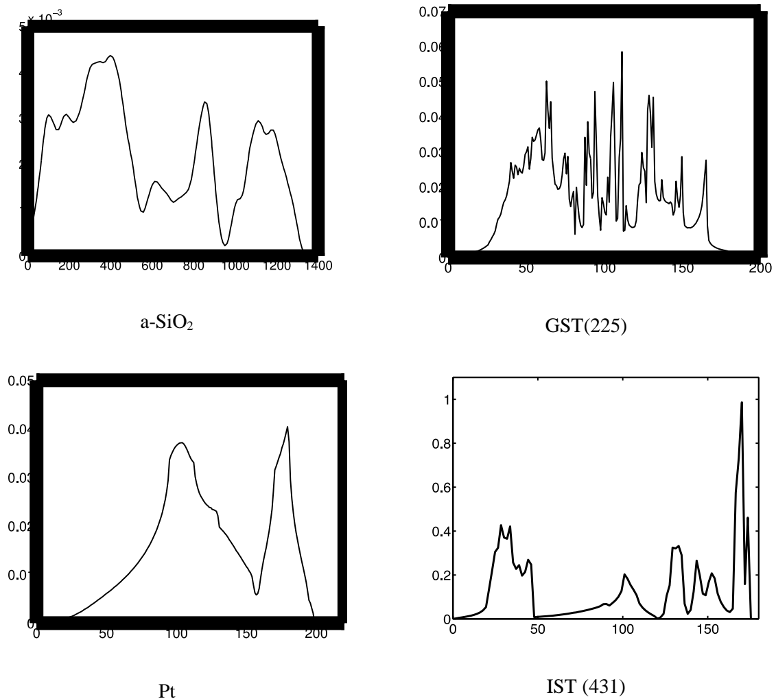
Figure 77: DOS for amorphous \text{SiO}_2 , GST(225), IST(431) and Pt calculated using DFT (calculations performed by Marco Bernasconi, UMB).
