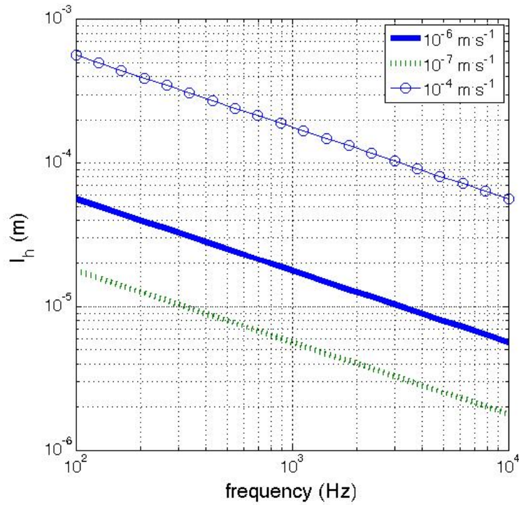
Figure 28: heat diffusion length for two values of the thermal diffusivity according to the experimental frequency range.
