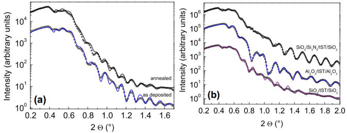
Figure 37: XRR data (symbols) and simulations (lines) of (a): as deposited and 480°C annealed 70 nm thick IST sandwiched between SiO 2 ; (b): as deposited IST, 48 nm thick, in contact with different bottom and top dielectric layers.
