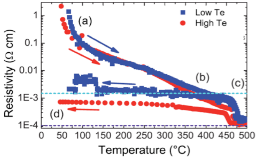
Figure 53: From Fallica et al. , 2013. In red \text{In}_3\text{Sb}_{2.5}\text{Te}_{1.2} (Cf figure 17). In blue \text{In}_3\text{Sb}_{2.7}\text{Te}_{0.8} . Electrical resistivity measured in-situ during heating experiment carried at 20^\circ\text{C}/\text{min} . Dashed cyan line: resistivity of \text{InSb}_{0.8}\text{Te}_{0.2} at room temperature. Dashed dark blue line: resistivity of \text{In}_3\text{SbTe}_2 at room temperature.
