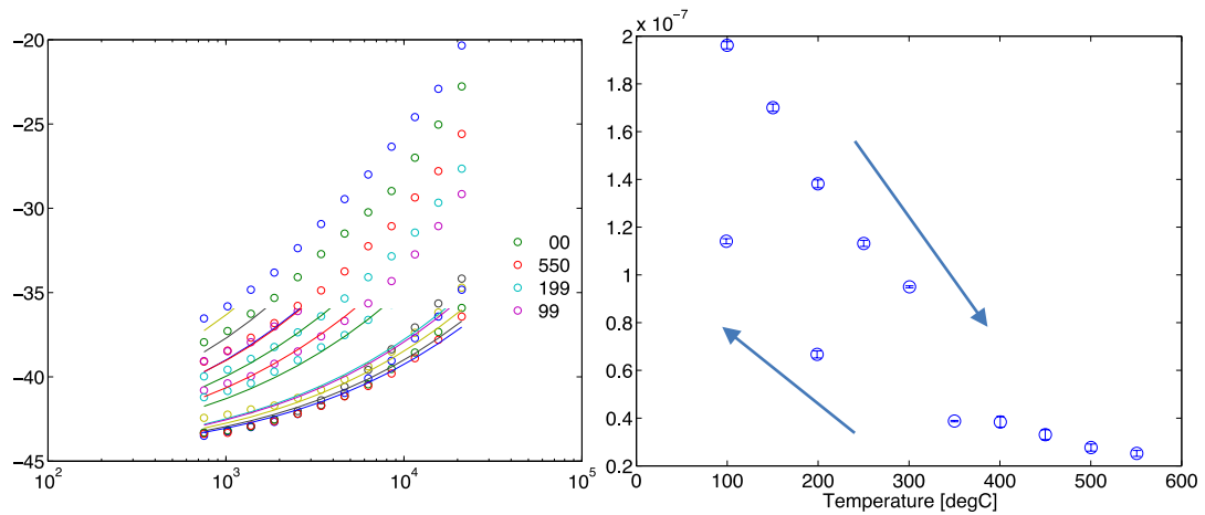
Figure 64: sample MOIST441 (30nm) left: phase calculated (line) with optimal value of R_t and measured (hollow disk); right: identified R_T' in \text{K.m}^2/\text{W} .
