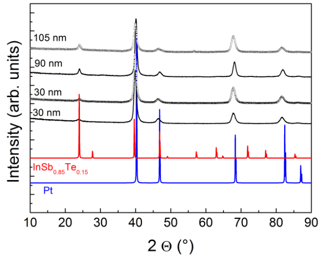
Figure 44: XRD measurements on as-deposited In-Sb-Te sample (MOIST439).
