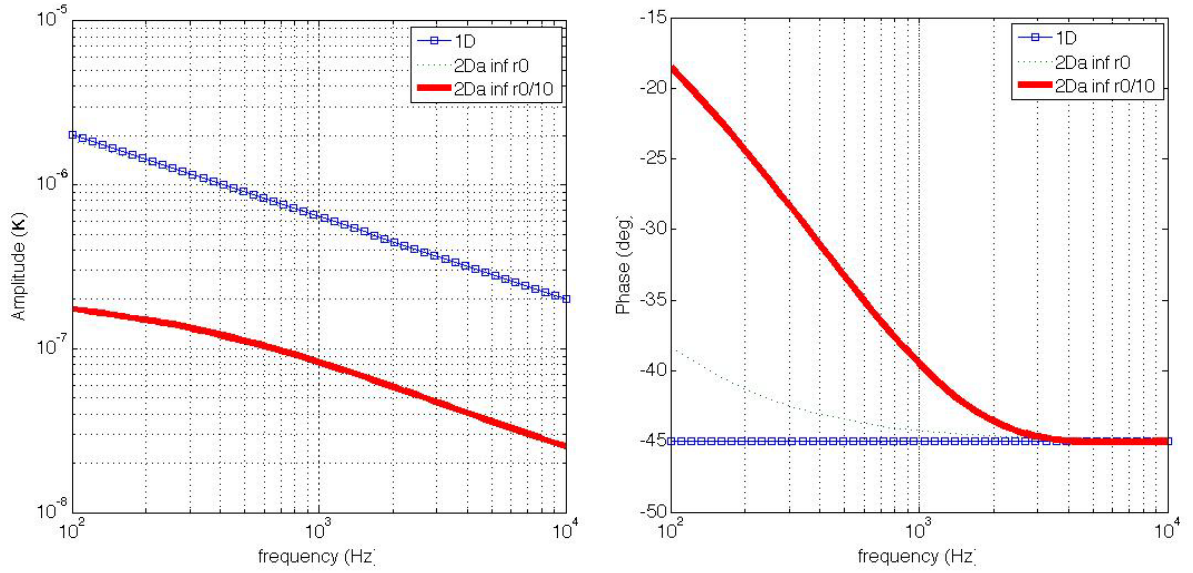
Figure 29: amplitude and phase calculated for the semi infinite substrate (with R_T=0 ) considering a 1D heat transfer model (relation (3.58)) and the 2D axi model (relation (3.54)). Values are r_0 = 2.5 \times 10^{-3} m; r_d = 0.5 \times 10^{-3} m; R = 2.5 \times 10^{-3} m; k=238 W.m -1 .K -1 , a = 1.45 \times 10^{-4} m 2 .s -1 (silicon).
