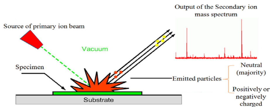
Figure 9: Description of ToF-SIMS principle
