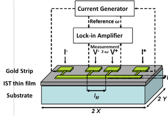
Figure 14: Layout of the 3 omega measurements
