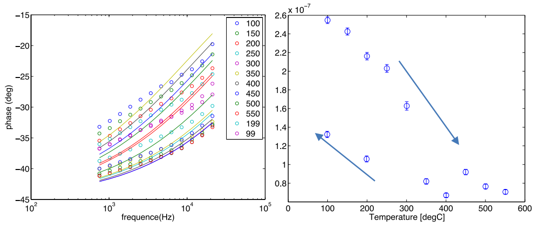
Figure 63: sample MOIST434 (90nm) left: phase calculated (line) with optimal value of R_t and measured (hollow disk); right: identified R_T' in \text{K.m}^2/\text{W} .
