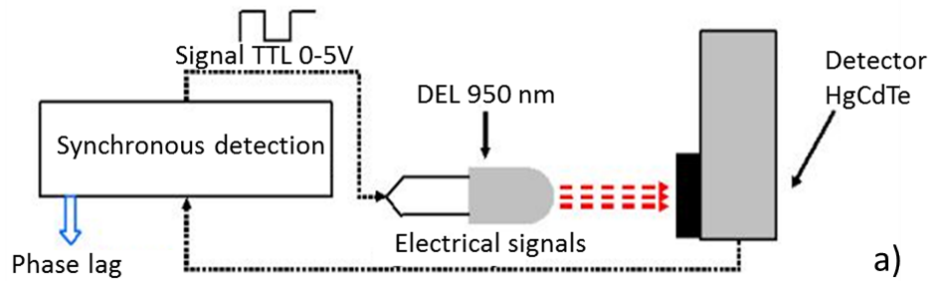
Figure 24. The infrared detector measures the LED signal, driven by the internal TTL generator of the lock-in amplifier.
