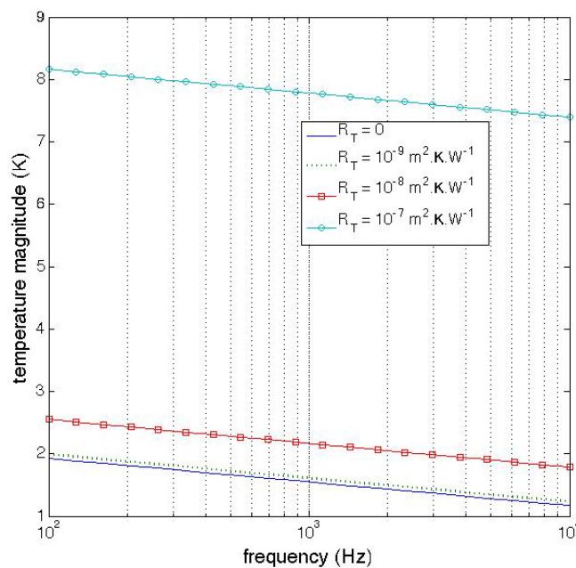
Figure 31: amplitude calculated for the substrate of thickness e_s=0.6 mm with different values of R_T considering the heat transfer model (relation (3.35)). Parameters are b = 2 \text{ } \mu\text{m} ; l = 2 \text{ mm} ; P = 1 \text{ W} ; k=238 \text{ W} \cdot \text{m}^{-1} \cdot \text{K}^{-1} , a = 1.45 \times 10^{-4} \text{ m}^2 \cdot \text{s}^{-1} (silicon).
