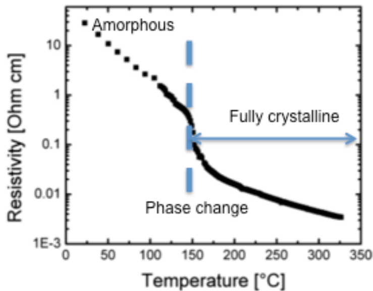
Figure 4: The Ge-Sb-Te electrical resistivity during heating at a constant heating rate of 10^{\circ} \text{C} \cdot \text{min}^{-1} from the amorphous state [13].
