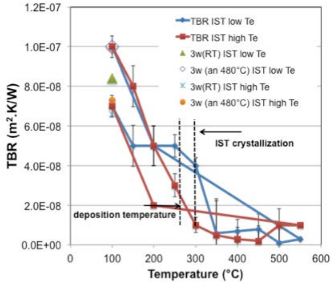
Figure 76: total thermal resistance R for the two Te contents as a function of temperature (blue filled square: comparison with theoretical value calculated using the DMM). The data obtained on as-deposited IST using the 3\omega method for both compositions are also reported.
