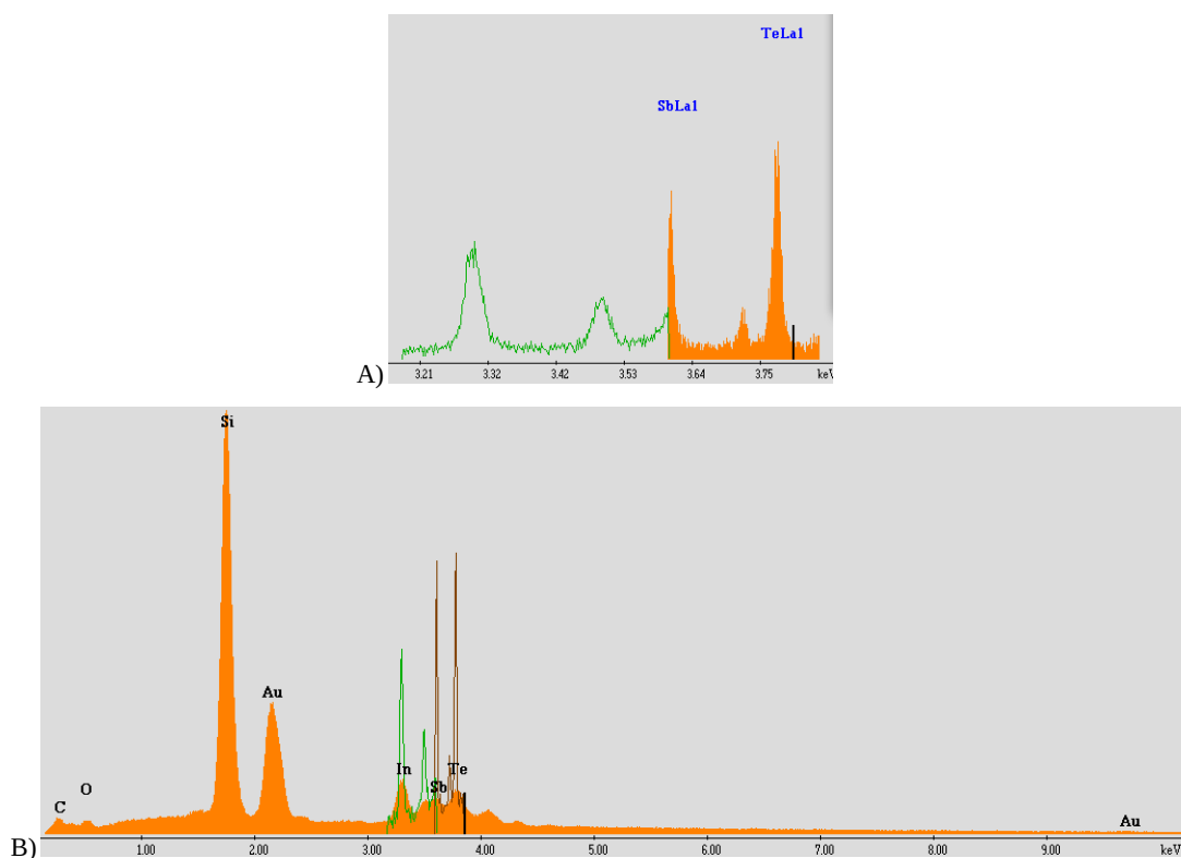
Figure 86: IST 439 sample which was previously heated in situ up to 460°C. WDS spectrum (A) and EDS spectrum (B) acquired on a GRAIN (see right view in Figure 85). The WDS spectra acquired with diffractor 1 (orange) diffractor 5 (green) are not normalized. In view B), the EDS and WDS spectra are superimposed, which allows to clearly see the much higher resolution of the WDS system. .
