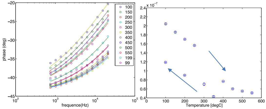
Figure 62: sample MOIST435 (65nm) left: phase calculated (line) with optimal value of R_t and measured (hollow disk); right: identified R_T' in \text{K.m}^2/\text{W} .
