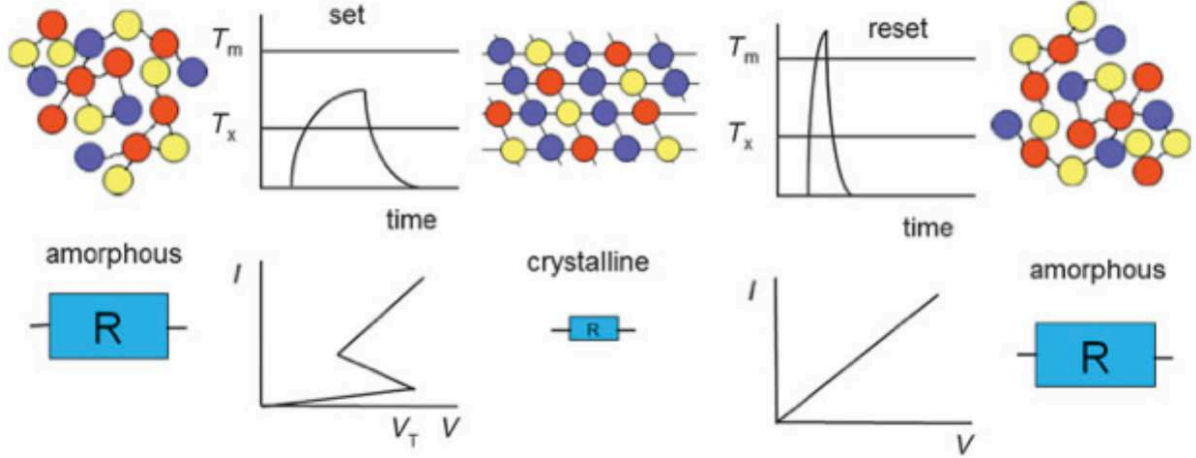
Figure 8: Electrical program of the cell. Starting from the amorphous phase with large resistance R (100 \Omega .cm), a current pulse is applied. At the threshold voltage V_T , the resistance drops suddenly, and a large current ( I ) flows that heats the material above the crystallization temperature T_c for a sufficiently long time to crystallize (SET operation). In the crystalline state, the resistance is low (1m \Omega .cm). A larger, short current pulse is applied to heat the material above the melting temperature T_m . The material is melt-quenched and returns to the amorphous, high resistance state (RESET operation). Figure comes from reference [37].
