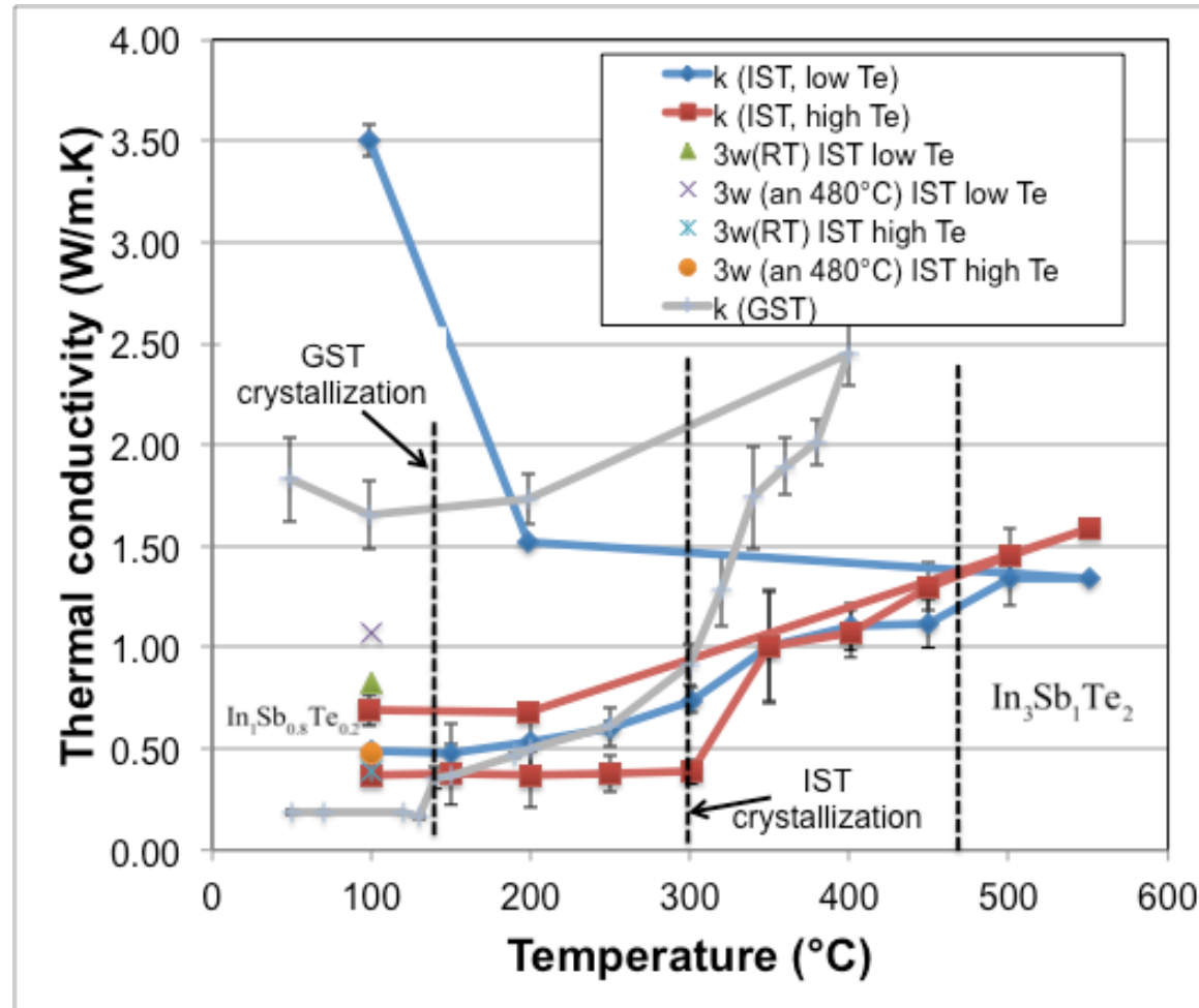
Figure 72: In-Sb-Te thermal conductivity k_{\text{IST}} for the two Te contents, comparison with GST(225). The data obtained on as-deposited IST using the 3 \omega method for both compositions are also reported.
