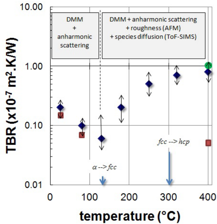
Figure 12: Measurement of the TBR at the interface at the interface between \text{Ge}_2\text{Sb}_2\text{Te}_5 and Al using the Time Resolved Thermorefectance [57].
