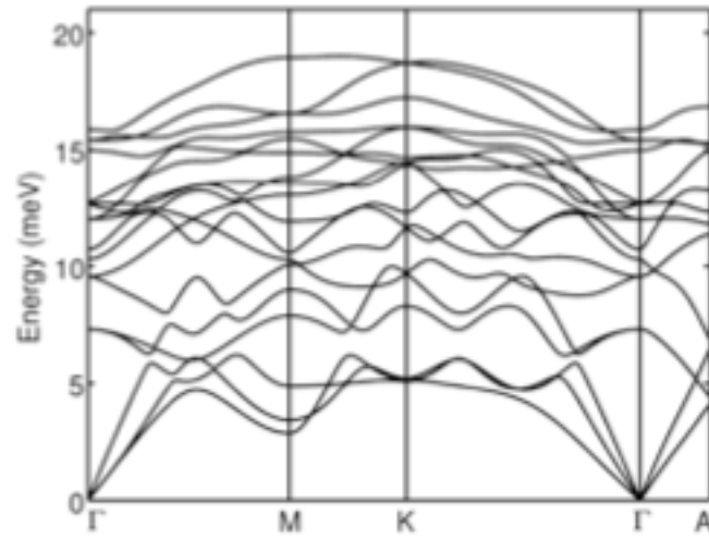
Figure 70: IST(312) dispersion curves \omega(k) calculated using the DFT (calculations preformed by Marco Bernasconi at the UMB).
