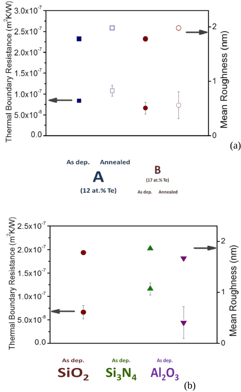
Figure 42: Relationship between thermal boundary resistance (left axis) and mean roughness (right axis) of full stacks of dielectric/IST/dielectric. (a) Results of \text{SiO}_2 -capped batches A (blue squares) and B (red circles), as deposited (full symbols) and after thermal treatment (hollow symbols). (b) Results of the same batch B, sandwiched between \text{SiO}_2 (circles), \text{Si}_3\text{N}_4 (upward triangle) and \text{Al}_2\text{O}_3 (downward triangle).
