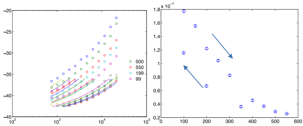
Figure 60: sample MOIST436 (30nm) left: phase calculated (line) with optimal value of R_t and measured (hollow disk); right: identified R_T' in K.m^2/W .
