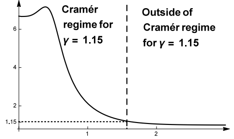
FIGURE 2.4. A representation of the function \gamma_c(\cdot) for the distribution K_h(\cdot) with c = 2.15 , E_b = 6 and E_l = 3 . The horizontal dashed line corresponds to the value of \gamma = 1.15 and the vertical one to the critical point h_{c,\gamma} \simeq 1.676 . Computing \gamma_c(h) is immediate from (2.23) once G(h) and \bar{\lambda}_1(h) are known: we have first obtained G(h) by solving numerically \sum_{n,m} \tilde{K}_h(n,m) = 1 and then we have solved numerically q_h(\bar{\lambda}_1, G) = 1 for \bar{\lambda}_1(h) .
