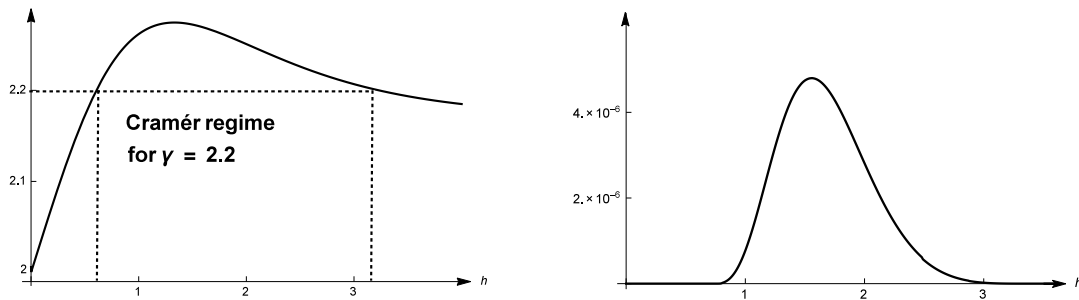
FIGURE 2.5. On the left the function \gamma_c(\cdot) for the inter-arrival distribution K_2(\cdot) , with \alpha = 0.5 and \kappa = 0.01 . The horizontal dashed line corresponds to the value of \gamma = 2.2 . There are two values of h (vertical dashed lines) such that \gamma_c(h) = \gamma and therefore there are two transitions. On the right we plot the difference N(\cdot) - \tilde{F}_\gamma(\cdot) , that is N(\cdot) - \hat{c}_\gamma(\cdot) (recall (2.69) and (2.70)), which makes clear the presence of the two transitions. The resolution of the graph does not allow to appreciate the positivity of such a difference for example at h = 3 where it is about 6 \times 10^{-9} .
