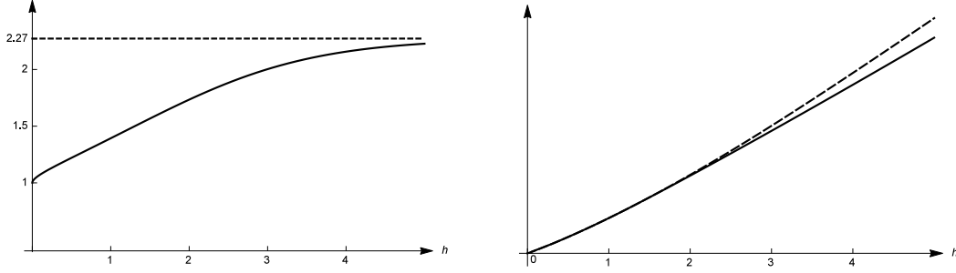
FIGURE 2.6. For the inter-arrival distribution K_3(\cdot) , the function \gamma_c(\cdot) (on the left) is strictly increasing (for \alpha = 1.5, \varrho = 0.02 ), this implies that if \gamma_0 := \lim_{h \rightarrow \infty} \gamma_c(h) \leq \gamma (dashed line represent the value of \gamma_0 computed using (2.25)), there is no transition in the system. On the right, we present the free energy \tilde{F}_\gamma(h) and N(h) (dashed line, recall (2.70)) for \gamma = 1.5 .
