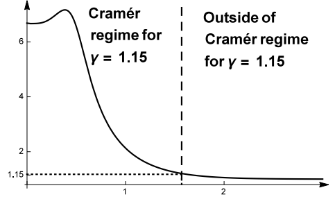
FIGURE 2.4. A representation of the function \gamma_c(\cdot) for the distribution K_h(\cdot) with c = 2.15 , E_b = 6 and E_l = 3 . The horizontal dashed line corresponds to the value of \gamma = 1.15 and the vertical one to the critical point h_{c,\gamma} \simeq 1.676 . Computing \gamma_c(h) is immediate from (2.23) once G(h) and \bar{\lambda}_1(h) are known: we have first obtained G(h) by solving numerically \sum_{n,m} \tilde{K}_h(n,m) = 1 and then we have solved numerically q_h(\bar{\lambda}_1, G) = 1 for \bar{\lambda}_1(h) .
