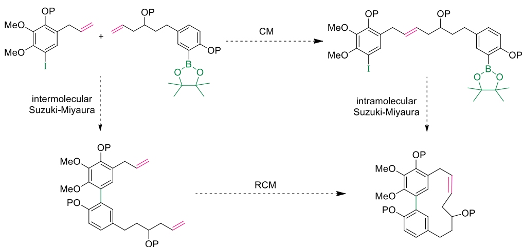
Scheme 6-8 Perspectives on Suzuki-Miyaura coupling with boronic ester
