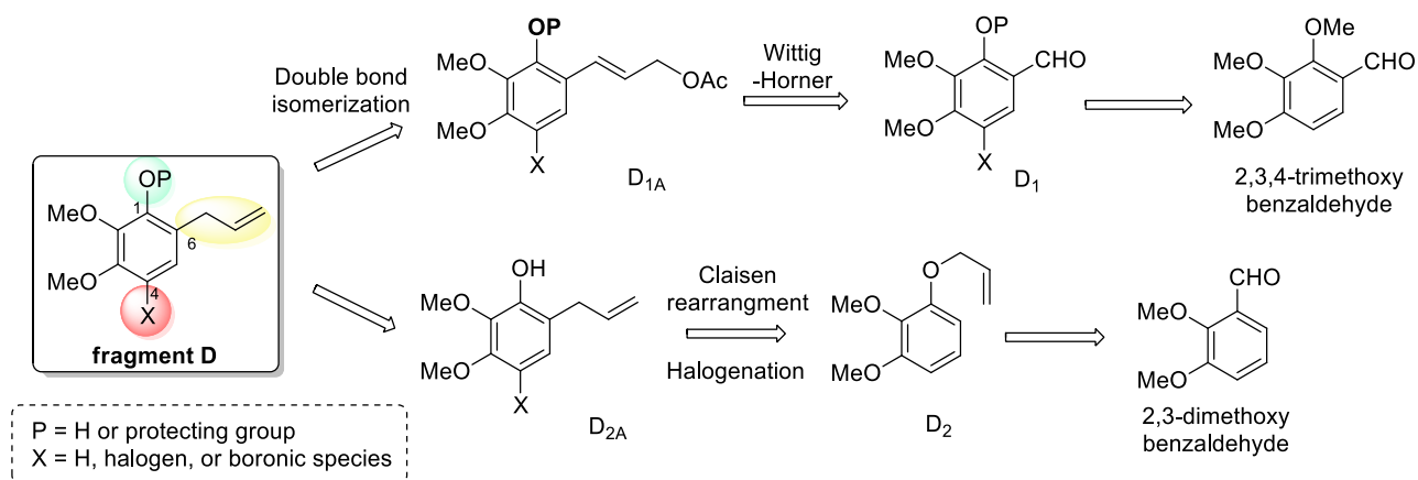
Scheme 4-1 Retrosynthetic approaches to building block D
