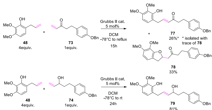
Scheme 4-41 Preparation by CM of linear diarylhexanoids shorter analogues 77 , 78 and 79
