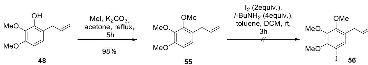
Scheme 4-13 Iodination on a protected phenol with amine- I_2 complex
