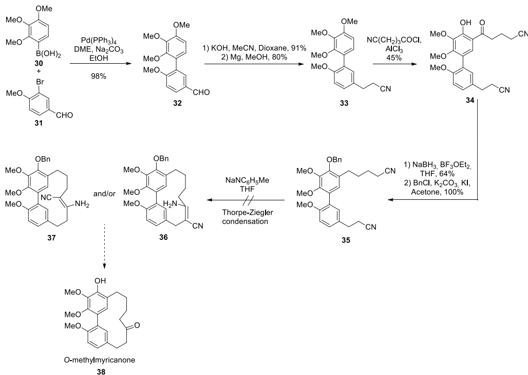
Scheme 2-11 Towards the total synthesis of O -methylmyricanone
