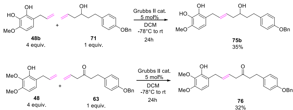
Scheme 4-40 Preparation by CM of linear diarylheptanoids analogues 75b and 76
