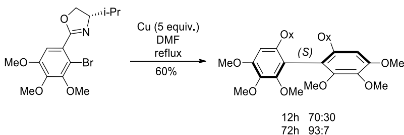
Scheme 4-48 Diastereoselective homocoupling of o -bromooxazolinyllbenzene by Meyers et al.
