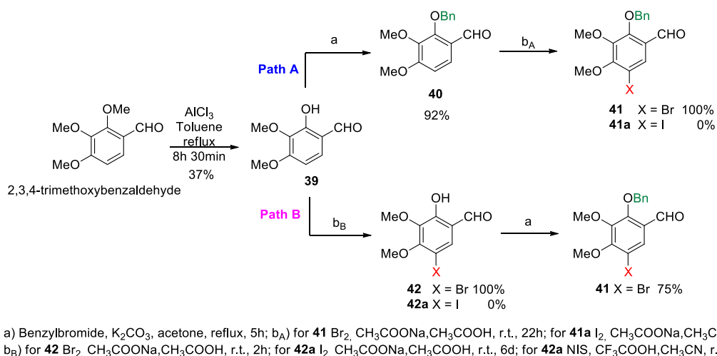
Scheme 4-2 Functionalization of 2,3,4-trimethoxybenzaldehyde
