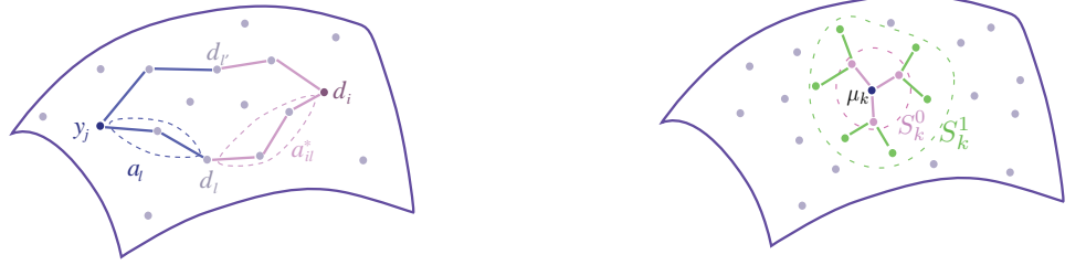
Figure 4.2 – Illustration of AGNN. The affinity between y_j and d_l is a_l , and the affinity between d_l and d_i is a_{il}^* . The intermediate node d_l contributes by the product a_l a_{il}^* to the overall affinity between y_j and d_i . The sample d_{l'} is just another intermediate node like d_l . Summing the affinities via all possible intermediate nodes (i.e., all training samples), the overall affinity is obtained as in (4.9).
