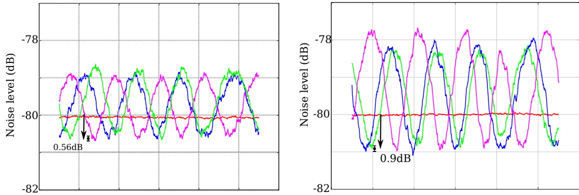
Figure 8.4.: Squeezing and anti-squeezing at 3\text{MHz} for (a) the standard fiber with 70\text{mW} of power and (b) the photonic fiber with 100\text{mW} of power at 3\text{MHz} . We observe 0.56\text{dB} of squeezing and 1.05\text{dB} of anti-squeezing for the standard fiber and 0.9 of squeezing and 1.8\text{dB} of anti-squeezing for the photonic fiber.
