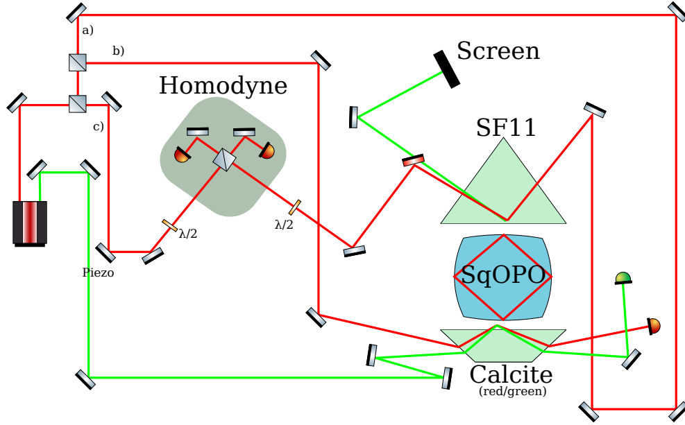
Figure 12.5.: Schematic of the experiment. The Diablo laser is sending a green beam (the pump at 532nm) which is aligned in the green calcite prism. The green light is coupled through the SF11 prism and sent to a screen to observe the mode during locking. The laser also generates some red light (sub-harmonic at 1064nm) that we divide in three. (a) is aligned to the SF11 to observe double resonance, (b) is aligned to the red calcite prism for alignment of the homodyne, and (c) is the LO of the local oscillator. The two calcite prisms can almost be switched without disturbing the alignment.
