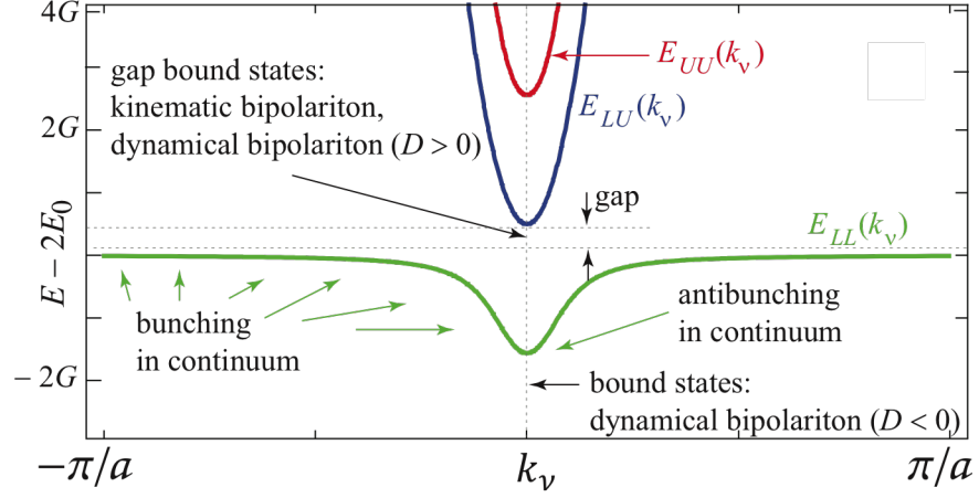
Figure 4.3: Band structure in the two-excitation case. E_{LL}(k_v) = 2E_L(k_v) , E_{LU}(k_v) = E_{UL}(k_v) = E_L(k_v) + E_U(k_v) , E_{UU}(k_v) = 2E_U(k_v) ; a is the lattice constant. The figure summarizes the main results from this chapter.
