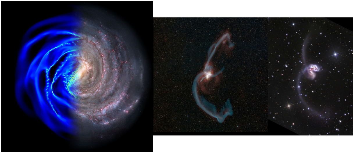
Figure 2.1: Simulations compared to observations. Left : the Milky Way simulation from F. Renaud and the Milky Way artist's conception based on observations of the Galaxy and several local galaxies such as M51, by N. Risinger. Right : the Antennae simulation from F. Renaud and H \alpha R-L-RGB observations of the Antennae at the Cerro Tololo Inter-American Observatory (CTIO) by J. Thibert. Credit: F. Renaud.
