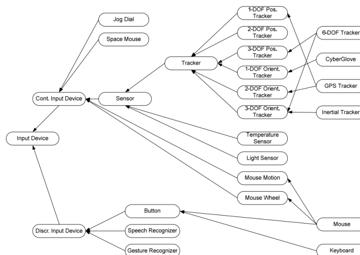
FIGURE 4.3 – The hierarchy for input devices proposed by DEVAL [Ohlenburg et al., 2007]. This hierarchy includes a wide variety of input device units including trackers, buttons and gesture recognizers.
