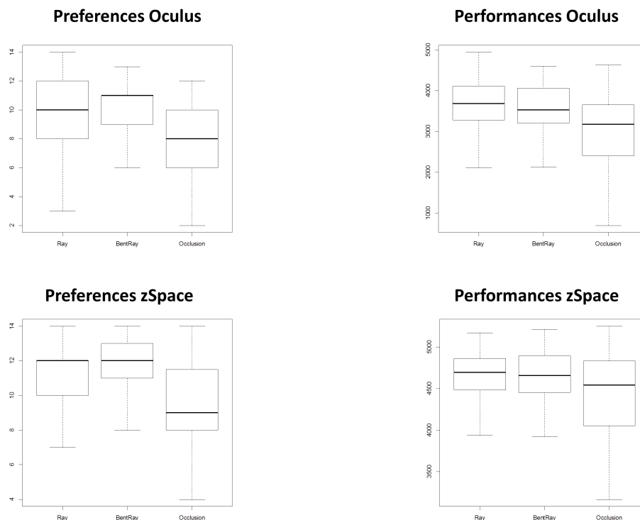
FIGURE 7.6 – Comparison of the preferences and performances results for the three techniques on the two device setups. The results for the 3D Ray-based interaction technique and the 3D Bentray are similar. However, the 3D Bentray seems to be preferred on the zSpace. We can also see that participants less preferred and less performed with the Occlusion selection technique.
