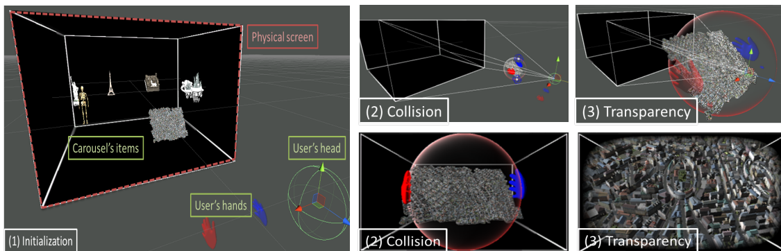
FIGURE 5.9 – Illustrative use case (inspired from [Gaucher et al., 2013]) of the manipulation technique smartly merging the two proposed approaches to handle frame cancellation. The user is interacting with a virtual carousel carrying several virtual objects (1). The user can turn the whole carousel and manipulate the front object. The object can be a map that the user can bring very close to him/her with the collision detection-based approach activated (2). Then, he/she can switch the manipulation mode to scale the map and perceive small details with the virtual alpha blended window approach activated (3). The first line shows the scene from an external point of view while the second line is captured from the user’s point of view.
