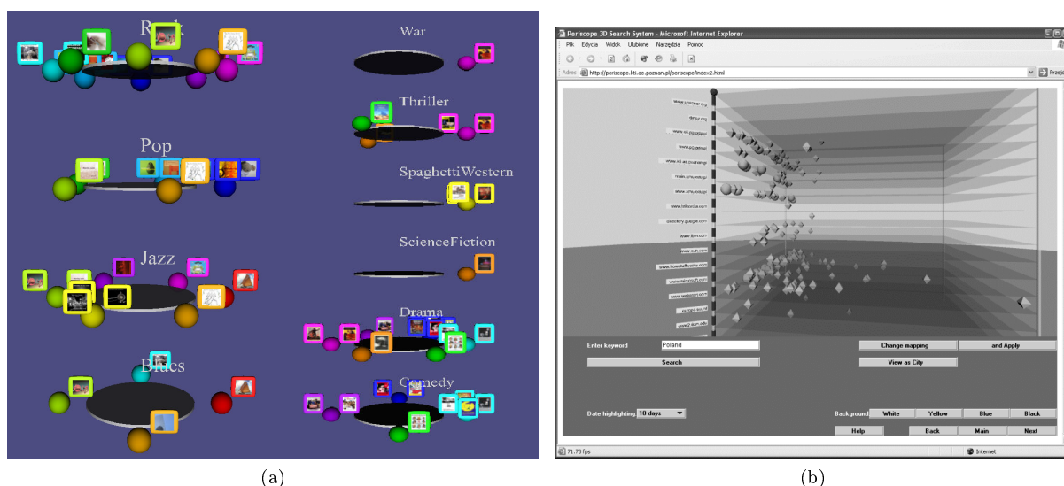
FIGURE 8.2 – Two examples of automatic creation of data visualization interfaces. (a) The visualization of two different databases (Music and Movies) with the same visualization metaphor (a tower of carousels) [Esnault et al., 2010]. (b) An example of analytical interface created with the Periscope system [Wiza et al., 2004].
