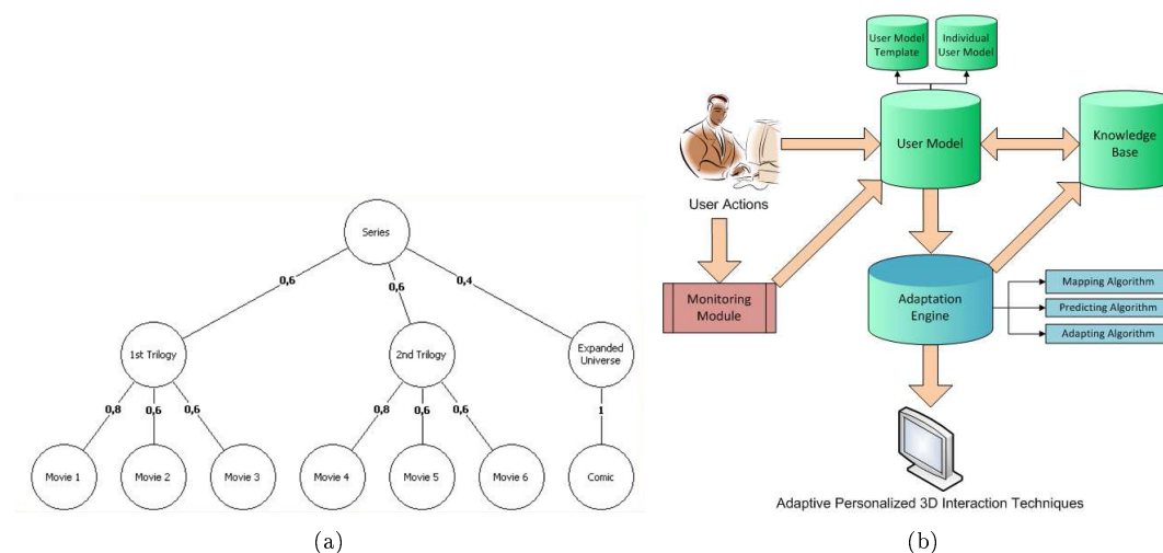
FIGURE 7.2 – Two software solutions for user adaptation (a) In [Bonis et al., 2009] a user model is represented by a semantic graph with scores of interest (b) The conceptual framework for adaptation and personalization in VEs proposed by Octavia et al. [Octavia et al., 2009].
