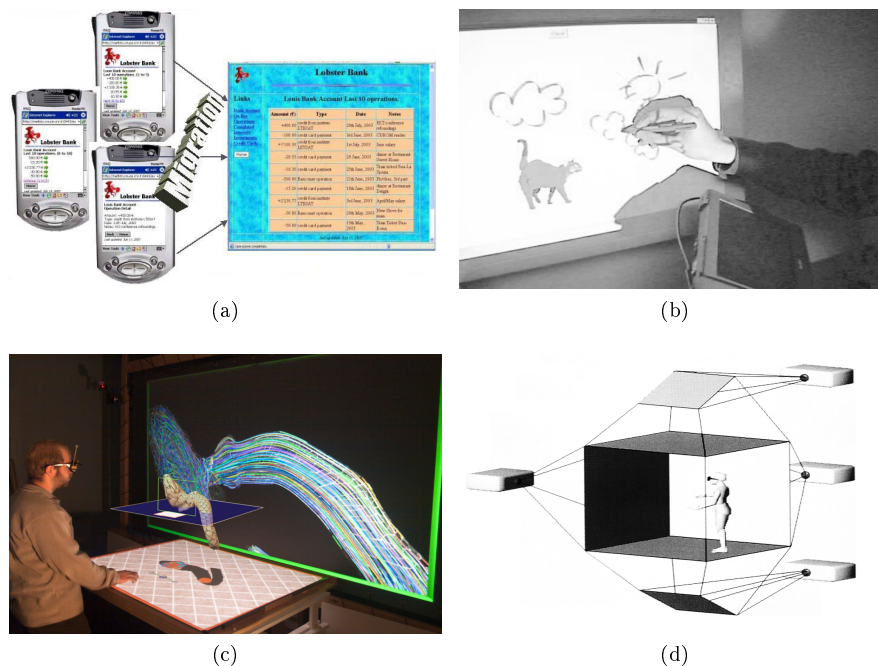
FIGURE 6.2 – Four examples of distribution at different levels. (a) A bank application that can be redistributed at the application level [Bandelloni and Paternò, 2004]. (b) The painter metaphor [Rekimoto, 1997] is an example of distribution at the workspace level. (c) Slice WIM [Coffey et al., 2011] is an example of distribution at the domain concept level. (d) A CAVE [Cruz-Neira et al., 1992] is an example of distribution at the pixel level.
