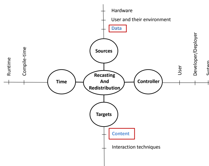
FIGURE 8.1 – Regarding our design space problem of plasticity for MR user interfaces, this chapter is interested in adapting the content visualization of an application according to data structure and semantics. At a lower level, we also show that the data can also be combined with the devices properties and the users properties.
