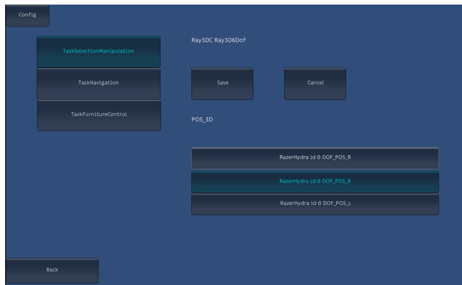
FIGURE 4.15 – An illustration of the meta-user interface. Here is an example where the user can change a device unit associated to a logical driver from a list of compatible ones. For the 3D ray-based interaction technique controlled with the Razer Hydra, the user can change which controller manipulates the ray position. It can be the one on the right or the one on the left.
