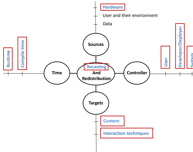
FIGURE 4.1 – Regarding our design space problem of plasticity for MR user interfaces, this chapter is interested in adapting the interaction techniques and the content visualization according to the devices. The basis of our models are also described in this Chapter so we also describe how we can handle the different adaptation times and adaptation controllers.
