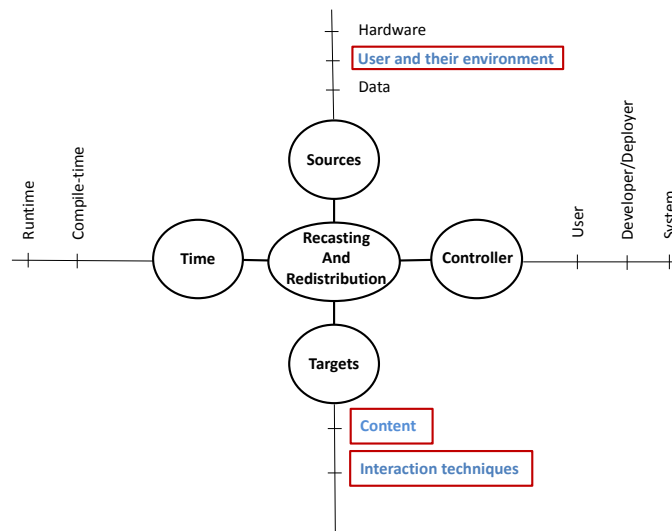
FIGURE 7.1 – Regarding our design space problem of plasticity for MR user interfaces, this chapter is focused on adapting the interaction techniques and the content visualization of an application according to the user properties.
