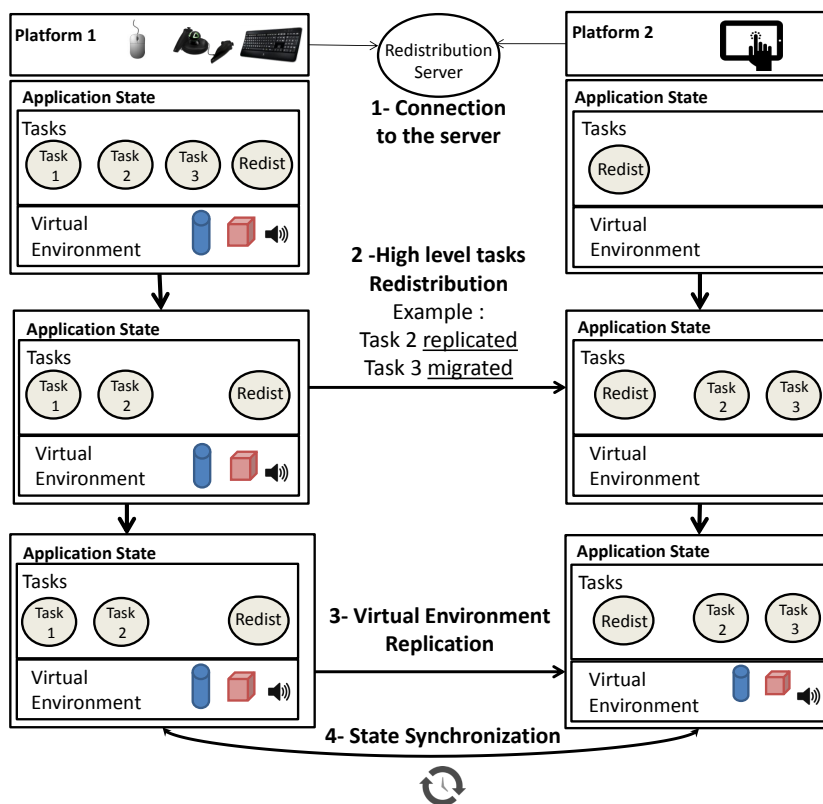
FIGURE 6.4 – With D3PART, the redistribution process is performed in four steps. First, the different platforms connect to the redistribution server. An empty application runs on these distant platforms. It only contains the redistribution task. Then, the user initiates a new distribution of the system with the meta-user interface. Here he chooses to replicate the task 2 and to migrate the task 3 to a second platform. For these two tasks, thanks to the dynamic recasting mechanism handled with our adaptation process, compatible application components are automatically deployed on the second platform that fits its capabilities. The third step consists in replicating the VE from the first platform to the second one. It includes 3D meshes, their materials, and sound assets. We ensure that the state of the application remains consistent during the redistribution. Then in the last step, the redistribution server ensures state synchronization between the two platforms while the applications are running.
