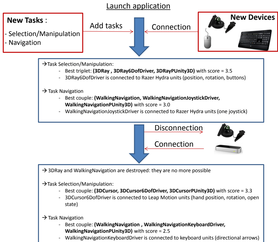
FIGURE 4.14 – A usage scenario of the furniture planning application developed with 3DPlastic-Toolkit. It demonstrates how the application can handle context changes: here the replacement of an interaction device by another one. This example represents the adaptation steps that correspond to the transition from the situation illustrated in Figure 4.12a to the one illustrated in Figure 4.12b
