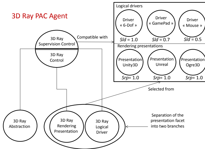
FIGURE 4.11 – The PAC agent of the 3D ray-based technique. This agent is compatible with three concrete logical drivers and three rendering presentations. As shown each compatibility is ranked with a score.
