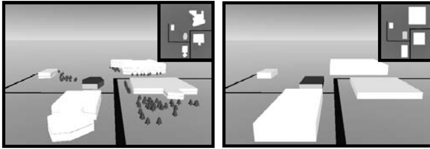
FIGURE 3.2 – In the solution proposed by Bilasco [Bilasco et al., 2007], a 3D scene can be adapted according to the semantic of each element. Here, in the image on the right, the geometries of type "building" have been degraded, and the geometries of type "tree" have been removed from the scene.
