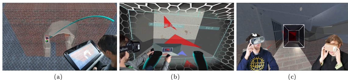
FIGURE 5.10 – Collaborative manipulation of a virtual object (here, a cube) based on an asymmetric setting between two users who can be helped by two additional users. With 3DPlasticToolkit each user benefits from the adapted interaction technique, the adapted point of view and the adapted scene visualization according to his/her device setup in order to ensure an efficient collaboration. (a) The first participant has a global view of the scene and moves the object with a 3D bent ray. (b) The second user is placed inside the object and precisely rotates and scales it. (c) Two additional roles can be added. The first one helps to scale the object using a third person view of it. The other one is a spectator who switches between the other participants' viewpoints and helps them with oral communication.
