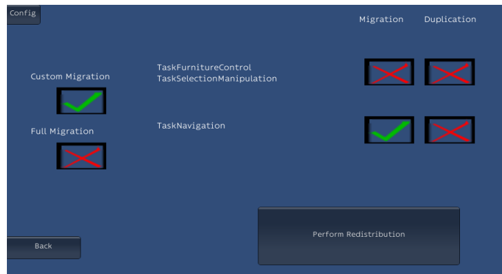
FIGURE 6.5 – The extension of the meta-user interface to control the redistribution process. Here, the user chooses the high level tasks that will be redistributed to the distant platform. In this example based on the furniture planning application, three tasks can be redistributed: navigation, selection/manipulation and furniture control. The last two ones are dependent. The user chooses a partial migration, only the navigation task will be redistributed. The two others tasks remain on his current platform.
