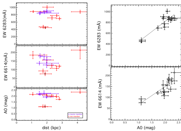
Fig. 11. NGC 4815 field: ( left ) DIB and A_0 distance profiles. Stars identified by Friel et al. (2014) as cluster members correspond to blue, non-members to red markers. Right : 6283 (top) and 6614 (lower panel) Å DIB EW vs the estimated extinction A_0 . The black “0” sign indicates the unique star with a single DIB velocity, for all other targets the adjustment to the data requires two velocity components.
