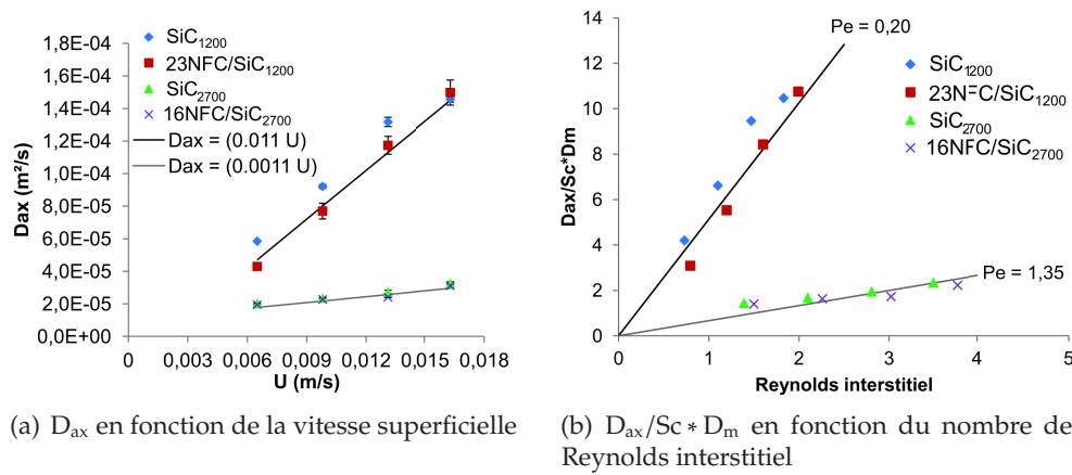
Figure 3.6 Dispersion axiale
