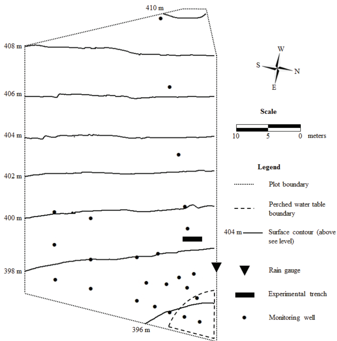
Figure 55: Plot and perched water table boundaries, surface contour, rain gauge, and experimental trench positions
