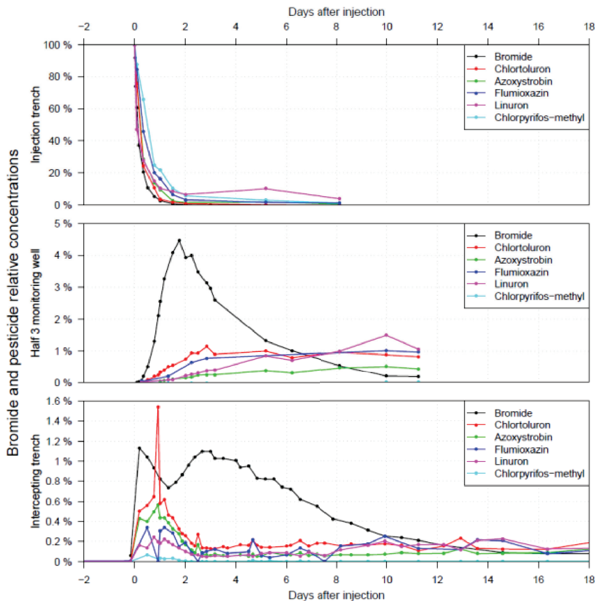
Figure 68: Relative concentrations of bromide, chlortoluron, azoxystrobin, flumioxazin, linuron and chlorpyrifos-methyl, in the injection trench (top of the figure), in Half-3 monitoring well (center of the figure), and in the intercepting trench (bottom of the figure). Points correspond to measured values, and lines are plotted to help reading.
