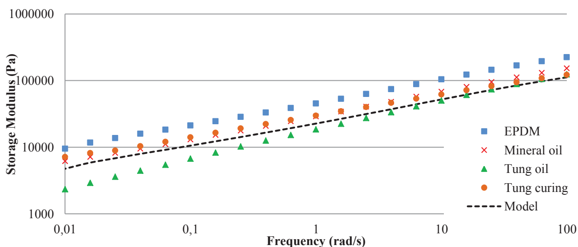
Fig. 10. Variation of the storage modulus G' versus frequency (rad/s) for the pure EPDM and EPDM plasticized with 30%w of different oils at 160^\circ\text{C} .
