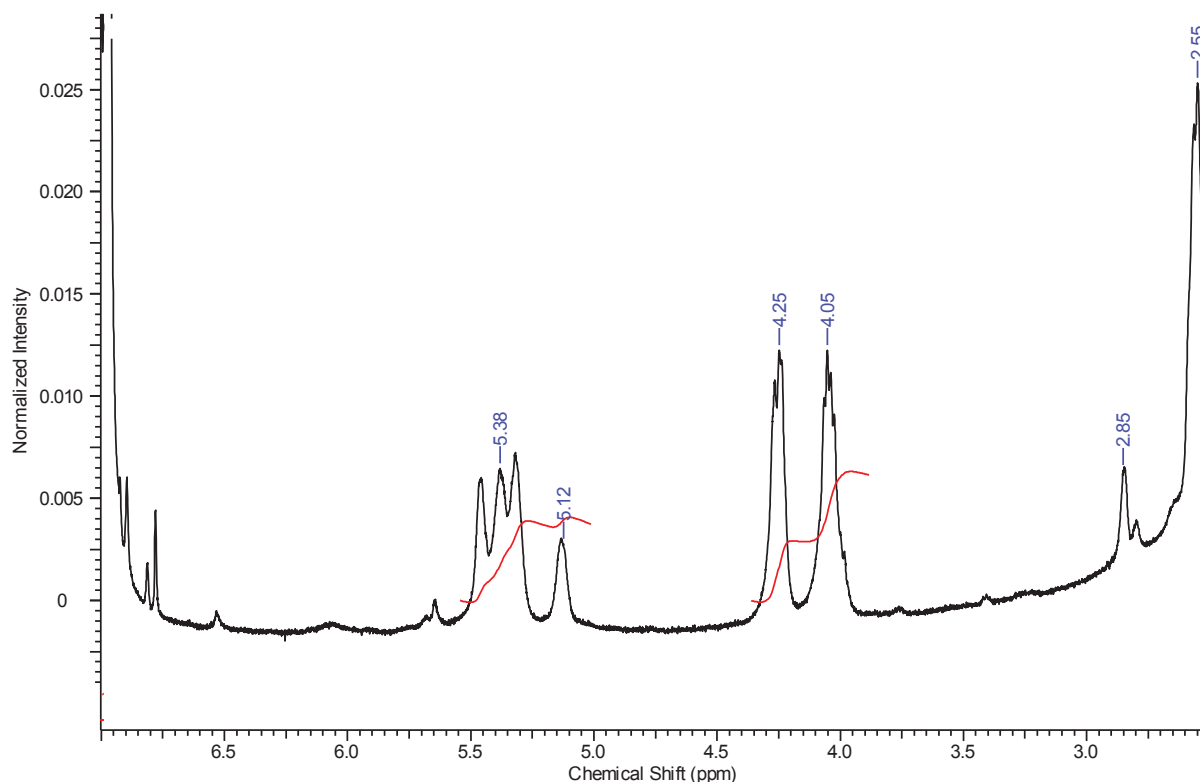
Fig. 12. Liquid ^1\text{H} NMR spectrum of the system EPDM/FFM and Tung oil curing at 250^\circ\text{C} during 5 min, center between 2.5 and 7.0 ppm (toluene d_8 at 30^\circ\text{C} ). Sample was taken at t = 35 min (point C on the Fig. 8)
