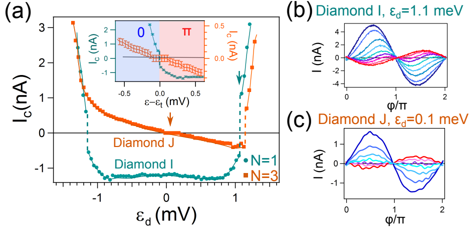
FIGURE 5.15 – (a) Critical current I_c , defined as the maximum amplitude of the measured switching current, as a function of the energy level \epsilon . I_c is defined as positive for a 0-junction, and negative for a \pi -junction. This quantity is plotted for the two diamonds I ( N=1 , blue dots) and J ( N=3 , orange squares), respectively in the single-level and two-level regime. The dashed lines materialize discontinuities of I_c , specific of first order transitions. Inset : focus on two 0- \pi transitions, centered around \epsilon_t (see Fig. 5.11.(c) for the definition) : at \epsilon = -1.1 meV in diamond I, and at \epsilon = 0.1 meV in diamond J. (b) Current-phase relations around the 0- \pi transition in diamond I, at \epsilon_d = 1.1 meV, indicated by a green arrow. The CPR becomes anharmonic and the critical current never vanishes. (c) Current-phase relations around the 0- \pi transition in diamond J, at \epsilon_d = 0.1 meV, indicated by an orange arrow. The CPR is harmonic all over the transition, and the critical current vanishes at the transition.
