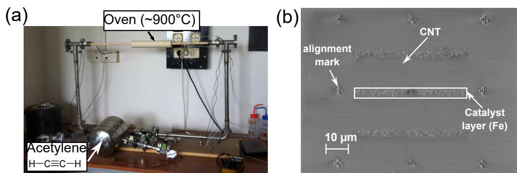
FIGURE 3.2 – (a) Optical picture of the oven used to make the nanotube CVD synthesis. A temperature around 900^{\circ}\text{C} is obtained making a current pass through a metallic wire around an alumine tube. It is controlled with a thermocouple connected to a voltmeter. (b) SEM image (inlens captor, see text) showing a typical sample after the CVD growth. One can see the alignment marks, the three lines of iron catalyst, as well as the nanotubes.
