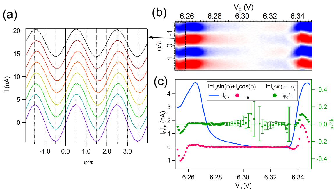
FIGURE 5.17 – (a) Current-phase relations for various values of gate voltage on the left edge of the gate voltage region (square in black on (b)). We can see that these CPRs look sinusoidal and that some of them are slightly dephased (in particular the red and orange). (c) Result of sinusoidal fits all over the diamond. In blue and pink are represented the critical current I_0 and the anomalous current I_a from I = I_0 \sin(\varphi) + I_a \cos(\varphi) , in green the phase shift \varphi_0 from I = I_c \sin(\varphi + \varphi_0) . Note that the error bar diverges at the 0-\pi transitions : at the center where the amplitude almost vanishes, and on the right edge where the CPRs are strongly anharmonics.
