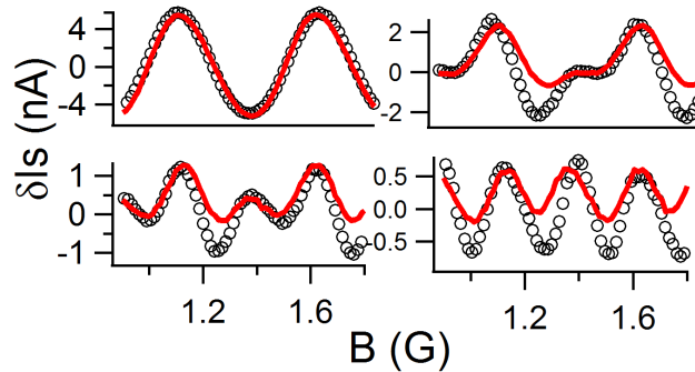
FIGURE 5.13 – Modulation of the switching current at the 0-\pi transition in diamond C with optimization of the environment (in black dots) and without (in red lines). The amplitudes of the optimized curves have been readjusted in order to compare the shapes of the curves.
