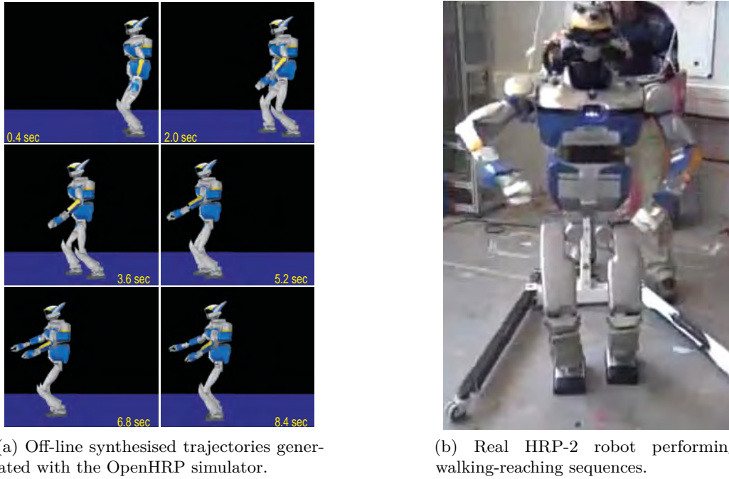
Figure 5.7: Experiment using the HRP-2 in LAAS-CNRS
