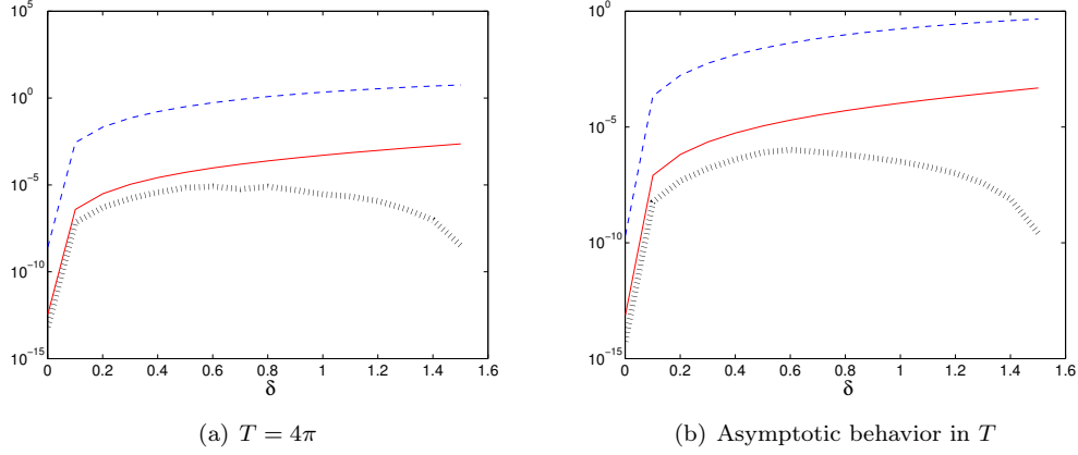
FIGURE 2.3 – a(\cdot) = 0 and \omega = (0, \delta) \cup (\pi - \delta, \pi) . Plots of C_0(T, |\omega|) (– –), C'_{T, T_0, 0, \lambda} (//) and \tilde{C}_{T, T'_0, 0, \lambda} (–) with respect to \delta
