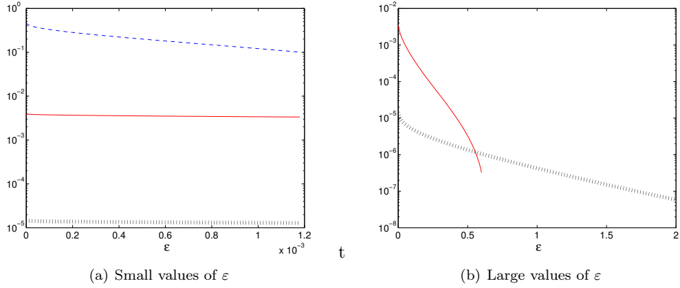
FIGURE 2.4 – a : x \mapsto \varepsilon x , \omega = (0, \frac{3}{2}) and T = 8\pi . Plots of C_a(T, |\omega|) (– –), C'_{T, T_0, a, \lambda} (//) and \tilde{C}_{T, T'_0, a, \lambda} (–) with respect to \varepsilon
