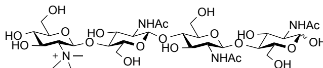
Figure 33 : TMG-chitotriomycin
