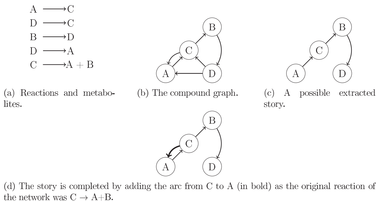
Figure 2.7: Procedure for verifying the acyclicity of the solution in the compound graph for the network in Figure 2.7a and represented as a compound graph in Figure 2.7b. One of the possible stories is shown in Figure 2.7c. The arc going from C to B is part of a reaction that also produces A. When the new arc C \rightarrow A is added, the solution is no longer acyclic (Figure 2.7d).
