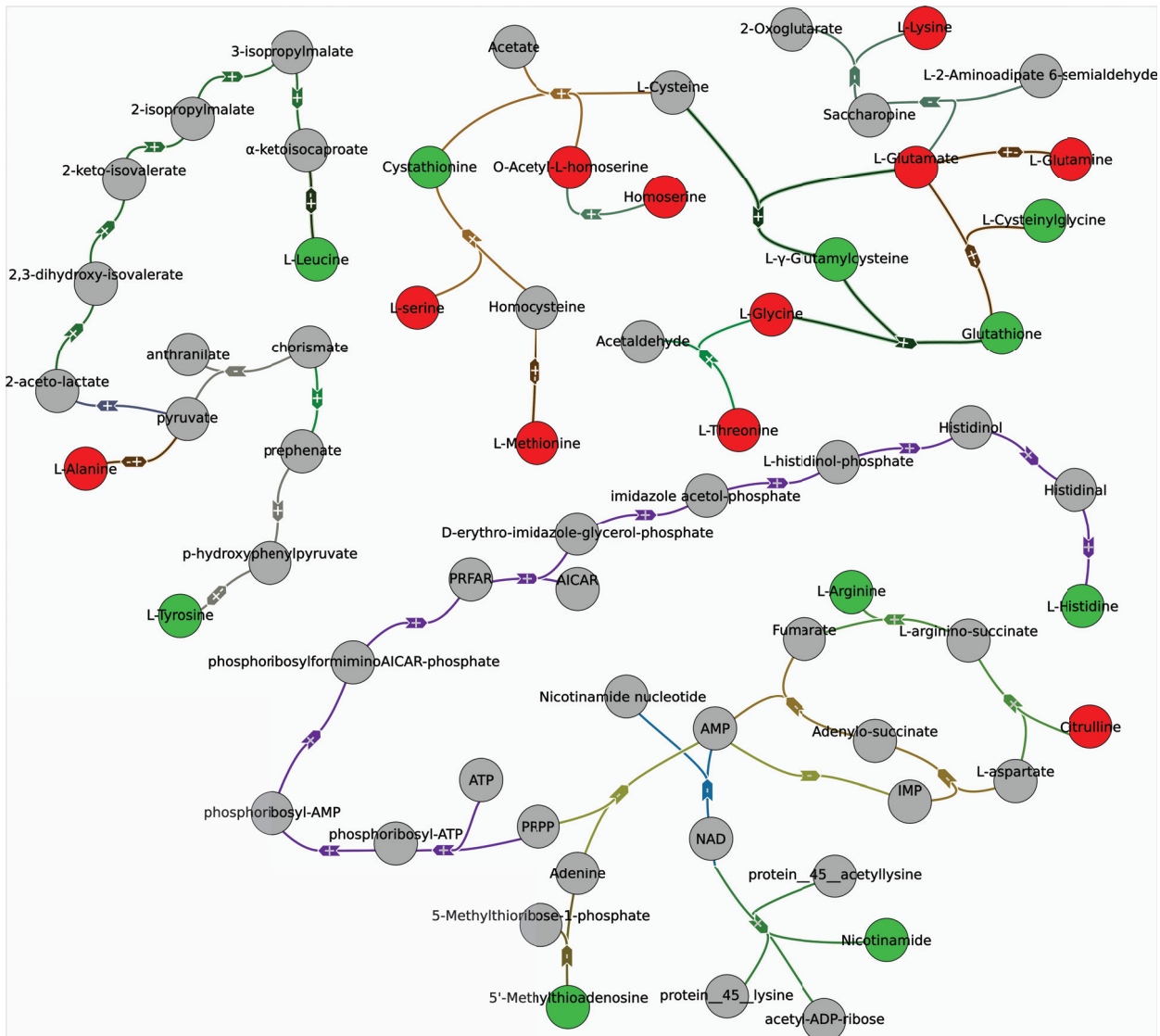
Figure 2.13: Results with 21 black vertices. The number of hyperarcs and of isolated grey vertices is minimised.
