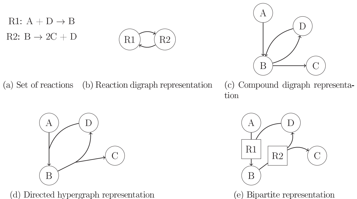
Figure 1.5: Directed graph representations of a set of reactions.
