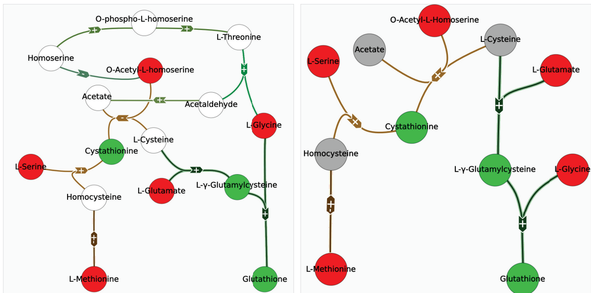
(a) Solution when all vertices are considered (b) Solution with grey vertices. The number of white (no isolated grey vertices). hyperarcs and of isolated grey vertices is minimised.
