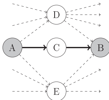
Figure 2.4: Example of the lightest path compression. Here, there are three paths linking the vertices A and B. D has a degree of 7, whereas E has a degree of 6 and C has a total degree of 2. The lightest path linking the vertices A and B is thus the one going through C indicated in bold. After the lightest path compression, there will be only 2 arcs remaining, A \rightarrow C \rightarrow B .
