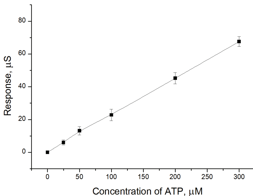
Figure 26. Typical calibration curve of HEX-based conductometric biosensor for the determination of ATP concentration. Glucose concentration: 200 \mu\text{M} . Working buffer: 5 mM HEPES, pH 7.4, 3 mM of \text{Mg}^{2+} . Data is presented as the mean of three biosensor responses \pm standard deviation.
