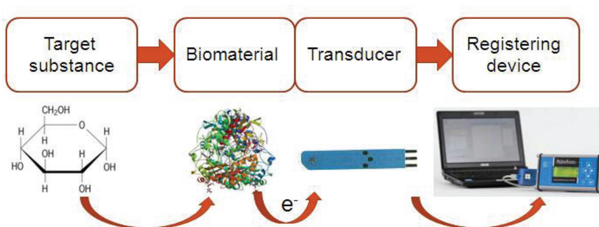
Figure 1. General working principle of a biosensor (top) and principle of the amperometric glucose biosensor (bottom).
