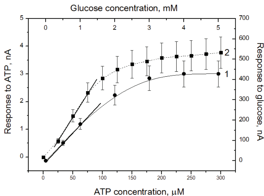
Figure 14. Typical calibration curves of GOX/HEX biosensor for the determination of glucose (1) and ATP (2). Calibration curve for ATP determination was plotted at glucose concentration of 50 \mu\text{M} . Measurements were carried out in 25 mM HEPES buffer, pH 7.4, with 2 mM \text{Mg}^{2+} , constant potential of 0.6 V vs Ag/AgCl reference electrode. Data is presented as the mean of five biosensors \pm standard deviation.
