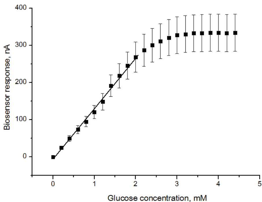
Figure 16. An average calibration curve ( n=5 ) of GOx-based biosensor for glucose determination. Measurements were carried out in 25 mM HEPES buffer, pH 7.4, with 2 mM Mg^{2+} , the constant potential of 0.6 V vs Ag/AgCl reference electrode. Data is presented as the mean of five biosensors \pm standard deviation.
