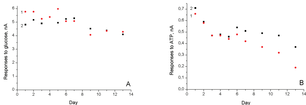
Figure 15. Responses to 50 μM glucose (A) and 25 μM ATP (B) of the biosensor based on GOx and HEX stored dry for two weeks at temperatures of +4 °C (1) and -18 °C (2). Measurements were carried out in 25 mM HEPES buffer, pH 7.4, with 2 mM Mg 2+ , constant potential of 0.6 V vs Ag/AgCl reference electrode.
