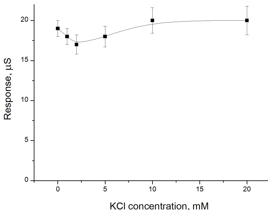
Figure 24. Influence of KCl concentration on biosensor response. ATP concentration: 100 \mu\text{M} , glucose concentration: 200 \mu\text{M} . Data is presented as the mean of three biosensors \pm standard deviation.
