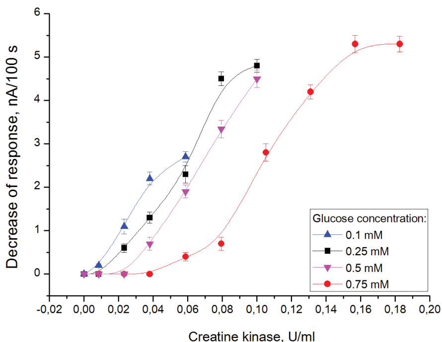
Figure 19. Calibration curves for creatine kinase determination, obtained at different concentrations of glucose in the working cell. Measurements were carried out in 10 mM HEPES buffer, pH 7.4, with 10 mM Mg^{2+} , 1 mM ADP, 10 mM creatine phosphate, at the constant potential of 0.6 V vs Ag/AgCl reference electrode. Data is presented as the mean of three biosensor responses \pm standard deviation.
