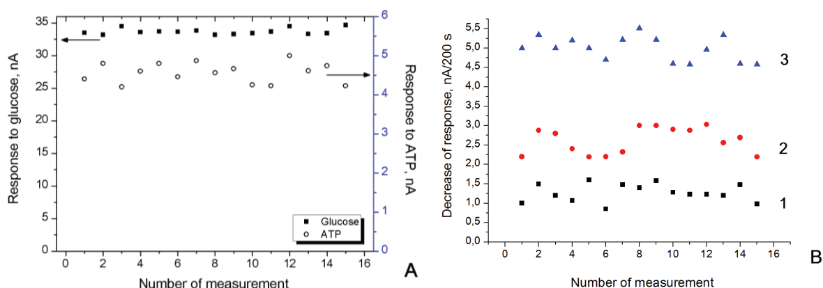
Figure 20. Reproducibility of biosensor responses to glucose and ATP (A), and to different concentrations of CK (B): 0.013 U/ml (B, 1), 0.038 U/ml (B, 2), 0.1 U/ml (B, 3). Glucose concentration – 0.25 mM, ATP – 0.1 mM. Measurements were carried out in 10 mM HEPES buffer, pH 7.4, with 10 mM \text{Mg}^{2+} , 1 mM ADP, 10 mM creatine phosphate, at the constant potential of 0.6 V vs Ag/AgCl reference electrode.
