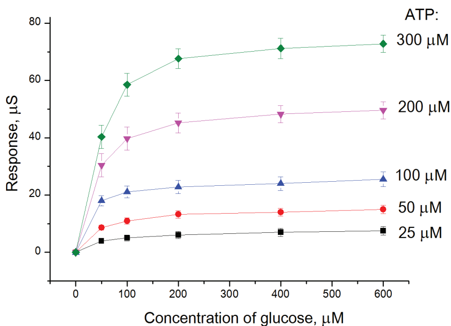
Figure 25. Influence of glucose and ATP concentrations on the biosensor response curves.
