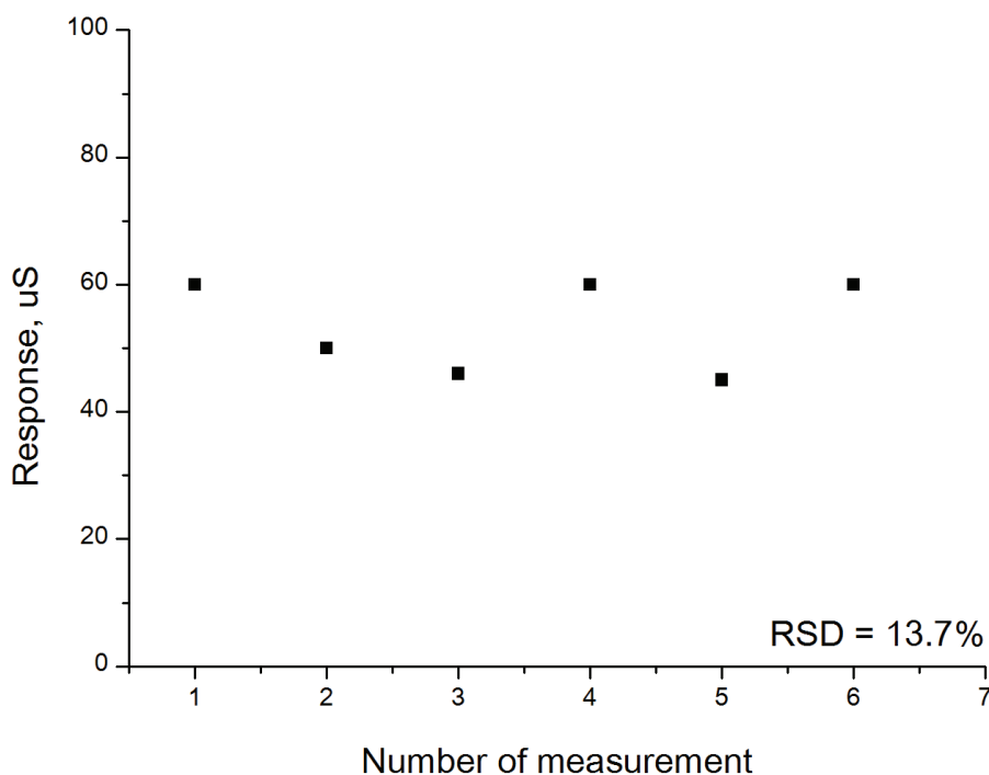
Figure 29. Repeatability of biosensor responses to ATP in one pharmaceutical sample (91-fold dilution). Working buffer: 5 mM HEPES, pH 7.4, 3 mM of Mg^{2+} . Concentration of glucose: 400 \mu M.
