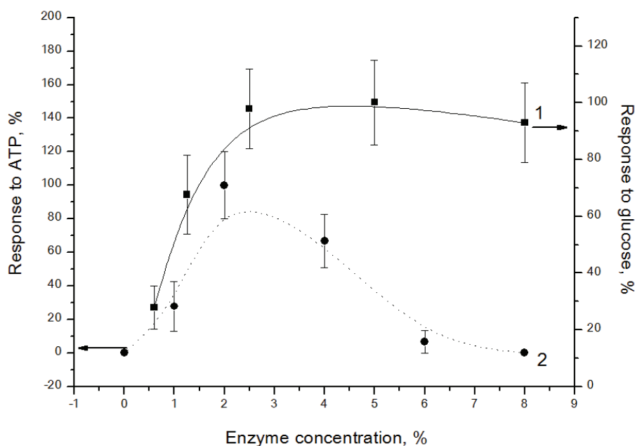
Figure 12. Dependence of biosensor response to 4 mM glucose (1) and 0.1 mM ATP (2) on concentrations of GOx (1) and HEX (2) in biorecognition element. The highest biosensor response was taken as 100%. When selecting HEX concentration, GOx concentration in biomembranes was 2%. Measurements were carried out in 25 mM phosphate buffer with 2 mM Mg^{2+} , pH 7.4, at constant potential of 0.6 V vs Ag/AgCl reference electrode. Data is presented as the average value of four biosensors \pm standard deviation.
