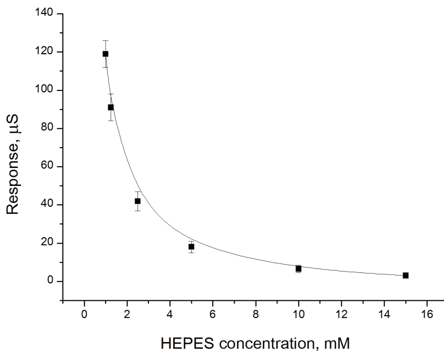
Figure 23. Influence of working buffer concentration on biosensor response. Buffer pH: 7.4. ATP concentration in buffer: 100 \mu\text{M} , glucose concentration: 200 \mu\text{M} . Data is presented as the mean of three biosensors \pm standard deviation.
