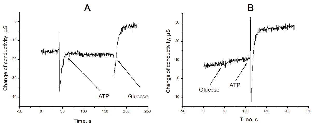
Figure 21. A: typical biosensor responses during measurements of the ATP concentration (first ATP or sample is added, and then glucose). B: control experiment, first glucose is added, and then ATP. Concentration of ATP was 100 \mu\text{M} , glucose – 200 \mu\text{M} .
