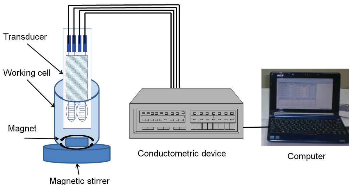
Figure 10. Scheme of a setup for conductometric measurements.
