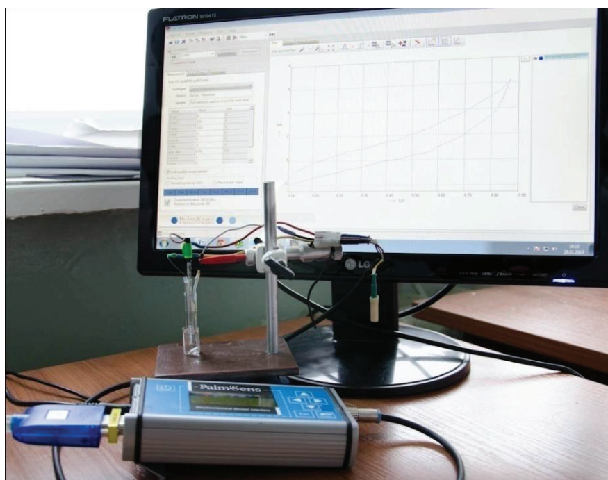
Figure 7. Photograph of the working area, presenting the PalmSens potentiostat, the electrochemical cell with conventional three electrode system, and the computer used during the amperometric experiments.
