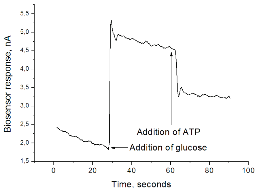
Figure 11. Example of the GOX/HEX biosensor response to subsequent additions of glucose (75 \mu\text{M} ) and ATP (50 \mu\text{M} ). Measurements were carried out in 25 mM phosphate buffer with 2 mM \text{Mg}^{2+} , pH 7.4, at constant potential of 0.6 V vs Ag/AgCl reference electrode.
