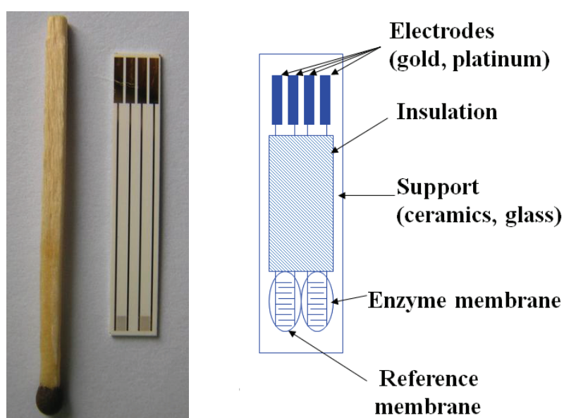
Figure 6. A photograph (on the left) and a scheme (on the right) of the conductometric transducer used in this work.
