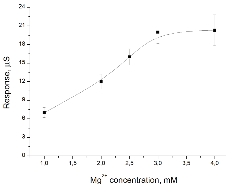
Figure 22. Influence of magnesium ions concentration in working buffer on biosensor response. Concentration of ATP was 100 \mu\text{M} ATP, glucose – 200 \mu\text{M} . Data is presented as the mean of three biosensors \pm standard deviation.
