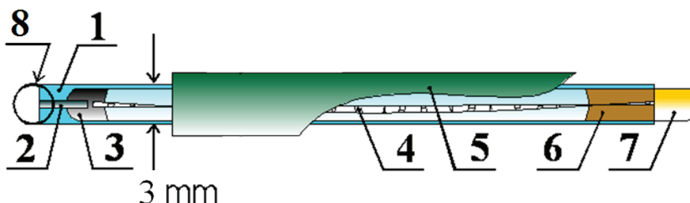
Figure 5. Scheme of the working amperometric electrode.
