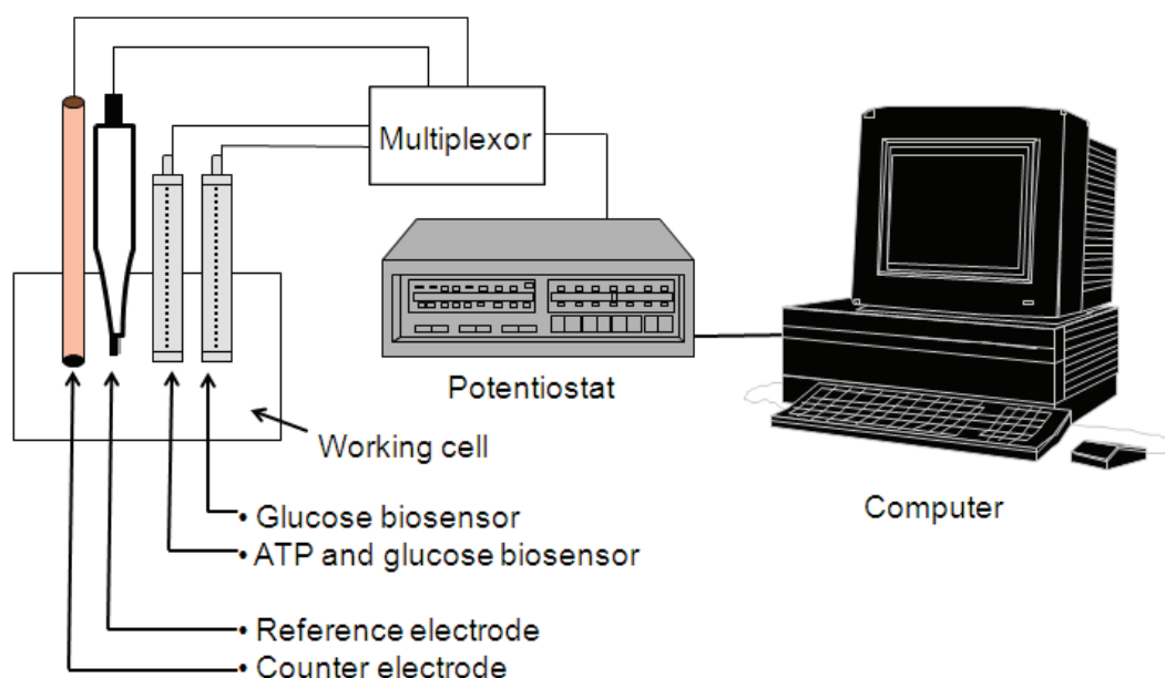
Figure 8. Scheme of a biosensor system.
