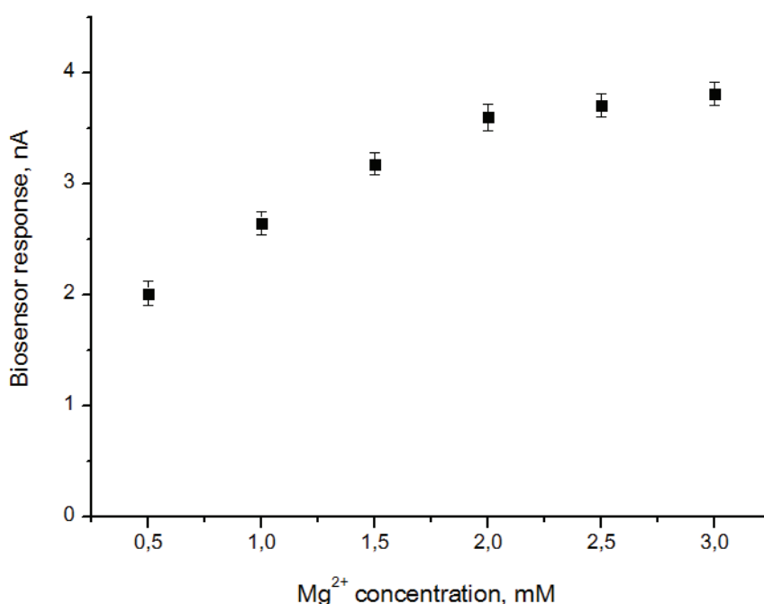
Figure 13. Influence of Mg^{2+} concentration in working buffer on GOx/HEX biosensor response to ATP. Glucose concentration: 100 \mu M, ATP concentration: 100 \mu M.
