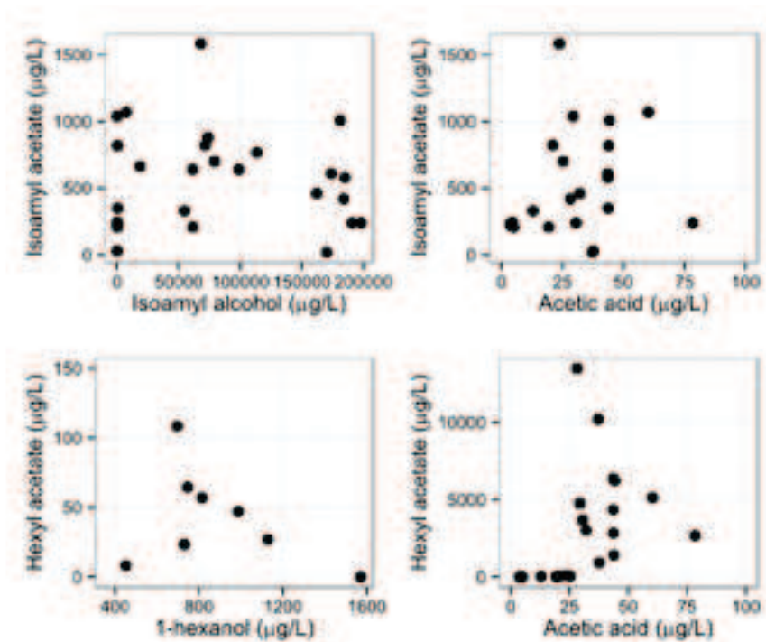
Figure 12. Relationships between the concentrations of acetate esters and their precursors in wines. Concentration of the isoamyl acetate and hexyl acetate is not correlated to the concentration of neither the alcohol nor the acid precursor ( \alpha=0.01 ).
