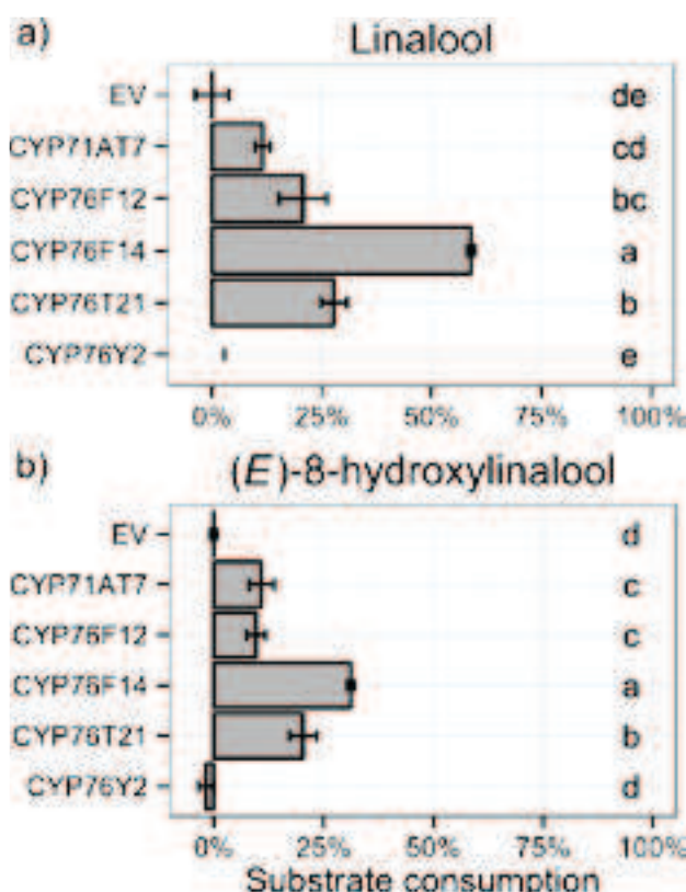
Figure 31. Conversion of linalool and (E)-8-hydroxylinalool by grapevine cytochromes P450 expressed in yeast. Microsomal membranes prepared from yeast expressing the candidate P450s were incubated with substrates at 100 \mu M concentration for 1h in the presence of NADPH. Reaction mixtures were extracted and analyzed by GC-FID. Conversion ( \pm SD, N=3) is calculated relative to the residual concentration of substrate in negative control (microsomal fraction from yeast transformed with an empty vector - EV) incubated under the same conditions. One-way analysis of variance (ANOVA) revealed significant differences ( P < 0.001 ) for both substrates. Letters on the right axes indicate significant differences between means calculated with Tukey HSD test ( \alpha = 0.05 ).
