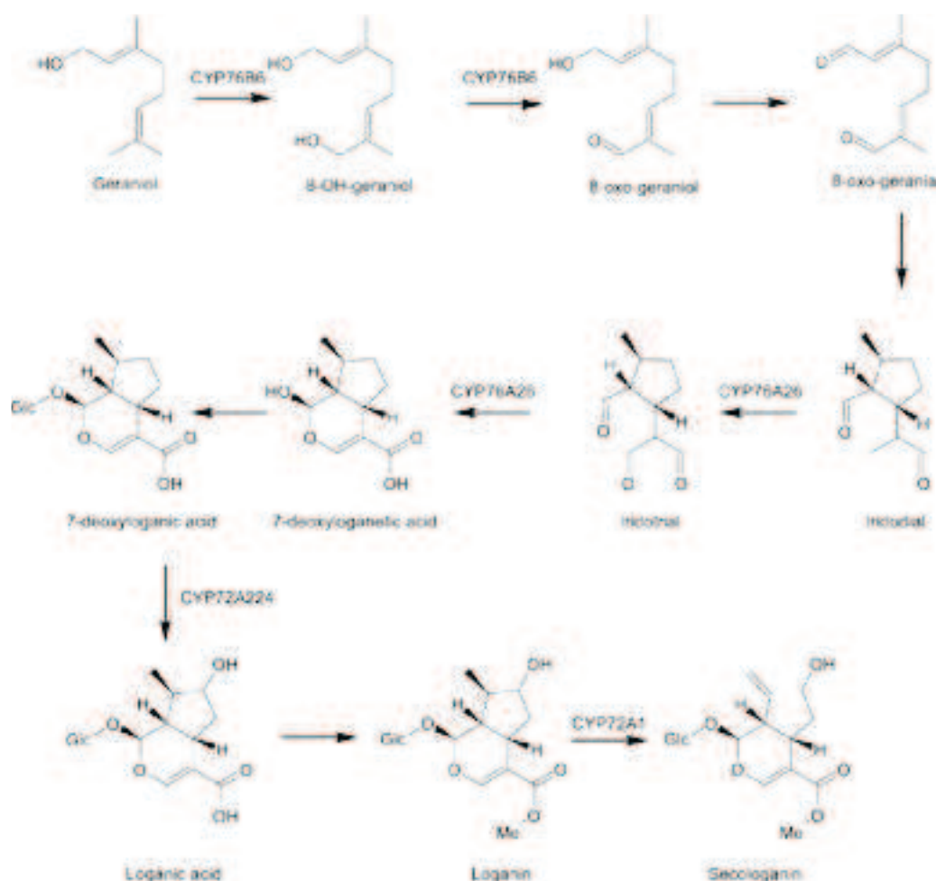
Figure 5. Cytochromes P450 involved in secologanin pathway in Catharanthus roseus . Glc: (β-D)-glucopyranosyl moiety.
