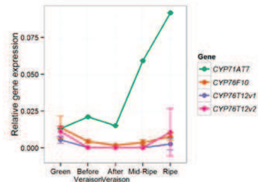
Figure 42. Relative expression of CYP76F10 and CYP76T12 during berry development. Error bars represent standard deviation of three technical and three biological replicates. CYP71AT7 is added for comparison of relative gene expression levels to genes discussed in the previous chapter.
