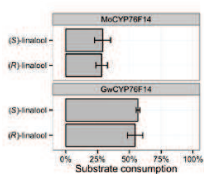
Figure S23. Conversion of two linalool enantiomers by CYP76F14 expressed in yeast. (Mo= Muscat Ottonel and Gw = Gewurztraminer). Sample preparation is identical to those used to generate data in Figure 4. Conversion ( \pm SD, N=3) is calculated relative to the residual concentration of substrate in negative control (microsomal fraction from yeast transformed with an empty vector - EV) incubated under the same conditions. Student's t-test showed no significant difference between the two substrates at \alpha=0.05 for neither of the enzyme variants.
