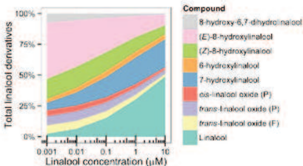
Figure 15. Estimated flux of linalool to different oxygenated derivatives. Relationship between log concentrations of each linalool derivative and linalool was described with a linear regression. These models were then used to estimate the concentration of each derivative in the function of linalool concentration. ( cis )-linalool oxide (F) and hotrienol were excluded from the figure because of low R^2 value (Table S3).
