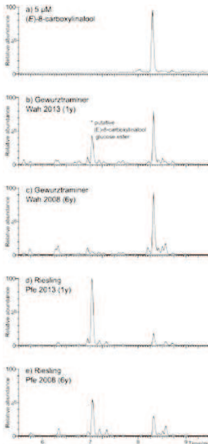
Figure S7. LC-MS/MS detection of (E)-8-carboxylinalool and its glucose ester in wines. Specific MS/MS transition was used for detection of (E)-8-carboxylinalool (167.3 > 93 m/z). Peak at 7 min was putatively identified as (E)-8-carboxylinalool glucose ester on the basis of its mass spectrum (Table S3).
