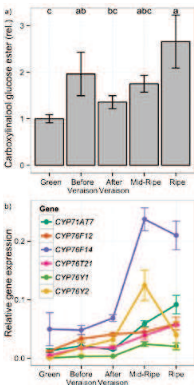
Figure 30. Comparative increase in (E)-8-carboxylinalool glucose ester content and candidate P450 genes expression during grape berry development. a) Relative concentration ( \pm SD) of (E)-8-carboxylinalool glucose ester in developing Gewurztraminer berries. One-way ANOVA revealed significant differences between developmental stages ( p=0.0016 ). Letters indicate significant differences among the means calculated with Tukey HSD test ( \alpha = 0.05 ). b) Expression of candidate genes in Gewurztraminer grape berries as determined by qPCR. Error bars represent standard deviation of 3 technical and 3 biological replicates. Gene expression was normalized to the expression of three constitutively expressed genes (30).
