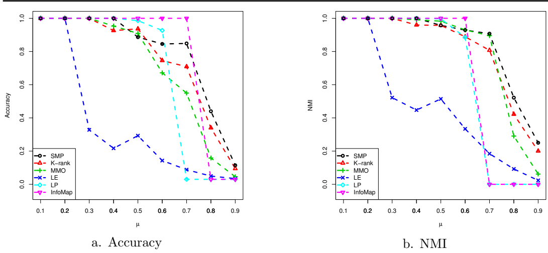
Figure 4.4: Comparison of SMP and other algorithms in LFR networks. The number of nodes is n = 2000 . The average degree is |k| = 30 , and the pair for the exponents is (\gamma, \beta) = (2, 1) .
