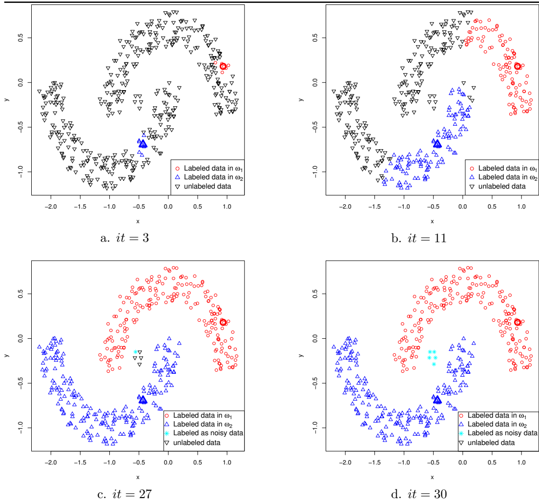
Figure 6.6: The label propagation process on two-moon data set. The initial labeled samples are marked with big size symbols in the figure.
