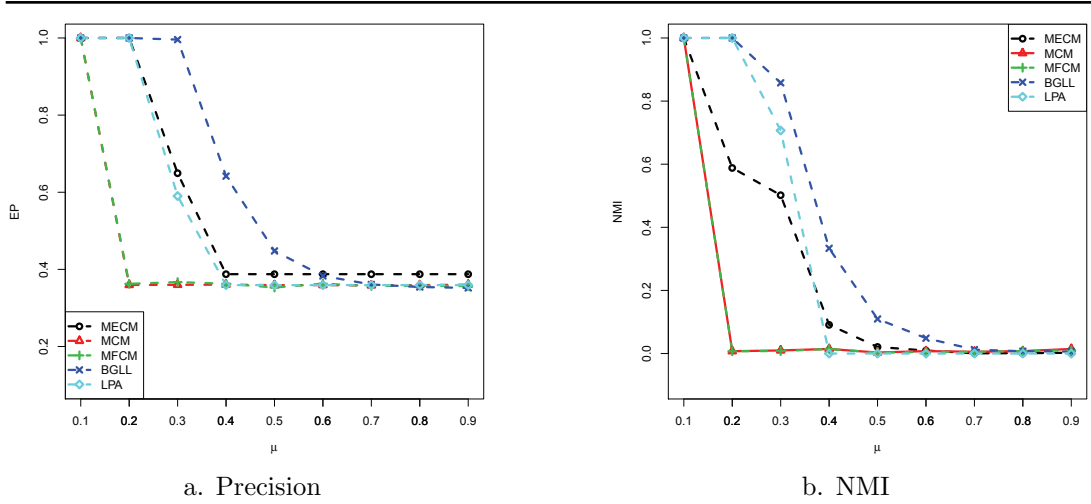
Figure 3.8: Comparison of MECM and other algorithms in LFR networks. The number of nodes is n = 500 . The average degree is |k| = 15 , and the pair for the exponents is (\gamma, \beta) = (2, 1) .
