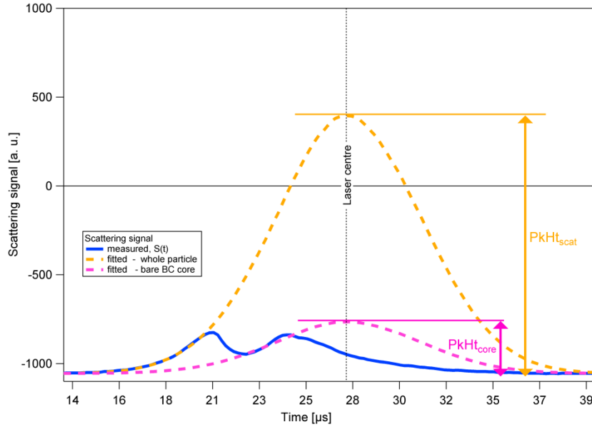
Figure 2.7. Example of reconstructed peak height for rBC-containing particle. Raw scattering signal in blue. Reconstructed scattering signal for the core-shell particle ( PkHt_{scat} ; dashed orange line) and the rBC core ( PkHt_{core} ; dashed pink line). The shape assumed for the Gaussian represent the shape of the laser and the maximum is kept at the centre of the laser beam while the Gaussian is scaled up and down until the signal is fitted up to the point of coating evaporation. All properties are expressed in arbitrary unit [a. u.]. Source: Laborde et al, (2012b))
