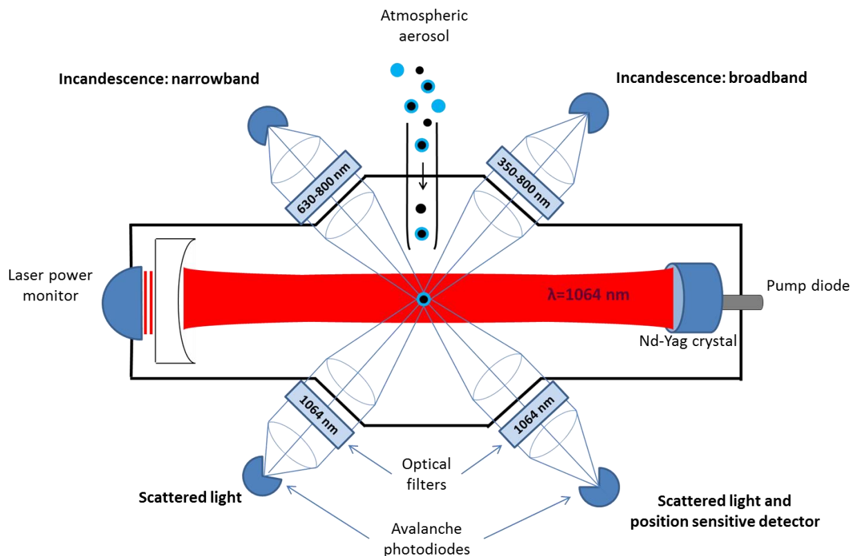
Figure 2.4. Schematic of the measurement chamber of the SP2.
