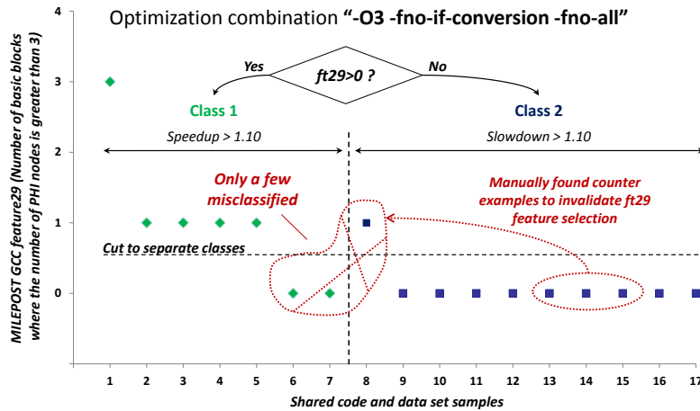
Figure 6.4 – Automatic detection of the relevant feature(s) to predict optimization cluster “-O3 -fno-if-conversion -fno-ALL” using complexity reduction. However, we manually converted several code samples to provide counter examples that invalidated this feature and showed that using small training sets in many current studies can be totally misleading.
