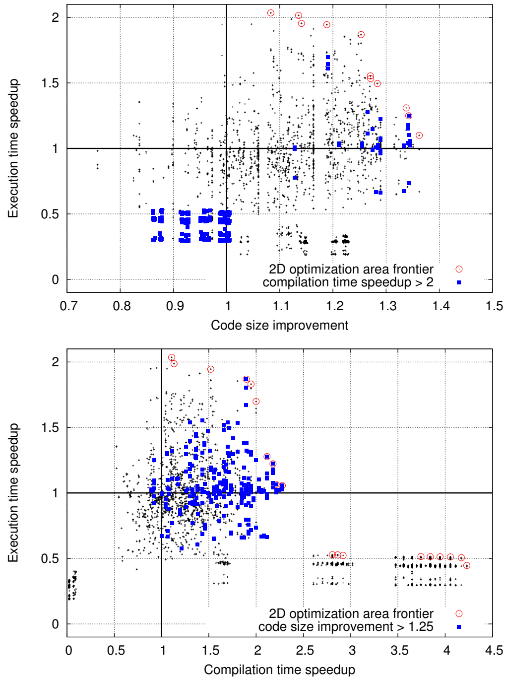
Figure 3.4 – Distribution of execution time speedups, code size improvements and compilation time speedups for benchmarks susan_c on AMD platform during iterative compilation. Depending on optimization scenarios, good optimization cases are depicted with circles on 2D optimization area frontier and with squares where third metric is more than some threshold (compilation time speedup > 2 or code size improvement > 1.2 ).
