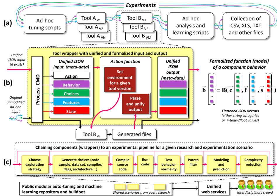
Figure 5.2 – (a) Conceptually depicted current ad-hoc experimentation; (b) wrappers developed by the community around existing tools to gradually expose behavior (characteristics), choices, features and system state using unified JSON input and output format; (c) wrappers and modules chained together as LEGO to implement various experimentation scenarios within a public buildbot that can be collaboratively explored and improved by the community.
