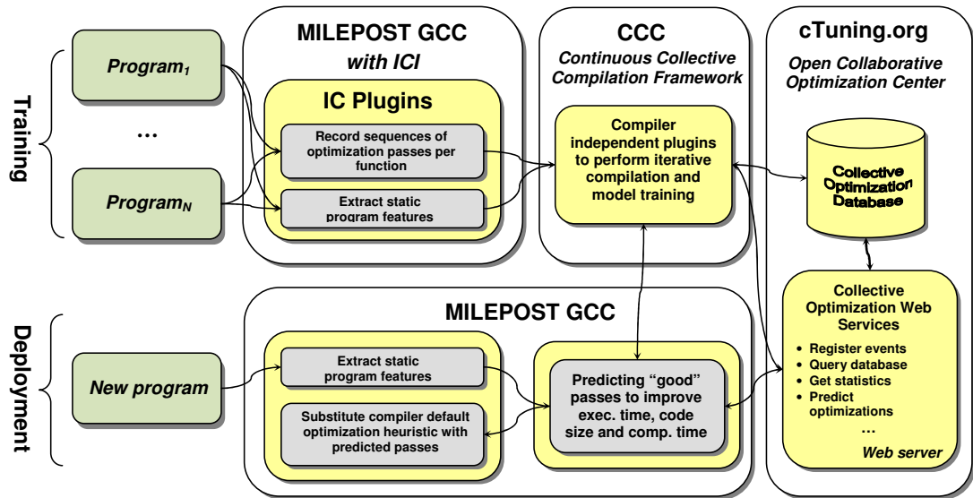
Figure 4.1 – Open framework to automatically tune programs and improve default optimization heuristics using predictive machine learning techniques, Milepost GCC with Interactive Compilation Interface (ICI) and program features extractor, CCC Framework to train ML model and predict good optimization passes, and COD optimization repository at cTuning.org.
