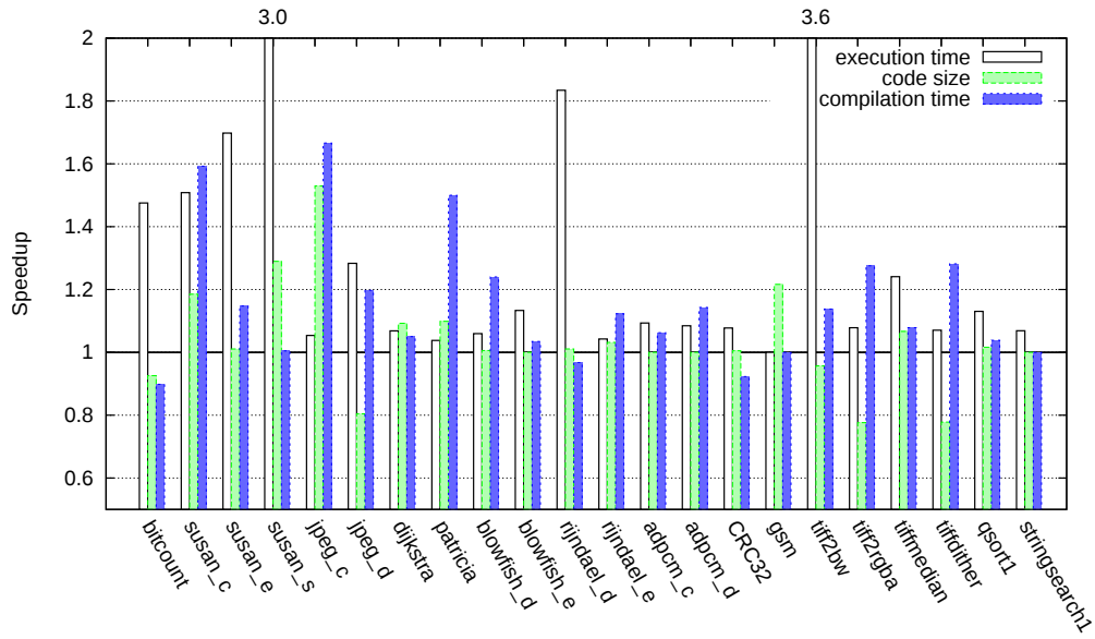
Figure 3.5 – Code size improvements and compilation time speedups for optimization cases with execution time speedups within 95% of the maximum available on Intel platform (as found by iterative compilation).
