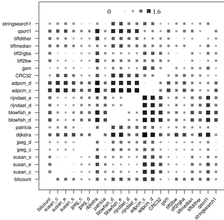
Figure 4.4 – Euclidean distance for all programs based on static program features normalized by feature 24 (number of instructions in a method).
