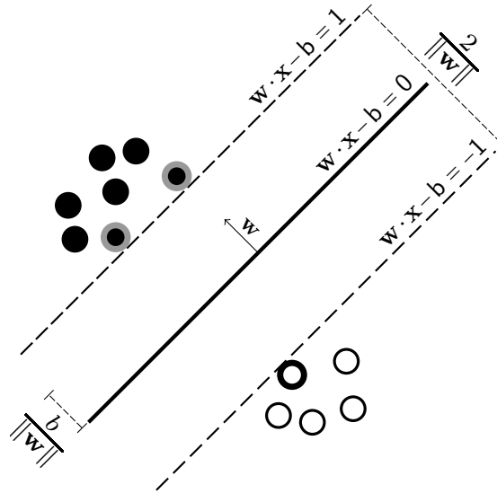
Figure 2.7 – Data points separated by two maximum-margin hyperplanes in a two-class SVM problem
