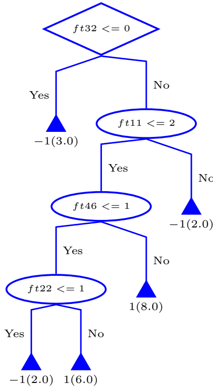
Figure 2.5 – Decision tree of -falign-functions optimization
