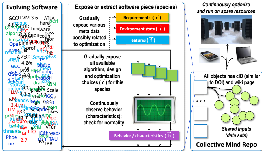
Figure 5.1 – Collective Mind Framework and Repository (cM) help to decompose any complex software into pieces with light-weight wrappers that expose design and optimization choices, measured characteristics, features and environment state in a unified and mathematical way(using vectors). It was developed to unify and systematize software autotuning, make it practical and reproducible, and distribute it among numerous computing resources such as mobile phones and data centers shared by volunteers [59, 100].
