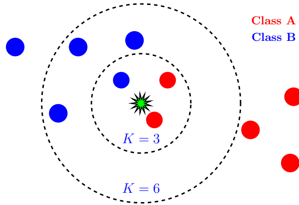
Figure 2.6 – Classification with KNN algorithm
