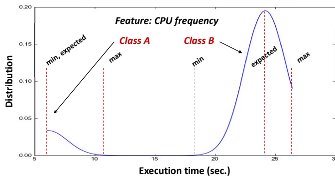
Figure 6.6 – Unexpected behavior helped to identify and share missing feature.
