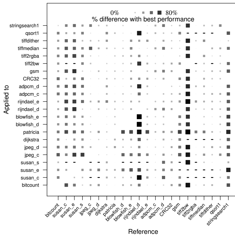
Figure 4.3 – % difference between speedup achievable after iterative compilation for “applied to” program and speedup obtained when applying best optimization from “reference” program to “applied to” program on AMD. “-” means that best optimization was not found for this program.
