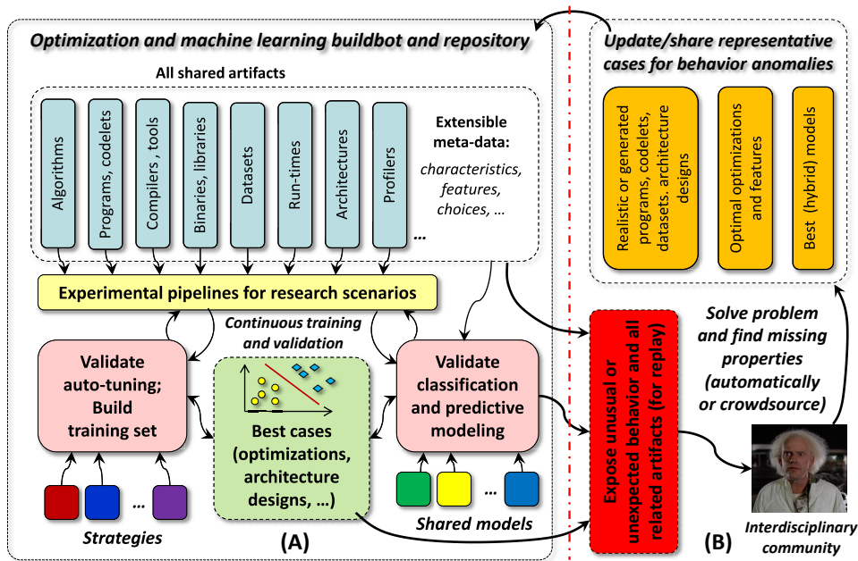
Figure 6.1 – Summary of the presented cooperative approach and practical buildbot to collaboratively and semi-automatically learn and improve behavior of computer systems using complete public experimental pipelines including code and dataset samples, tools, models, features and all other associated artifacts shared, analyzed and improved by the interdisciplinary community.
