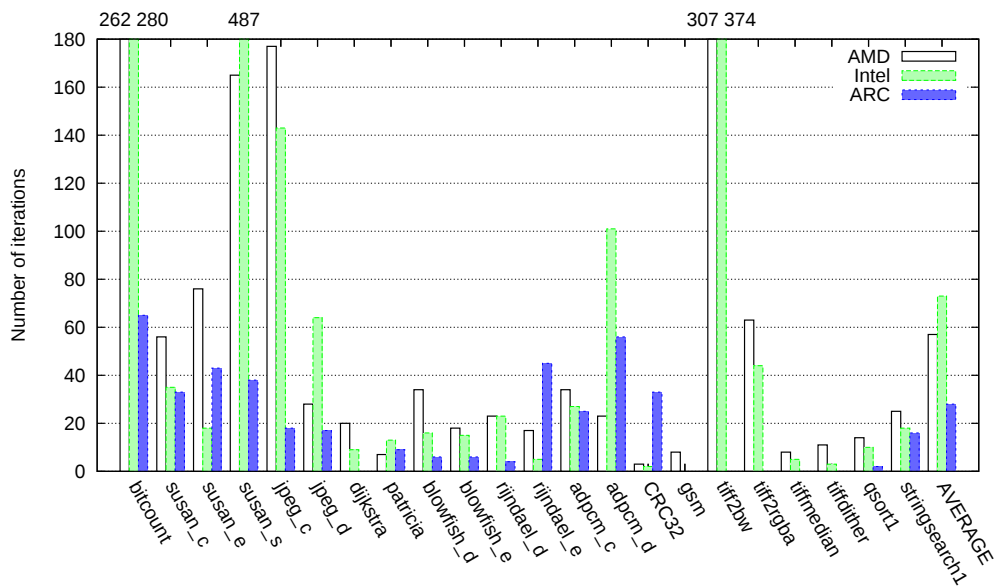
Figure 3.6 – Number of iterations needed to obtain 95% of the available speedup using iterative compilation with uniform random distribution.
