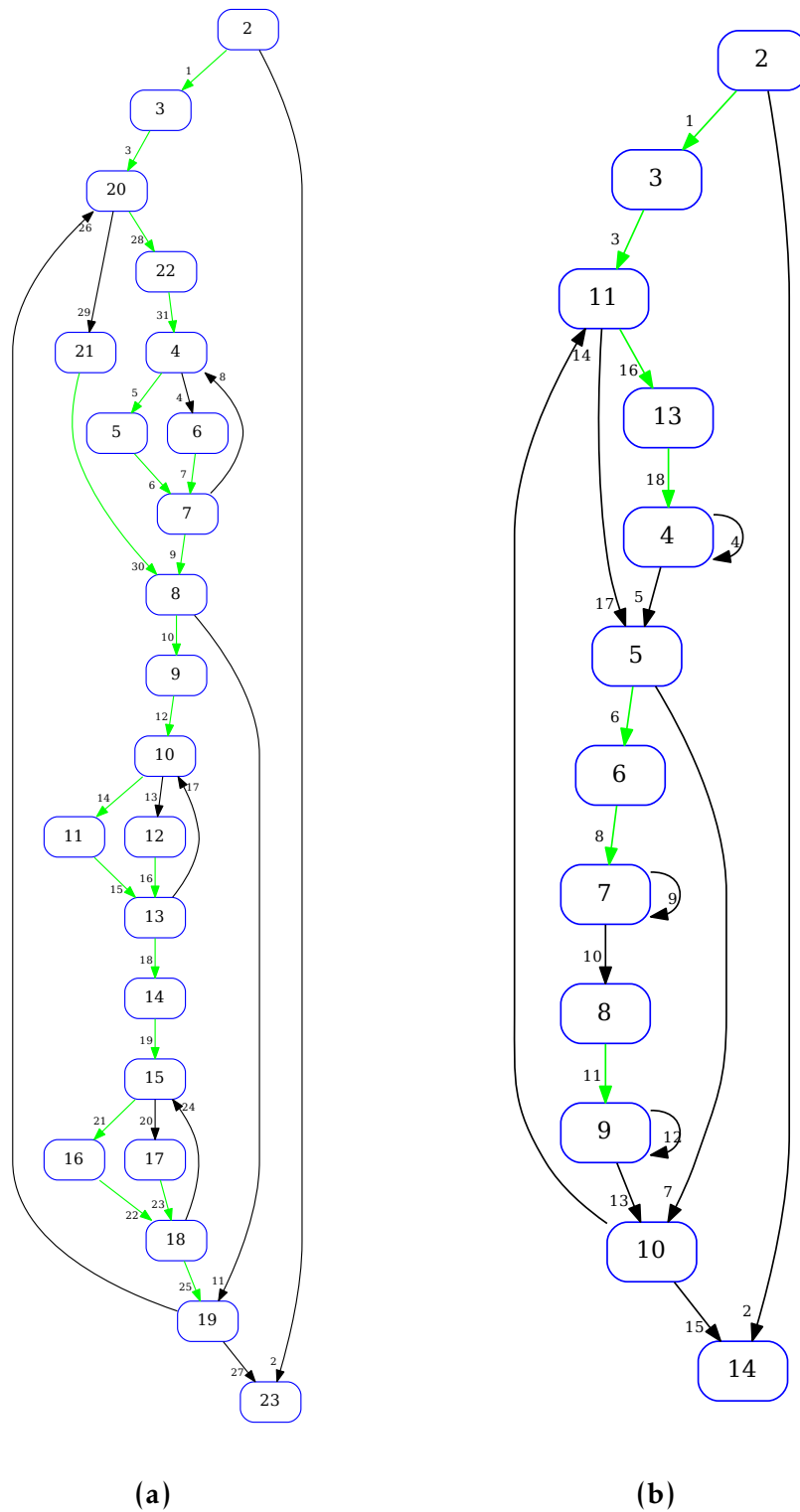
Figure 2.2 – Control flow graph of mc.codelet-9.1 constructed using a) gcc-4.6.3 -O3 b) gcc-4.6.3 -O3 -fno-ifconversion
