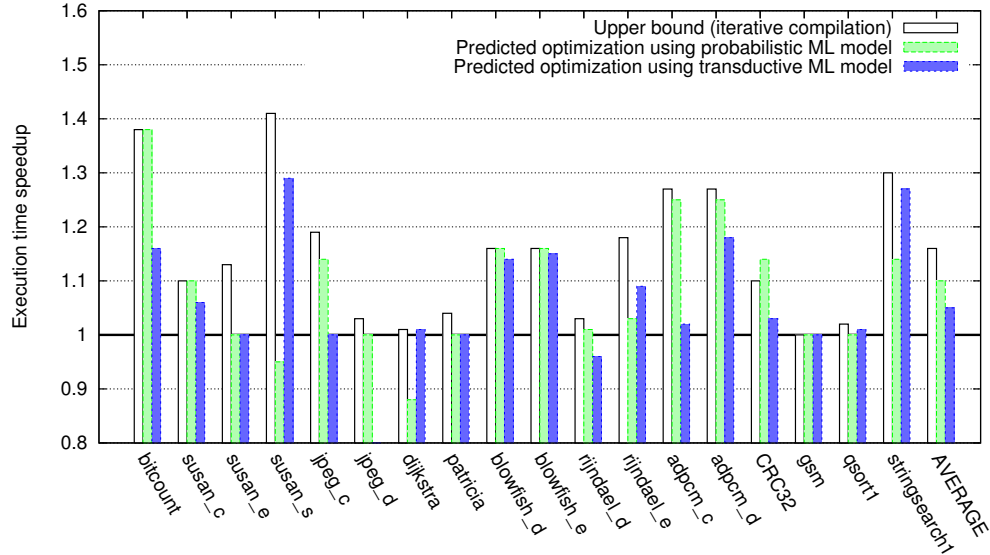
Figure 4.6 – Speedups achieved when using iterative compilation on ARC with random search strategy (1000 iterations; 50% probability to select each optimization;) and when predicting best optimizations using probabilistic ML model and transductive ML model based on program features
