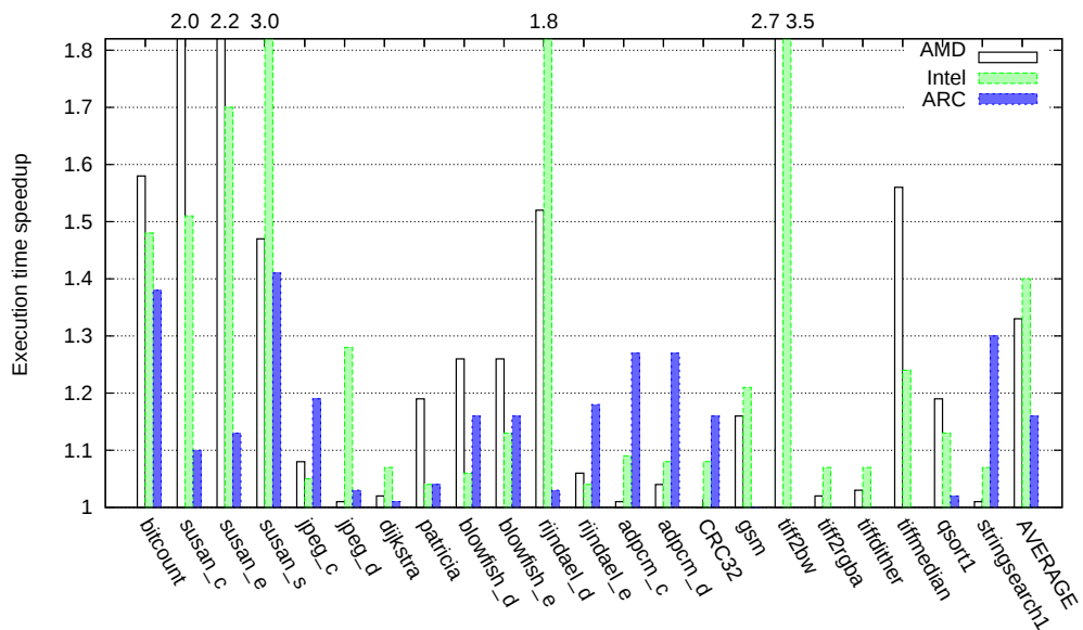
Figure 3.2 – Maximum execution time speedups over the highest GCC optimization level ( -O3 ) using iterative compilation with uniform random distribution after 1000 iterations on 3 selected architectures.
