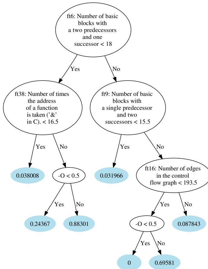
Figure 4.7 – Top levels of decision trees learnt for ARC.
