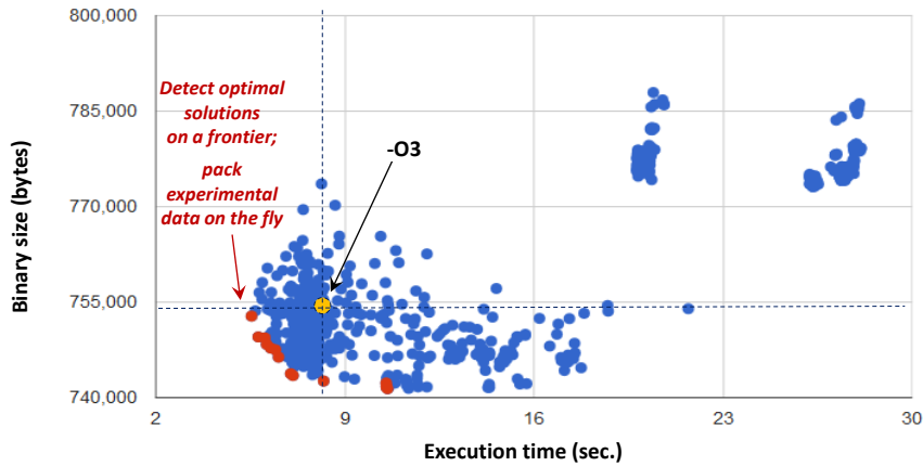
Figure 6.2 – Variation in execution time vs code size when crowdsourcing optimization of an image corner detection application with a fixed dataset on Samsung Galaxy Series mobile phone with ARMv6 830MHz processor when randomly selecting compiler flags for Sourcery GCC 4.7.2. Yellow point represents -O3 and red circles show Pareto frontier. This data will be available for validation at the conference.
