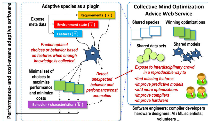
Figure 6.7 – Concept of performance- and cost-aware self-tuning software assembled from cM plugins.
