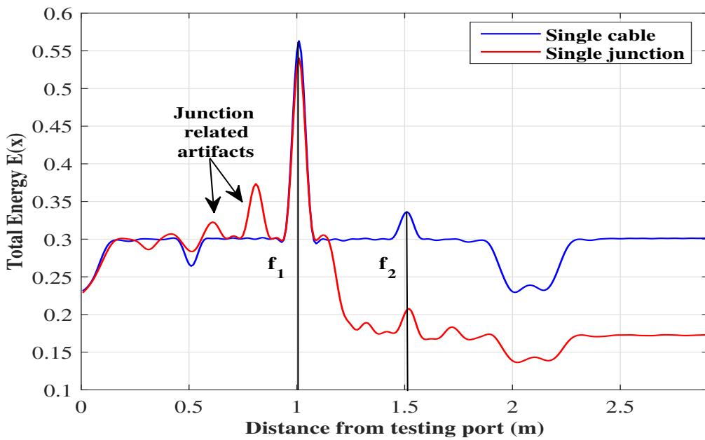
Figure 4.13 The total energy E(x) obtained for the description comparing the responses of weak faults with respect to the network's complexity between the single-branch configuration of Fig. 4.10 (a) and the single-junction NUT of Fig. 4.10 (b) along its second path, while considering two soft faults at the same distances with respect to the reference port (1 m for the first soft fault and 1.5 m for the weaker one).
