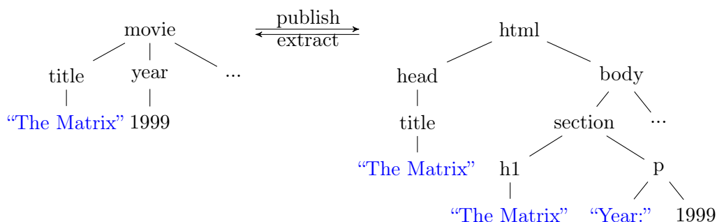
Figure 1.7: Web production that creates some data equality constraint in its output.
