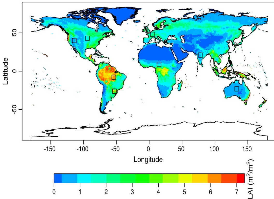
Fig. 4 - 3 Global map of the long term mean LAI in \text{m}^2\cdot\text{m}^{-2} (Dirmeyer et al., 2006).
