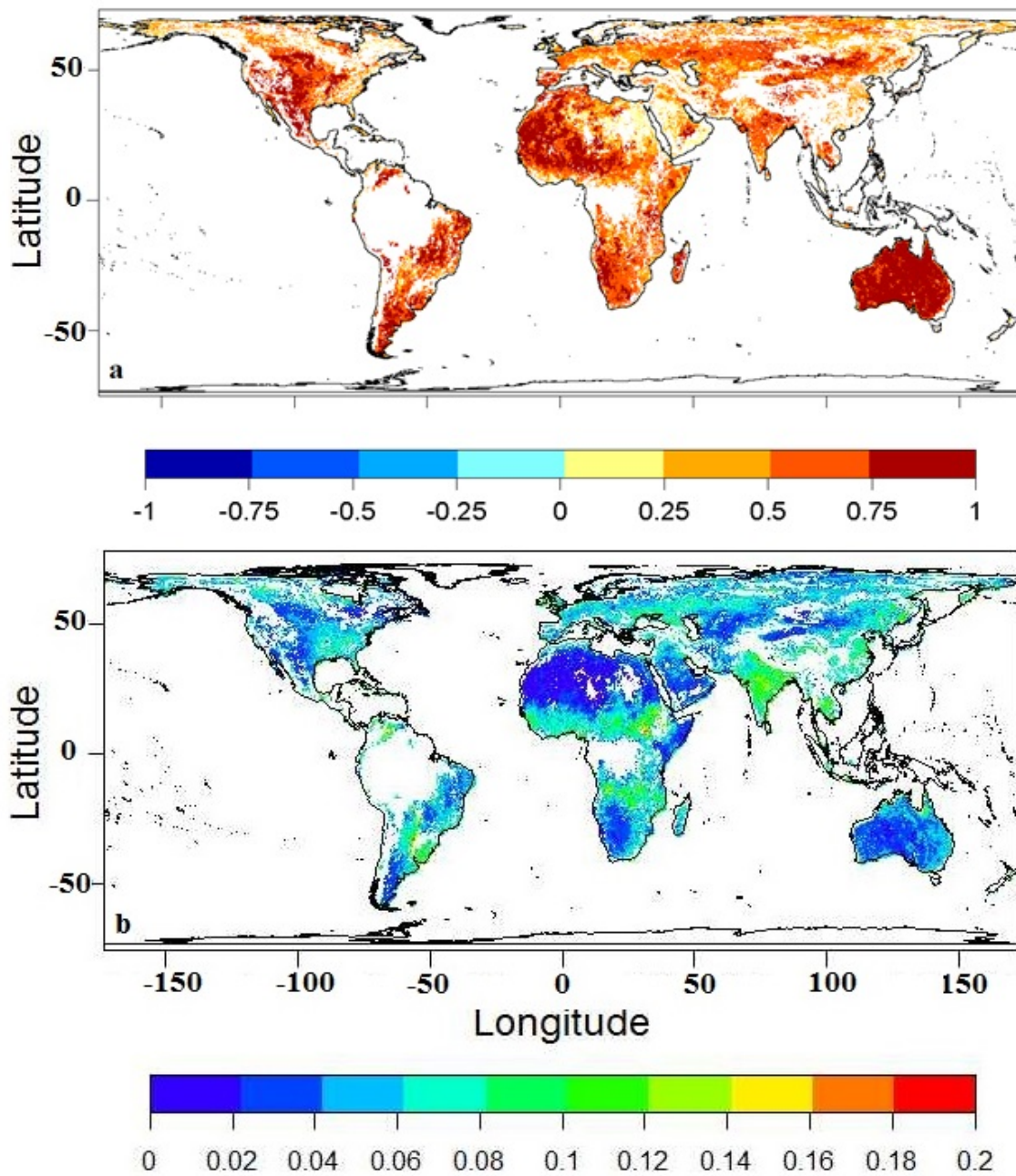
Fig. 6 - 4 Regression statistics of AMSR-reg vs. SMOSL3 SSM in 2010-2011 with Eq. (6.1): a) R (a) and b) RMSD ( \text{m}^3/\text{m}^3 ) (b). White areas over land indicate areas with dense vegetation, strong topography, and wetlands.
