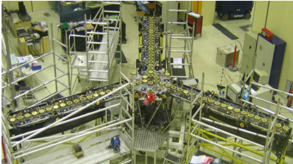
Fig. 3 - 2 MIRAS instrument configuration diagram (upper panel) and during its assembly and integration (bottom panel) (McMullan et al., 2008).
