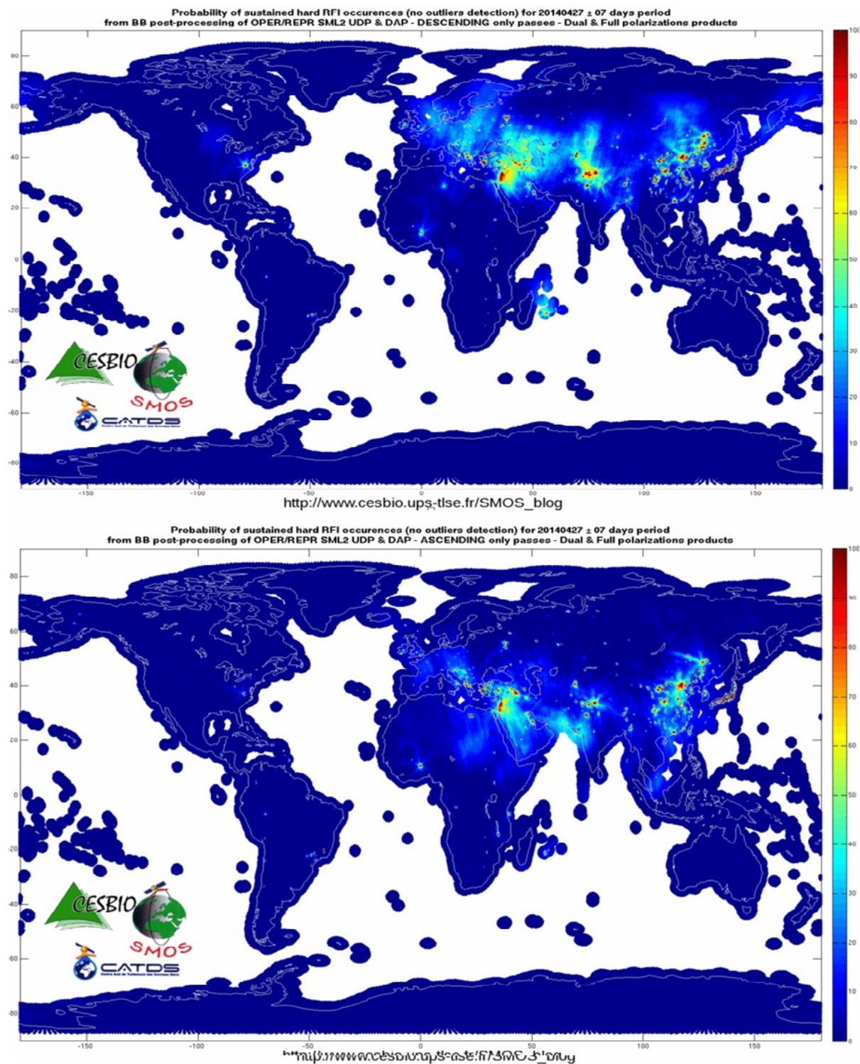
Fig. 3 - 7 probability of RFI occurrences for 20140427 ascending (bottom) and descending (top). Source: [ http://www.cesbio.upsc-tlse.fr/SMOS_blog/ ].
