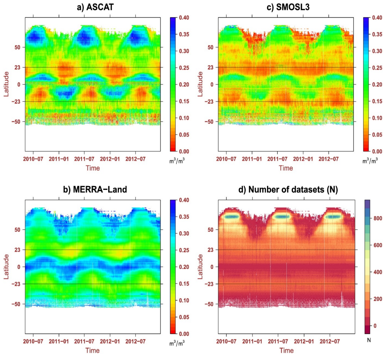
Fig. 5 - 7 Time–latitude variations of original surface soil moisture data ( \text{m}^3/\text{m}^3 ) for (a) ASCAT, (b) MERRA-L, (c) SMOSL3 and (d) number of data illustrated in Hovmöller diagrams.
