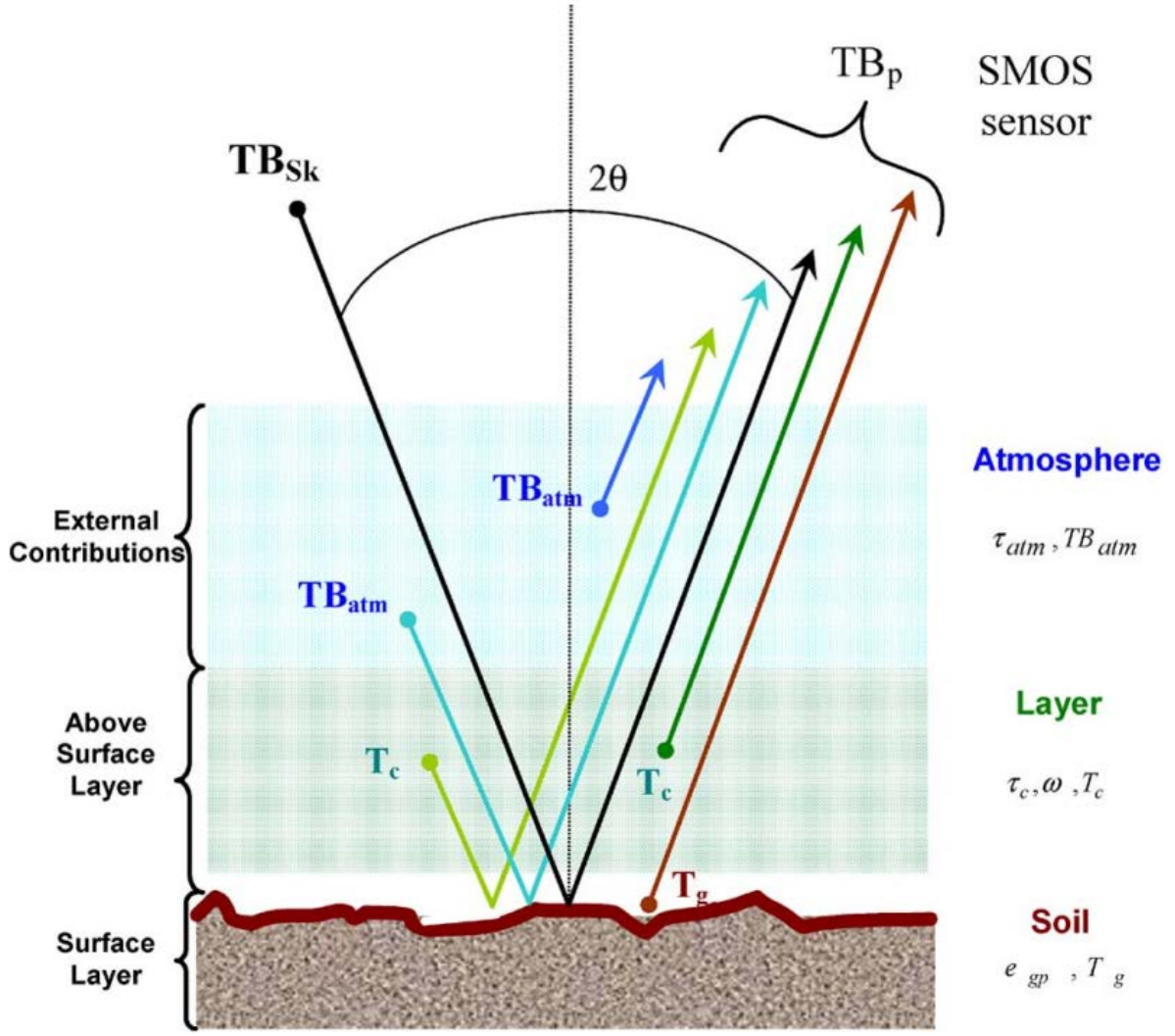
Fig. 3 - 5 Components of the general radiative transfer equation ( Kerr et al., 2012 ).
