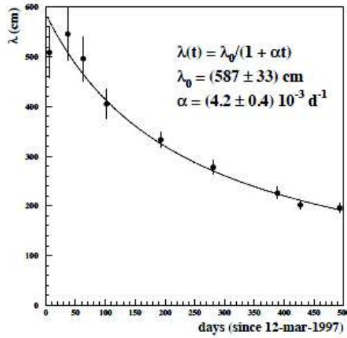
Figure 77: Evolution with elapsed days of the attenuation length \lambda measured by the CHOOZ collaboration in Ref. [107].
