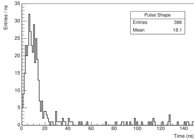
Figure 39: Example of a PS reconstructed in Double Chooz for a single event of 4.74 MeV.
