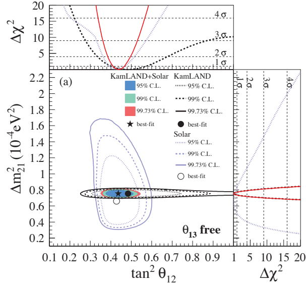
Figure 8: C.L. regions in the (\tan^2 \theta_{12}, \Delta m_{12}^2) space of results from KamLAND [93] and solar experiments.
