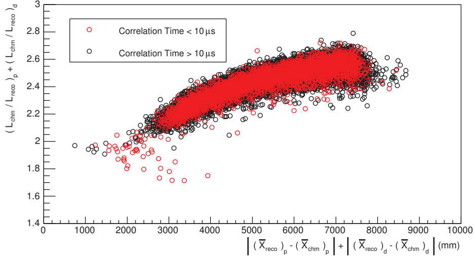
Figure 50: Chili plot, or sum of the prompt and the delayed ratio between L_{chm} and L_{reco} , as a function of the sum of the prompt and the delayed vertices distance from the chimney |(\bar{X}_{reco})_p - (\bar{X}_{chm})_p| + |(\bar{X}_{reco})_d - (\bar{X}_{chm})_d| , for neutrino candidates of the DC-III (n-Gd) selection. Events with short prompt-delayed \Delta t are featured in red.
