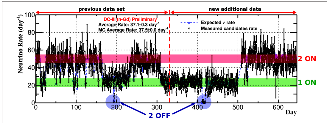
Figure 32: Selected number of neutrino candidates day by day.
