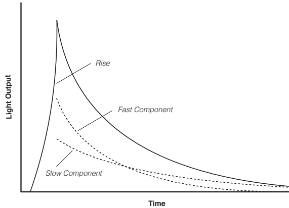
Figure 36: Graphic representation of the light time profile, as a result of the combination of the excitation and the two-component de-excitation of molecular states of a liquid scintillator.
