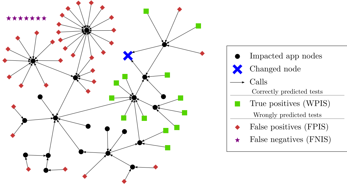
Figure 3.1: Visualization of the effect of a particular mutation. Black circles are the nodes that propagate the mutation injected in the node denoted with a blue cross. Nodes illustrated by green boxes, red diamonds and purple stars are test cases related to the injected mutation. Green boxes nodes are test cases that are correctly predicted as impacted by the injected mutation; these are true positives. Red diamonds nodes are test cases that are predicted as impacted, but are not; these are false positives. Purple stars nodes are test cases that should have been predicted as being impacted but have not been; these are false negatives.
