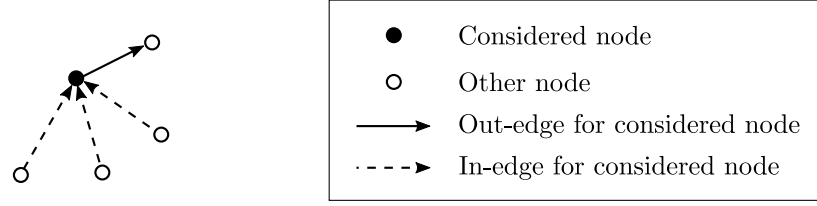
Figure 2.4: In-edges and out-edges for a simple digraph example.
