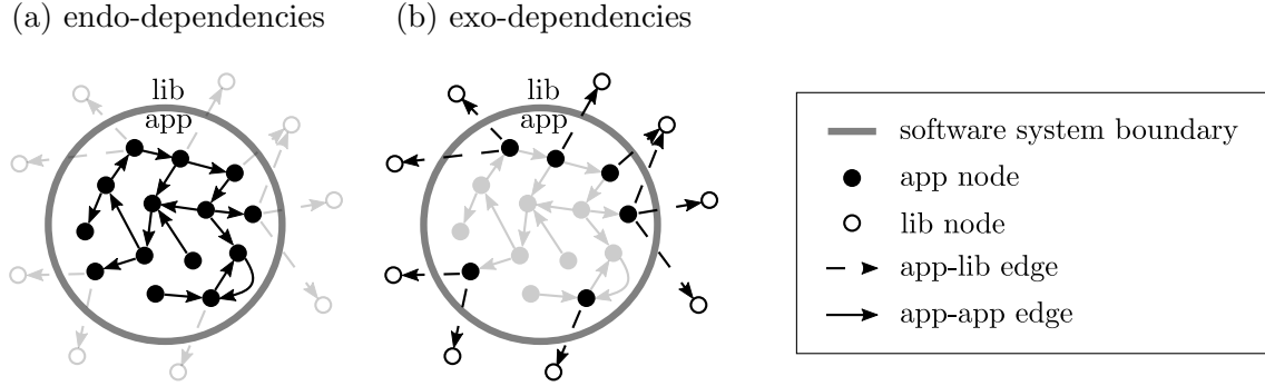
Figure 2.8: Illustration of the set of (a) endo-dependencies and (b) exo-dependencies in a dependency graph.
