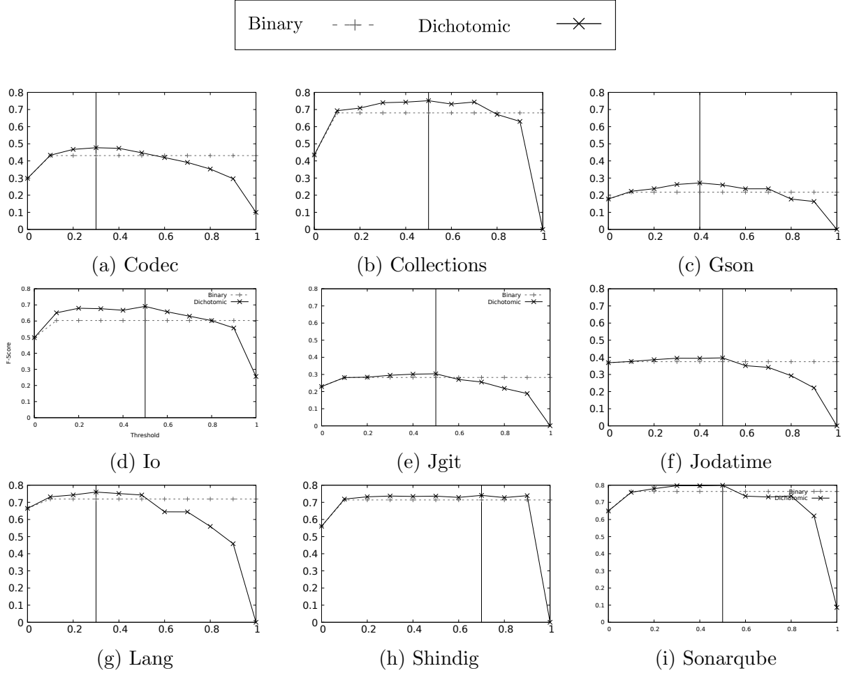
Figure 4.4: The impact of the prediction threshold (x-axis) on the F -score (y-axis). Low ( < 0.1 ) and high ( > 0.5 ) thresholds yield bad performances, the rest forms a plateau – Binary is a dashed line and Dichotomic is a plain one.
