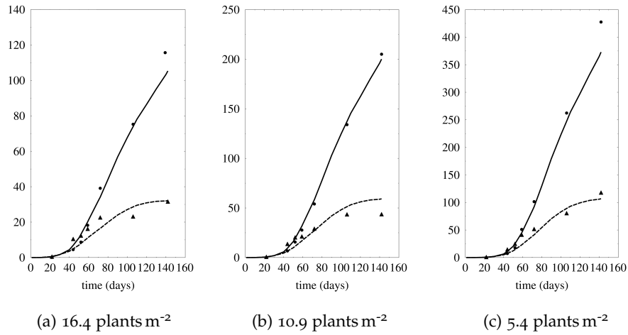
Figure 9.: Comparison of simulations using the parameters listed in table 1 to experimental data on A_{\sqrt{}}(t) (solid line, bullets) and A_{\spadesuit}(t) (dashed line, triangles) [g], per plant, for three different field densities.
