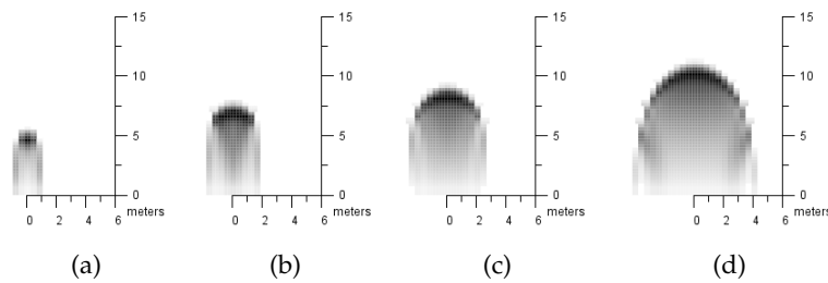
Figure 13.: Qualitative leaf density dynamics of a simulated tree in competition with neighbours at (a) 25, (b) 60, (c) 90 and (d) 140 years. Time-dependent stand density, defining the boundary region (cf. section 3.4.1 for details), corresponds to the one shown in figure 15, sub-plot 3 (cf. also section 6.2.1).
