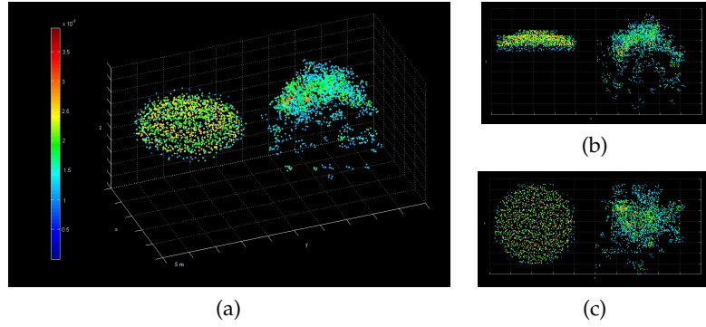
Figure 21.: (a) Oblique, (b) side and (c) top view of mean empirical (right) and simulated (left) relative twig- and leaf area density, \bar{\mathbf{a}} and \frac{\clubsuit}{\int \frac{\clubsuit}{\clubsuit}} , respectively. The figures also illustrate the agreement of real and simulated height (figure 16c, top right) and crown radius (figure 17 right). See text for quantitative comparison.
