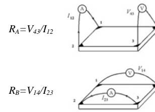
Figure 4: Schematic of the van der Pauw configuration
