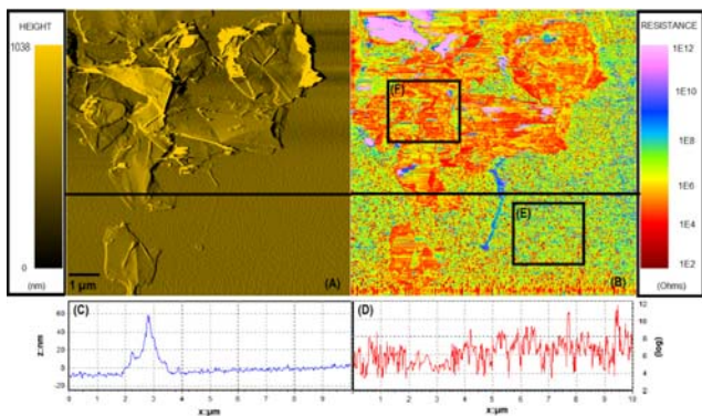
Fig. 5. (A) Topographic and (B) electric images of flakes exfoliated from suspension 8. PtIr tip, 50nN. (C) and (D) are profiles extracted from the image along the black horizontal line.
