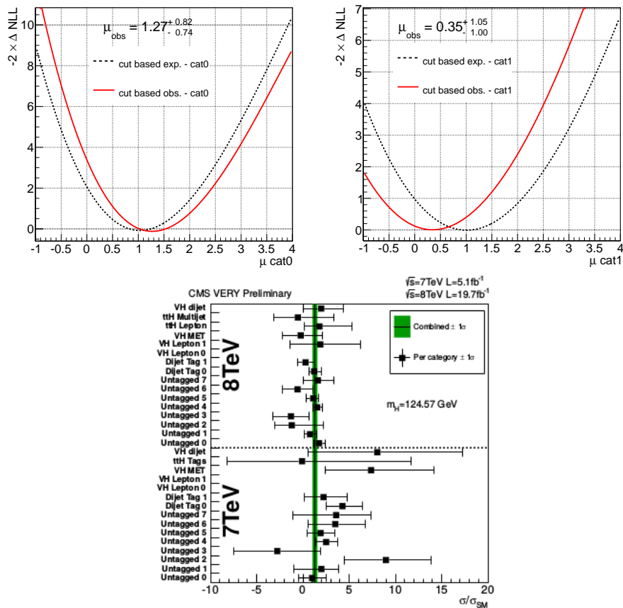
Figure 5.21: Likelihood scan as a function of \mu for our analysis (top plots), where the cut-based selection of Reference [13, 82] has been applied, for the tight category on the left and for the loose category on the right. The black line represents the expected \mu and the red line the observed one. The plot at the bottom shows the results of Reference [13, 82] at 8 TeV for the different categories. The results for the 2 Dijet Tag categories are similar to what we obtain.
