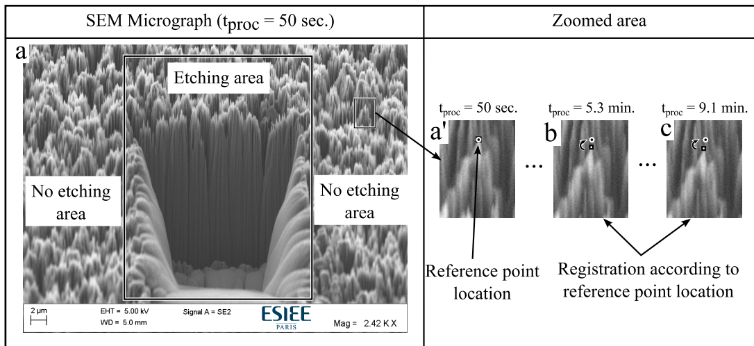
Figure 2.6. SEM micrographs registration for sample movement during FIB nanotomography. (a) SEM micrograph at t_{proc} = 50 seconds showing the etching and no-etching areas, (a') zoomed area of SEM micrograph at t_{proc} = 50 seconds where a peak is used as a reference point location, (b) and (c) corresponds to SEM micrographs (at t_{proc} = 5.3 minutes and t_{proc} = 9.1 minutes respectively) showing the peak displacement from the reference point location.
