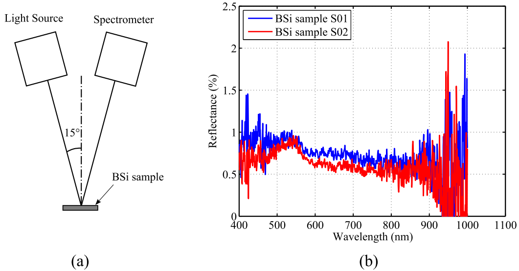
Figure 3.4. Specular reflectance measurements of BSi samples S01 and S02 by ellipsometry with angle on incidence of 15^\circ .
