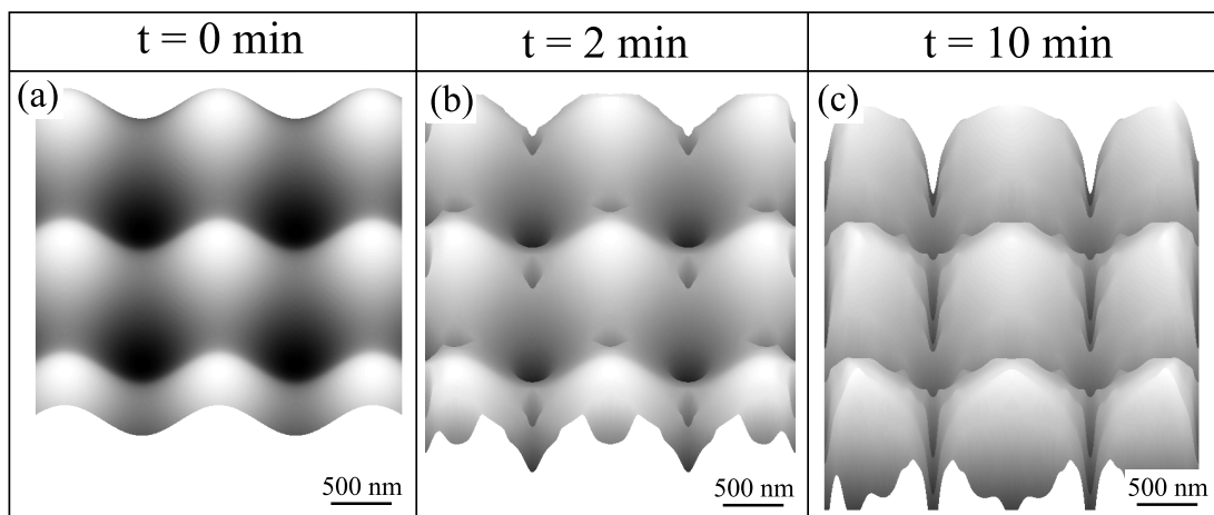
Figure 4.12. Formation of new etch fronts on saddle points on mathematically generated surface. (a) t = 0 \text{ min} , (b) t = 2 \text{ min} and (c) t = 10 \text{ min}
