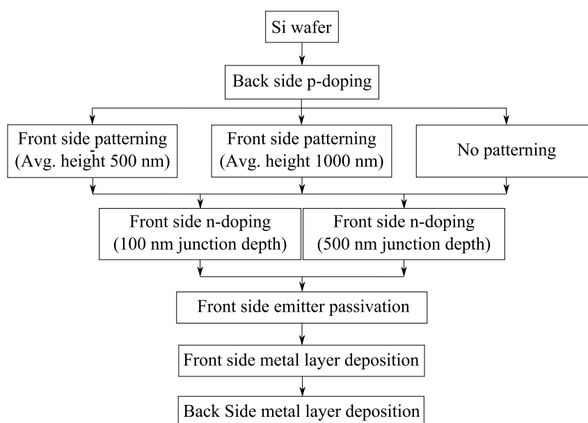
Figure 5.3. BSi solar cell fabrication process
