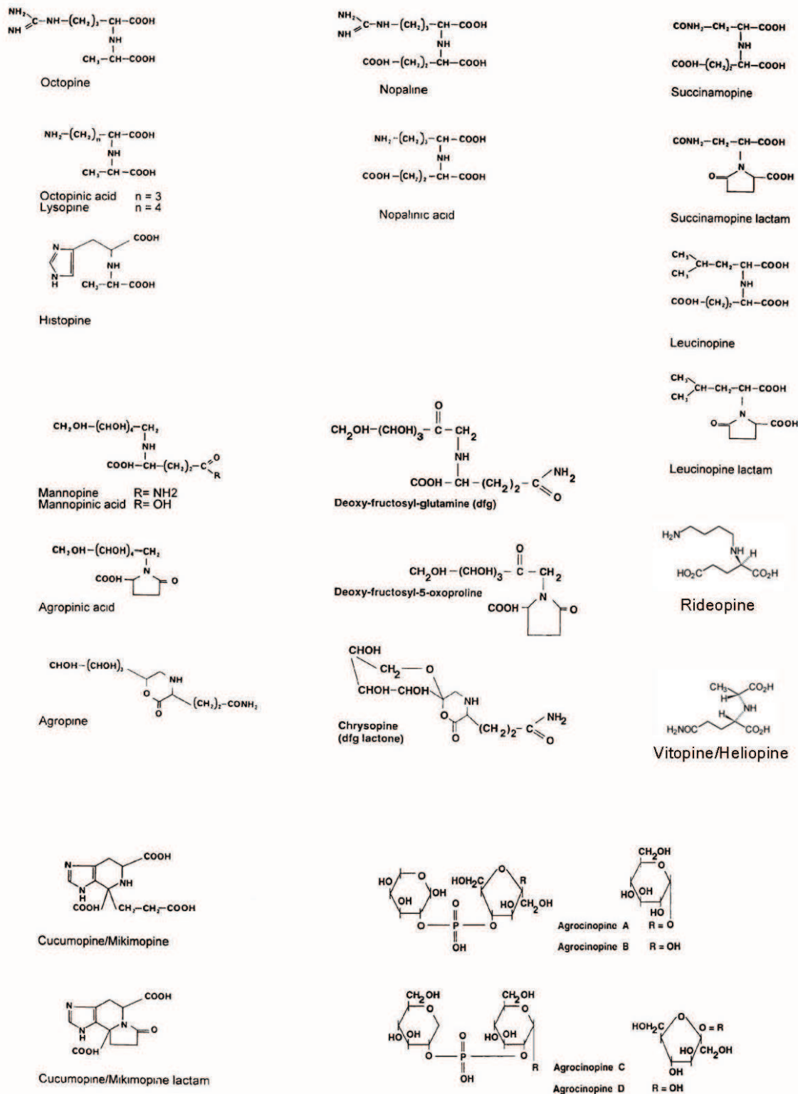
Figure 7. Chemical structures of opines produced by crown galls and hairy roots
