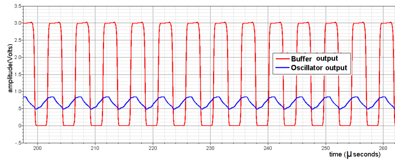
FIGURE 4.8 – Oscillateur csi (sans modification).
