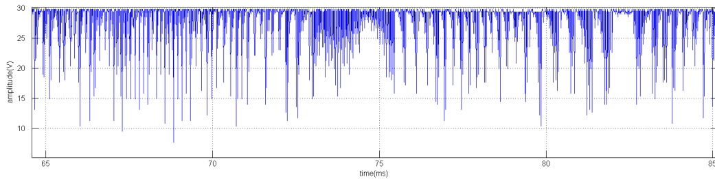
FIGURE 5.21 – Sortie Chaotique apres recalibration.
