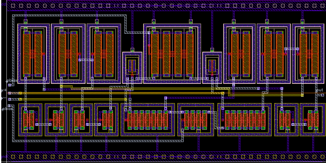
FIGURE 5.8 – Layout de la cellule OTA.
