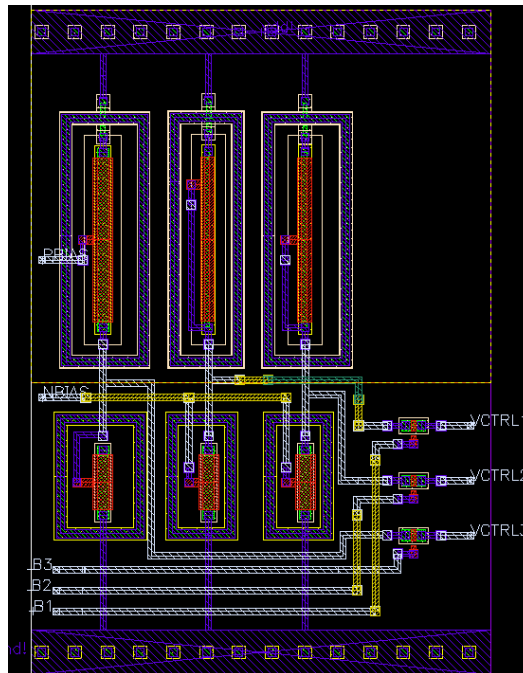
FIGURE 4.31 – layout du circuit de calibration.
