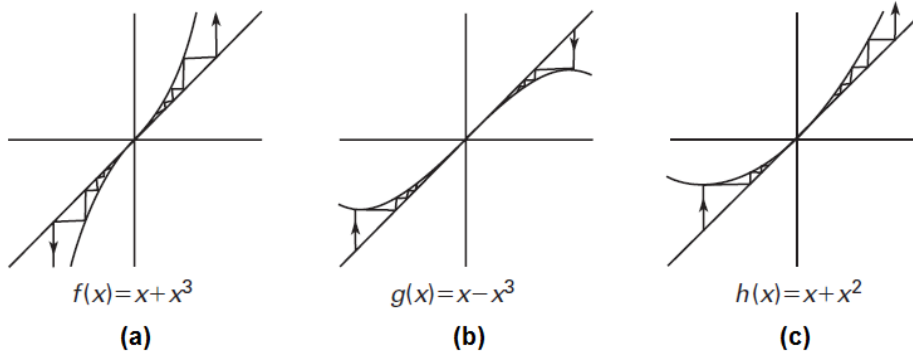
FIGURE 3.5 – Types de point fixe
