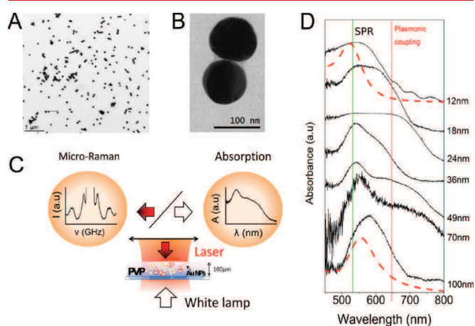
Figure 1. (A) TEM image of diluted gold 100 nm sample. (B) One hundred nanometer NP dimer showing d \approx 0.8 nm interparticle spacing. (C) Experimental setup allowing to measure both micro-absorption (transmission geometry, white lamp) and micro-Raman spectra (backscattering geometry, 532/647 nm laser lines) of gold NPs from a unique sample spot (laser spot \approx 0.6 \mu\text{m}^2 ). (D) From top to bottom, absorption spectra of samples with 12–100 nm diameter showing the dipolar resonance of isolated particles and the plasmonic coupling band. Red-dashed lines correspond to absorption spectra of 12 and 100 nm NPs in liquids before deposition. Green and red vertical lines correspond to the 532 and 647 nm excitation wavelengths used for Raman spectroscopy, respectively.
