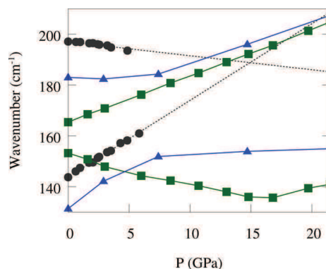
Figure 5. Variation of the E_g(1) and (2) optical phonon wavenumbers for bulk anatase \text{TiO}_2 as a function of pressure. The lines with green \blacksquare and those with blue \blacktriangle are for the first-principles calculations presented in this work and in ref 33, respectively. The black \bullet are measurements from ref 34. The black dotted lines are linear extrapolations of the experimental data.
