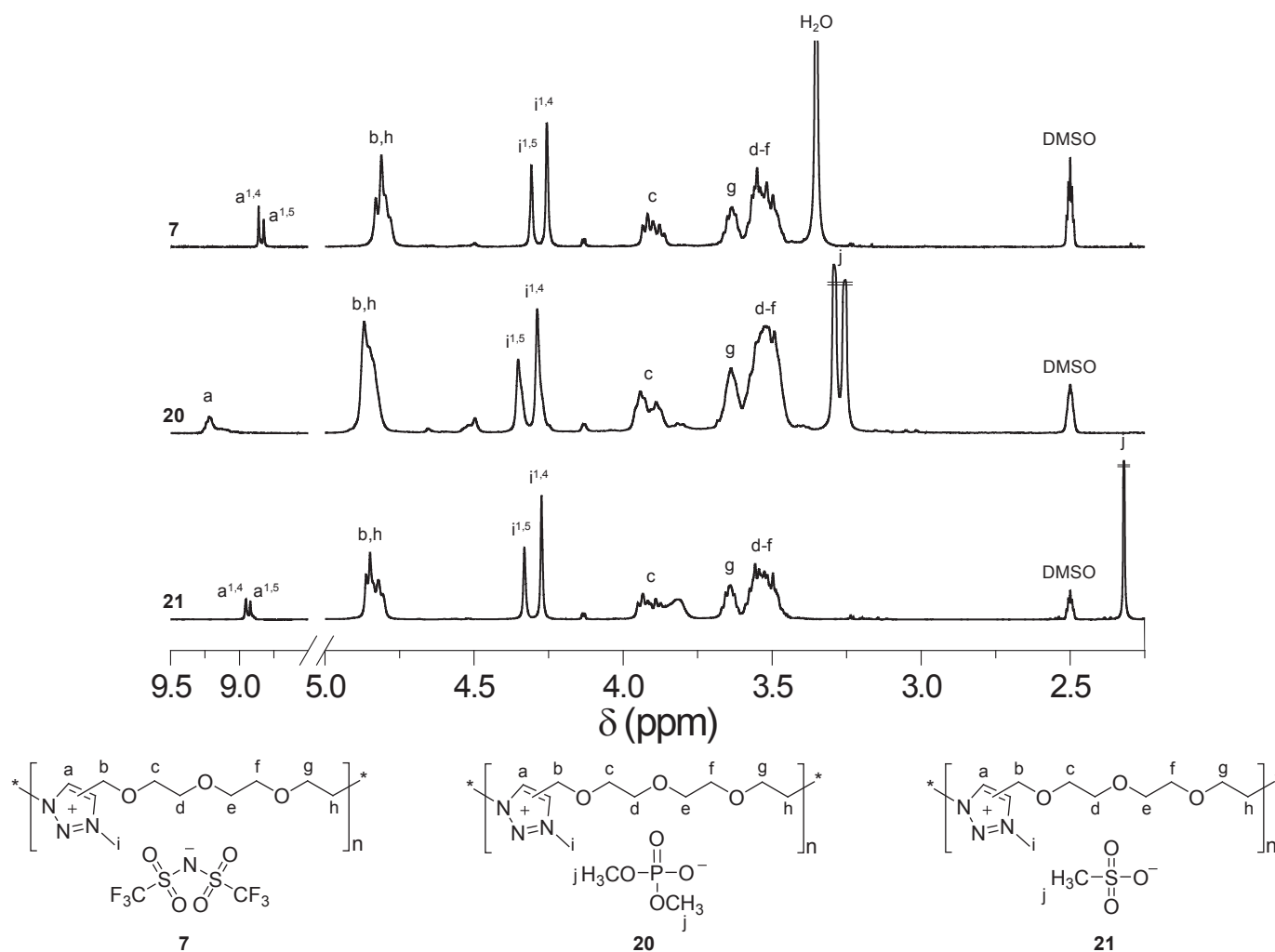
Figure III.12: Spectres RMN ^1\text{H} (25 °C, DMSO- d_6 ) des TPILs 7 , 20 et 21 .
