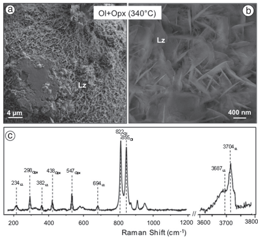
Fig. 2. SEM images and Raman spectra of reaction products at the end of experiments started with Ol + Opx (P9). (a) The SEM image shows small serpentine ca. ~1 µm in diameter grown on the surface of olivine and orthopyroxene and a zoom (b). (c) A typical Raman spectrum indicates that the degree of transformation of Ol + Opx into serpentine is quite low.
