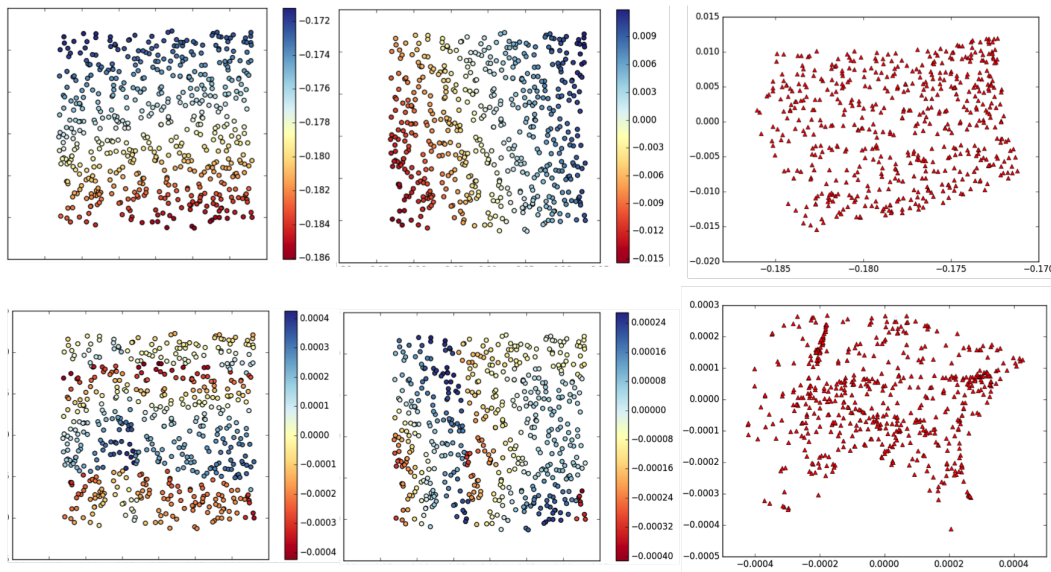
Figure VI.8 – Spatial distributions of the coefficients of the PSFs used for the experiments relative to 4 principal components calculated over the "learning" PSFs set; the top panel corresponds to the first and second principal components and the coefficients scatter plot; the bottom panel corresponds to the 6th and 7th principal components and the coefficients scatter plot as well.
