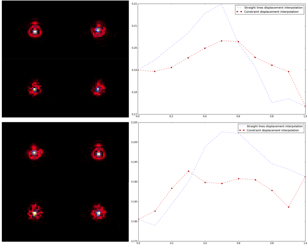
Figure VI.16 – Constrained displacement interpolation : the two PSFs panels show original PSFs on the top and the interpolated PSFs for t=0.5 are shown on the bottom left for the regular displacement interpolation and the bottom right for the velocity constrained displacement interpolation ; the right plots show the evolution of the l_2/l_1 norms ratio of interpolated PSFs as functions of the time parameter in the two examples respectively ; the velocity constraint reduces the shrinkage effect since the corresponding l_2/l_1 norms ratios are flattened compared to those obtained with the regular displacement interpolation ; moreover, the interpolated images are smoother.
