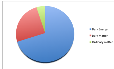
Figure I.1 – The Universe content.
