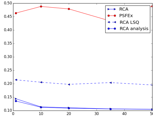
Figure V.10 – Average normalized least square error
