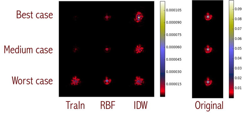
Figure VI.7 – Absolute error images for 15 neighbors ; from the left to the right, TraIn, RBF, IDW, original image ; from the top to the bottom, best, average and worst case in terms of the relative accuracy of TraIn with respect to the pixels mean square error.
