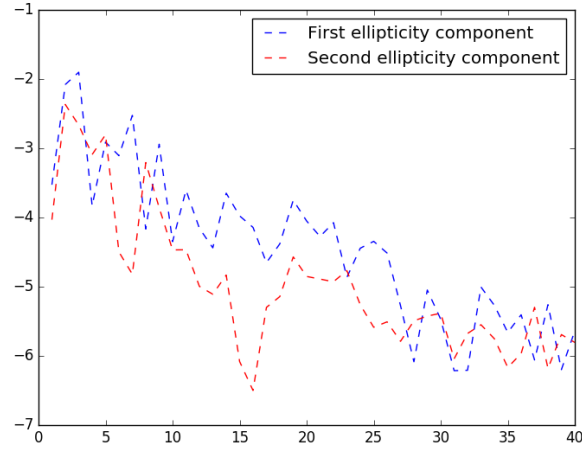
Figure VI.9 – Ellipticity components sensitivity to the PCA atoms. Y axis : \log_{10}(\mathcal{V}(e_k, \mathbf{P}_j)) (see Eq. VI.34) ; X axis : PCA atoms indexes j ; moderate errors on the PCA coefficients have a weak impact on the ellipticity, especially for the "high indexes" PCA components.
