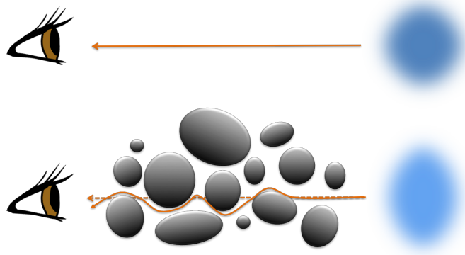
Figure I.2 – Weak gravitational lensing.
