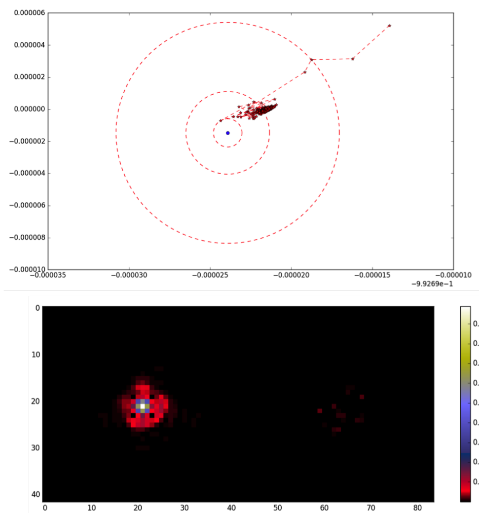
Figure VI.12 – Assignment failure : on the top plot, the sequence of images associated with each iterate are represented by the red dots and the image associated with the ideal solution is represented by the blue dot ; these images are shown in the plan spanned by the two first principal components calculated from the whole images set ; the iterates end up oscillating around a point in the middle circle ; the bottom left plot shows the ideal image and the bottom right plot shows the absolute difference between the final image and the ideal one ; one can see that there is some non-negligible artifacts.
