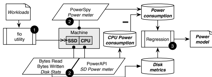
Figure 4.8: Empirical SSD power modeling approach.
