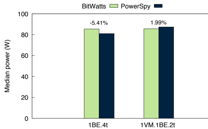
Figure 7.12: Median power consumption for SPECjbb on Intel i3 2120 servers for a distributed setup, virtualized and non-virtualized.
