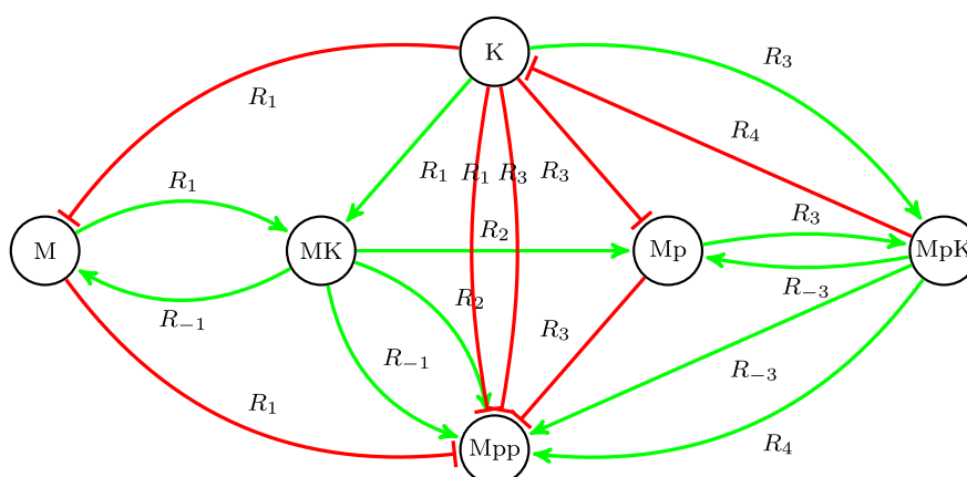
Fig. 8 Influence graph of Fig. 5, but with arcs ending in K and Mpp substituted, and then the only arc ending in K changed of sign. Resulting negative self-loops are, as usual, not shown, but note that the negative arcs from K to Mpp corresponds to the negative self-loops on K in the original graph. All positive circuits remaining can be ruled out by one of our corollaries as being a possible source of multistationarity
