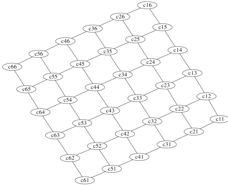
Fig. 4. Delta-Notch square cell grid inferred by \alpha_N in a 6x6 model.
