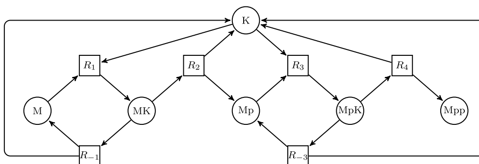
Fig. 5 Bipartite graph representation of the reactions M + K \rightleftharpoons MK \Rightarrow K + M_p \rightleftharpoons M_pK \Rightarrow K + M_{pp} . Arcs being all labeled with 1; this label is not shown
