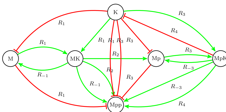
Fig. 8 Influence graph of Fig. 5, but with arcs ending in K and M_{pp} substituted, and then the only arc ending in K changed of sign. Resulting negative self-loops are, as usual, not shown, but note that the negative arcs from K to M_{pp} corresponds to the negative self-loops on K in the original graph. All positive circuits remaining can be ruled out by one of our corollaries as being a possible source of multistationarity
