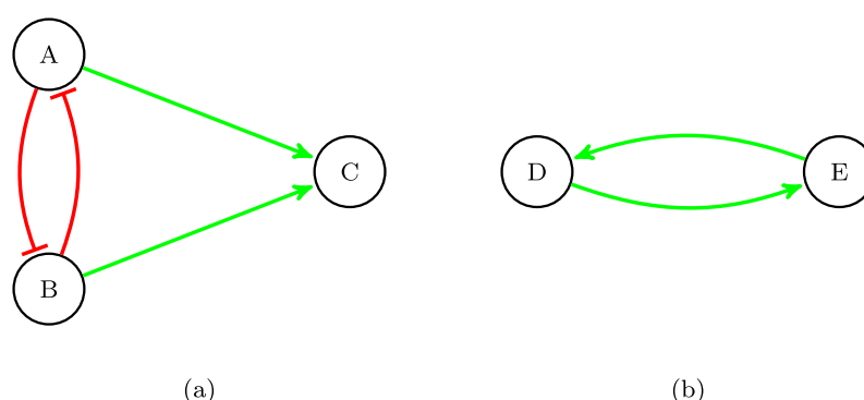
Fig. 1 (a): mutual inhibition resulting from A + B \Rightarrow C . (b): mutual activation resulting from D \Leftrightarrow E . For clarity, negative self-loops have not been represented
