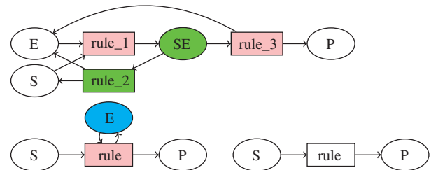
Fig. 1. Reaction graphs of the Michaelis–Menten enzymatic reaction, either complete with intermediary complex SE , or reduced with or without enzyme E . The first reduction can be achieved with the graphical operations explained in Section 2.2, for example by merging the reaction nodes rule\_1 and rule\_3 in pink into a reaction node rule and by deleting the green nodes SE and rule\_2 . The second reduction simply deletes the blue node E .
