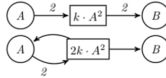
Figure 4. Two possible structures for Example 2. This illustrates the need for symbolic parameters in order to avoid confusion when inferring the structure. doi:10.1371/journal.pone.0014284.g004
