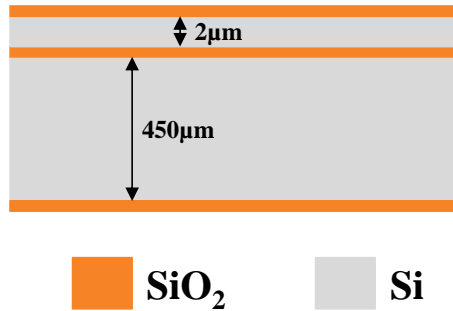
Figure 3-1 : Wafers SOI
