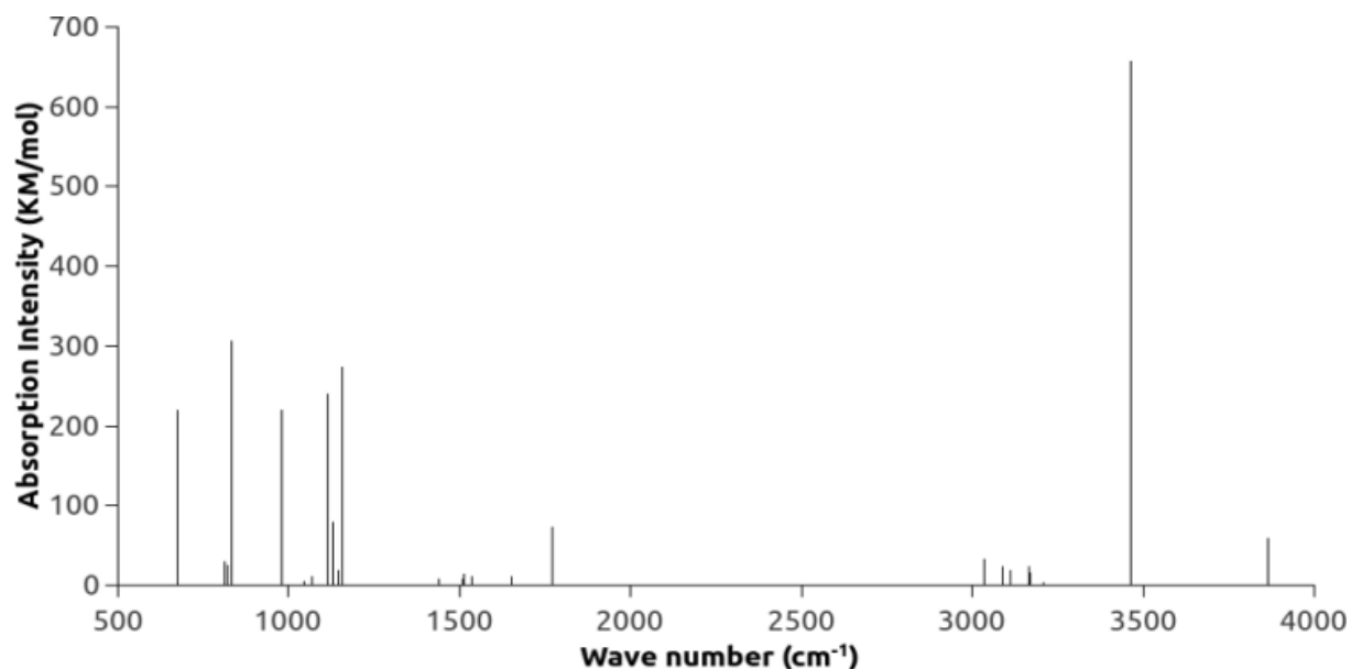
Figure V.6: QM computed IR spectra of functionalized styrene- \text{Na}^+\dots\text{H}_2\text{O} adduct (Fig. V.1)
