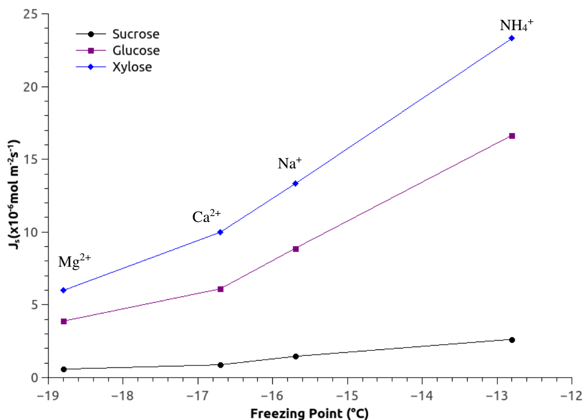
Figure V.18: Sugar fluxes in function of the freezing temperature of water entrapped in CMX membrane soaked in different electrolytes. Sugar fluxes measured in diffusion regime [Sugar] = 1 mol L -1 [electrolyte] = 1equiv. L -1 [10].
