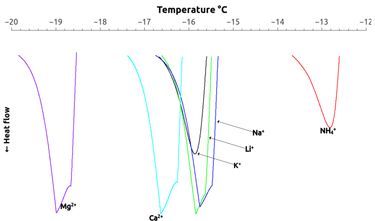
Figure V.17: DSC cooling peaks for CMX membrane equilibrated by different counter-ions.
