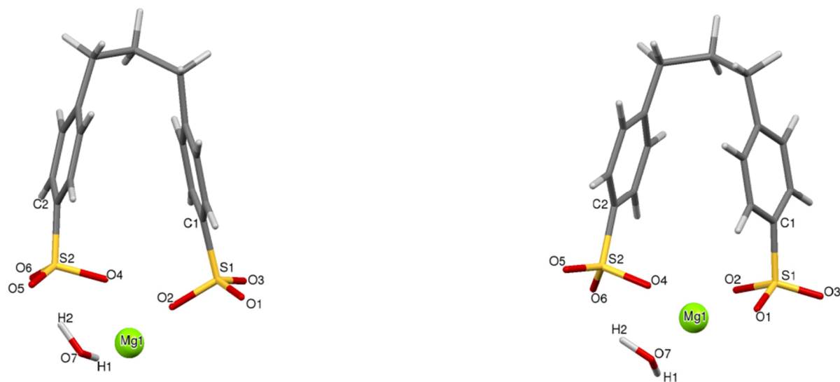
Figure V.5: Initial (left) and optimized (right) geometries of two functionalized styrene monomers equilibrated by Mg^{2+} with a water molecule in external position in the initial and optimized geometries.
