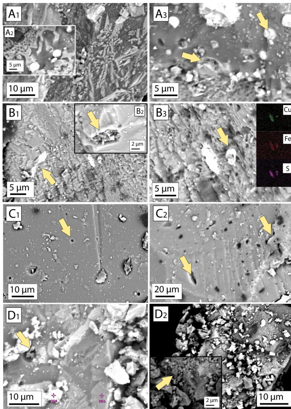
FIGURE 5.6 Scanning electron microscope images presenting weathering features of slags exposed to humic acid solution for 960 h.
